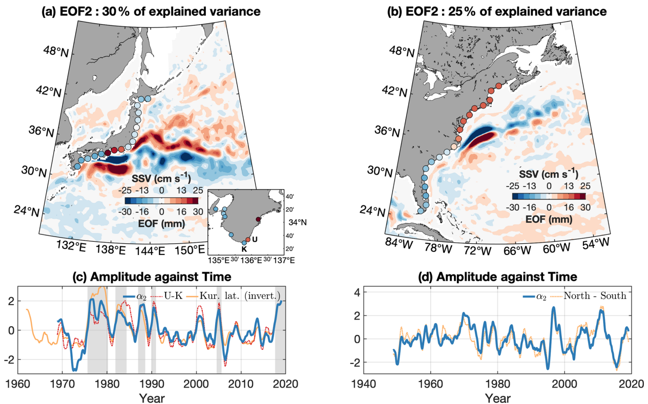
Figure 6. The second EOF ( \phi_2 ) of the gridded tide-gauge-based sea-level anomaly (circular markers) from the Pacific (a) and the Atlantic (b). The associated principal components \alpha_2 are shown as thick dark blue lines for the Pacific (c) and Atlantic (d). Also in (c), the Kuroshio southernmost latitude south of Tōkai is represented by the solid orange line (positive values indicate Kuroshio further to the south); the difference between sea level at Urugami and Kushimoto is represented by the dot-dashed red line, and grey shading represents periods of typical large meander (JMA, 2018). In (d), the dashed yellow line is the sea-level difference between the averages of northern and southern groupings of tide gauges, as in McCarthy et al. (2015). All time series in (c) and (d) are normalized. For each basin, colour shading in (a) and (b) is the sea surface velocity magnitude composite difference based on the principal component \alpha_2 (period of \alpha_2 > +2/3 minus period of \alpha_2 < -2/3 ). The arbitrary threshold of \pm 2/3 was used, but taking any number between 0 and 1 leads to similar patterns. The inset in (a) presents the regression coefficient obtained when the principal component is regressed on the original tide gauges, with a zoom-in on the Kii peninsula.
