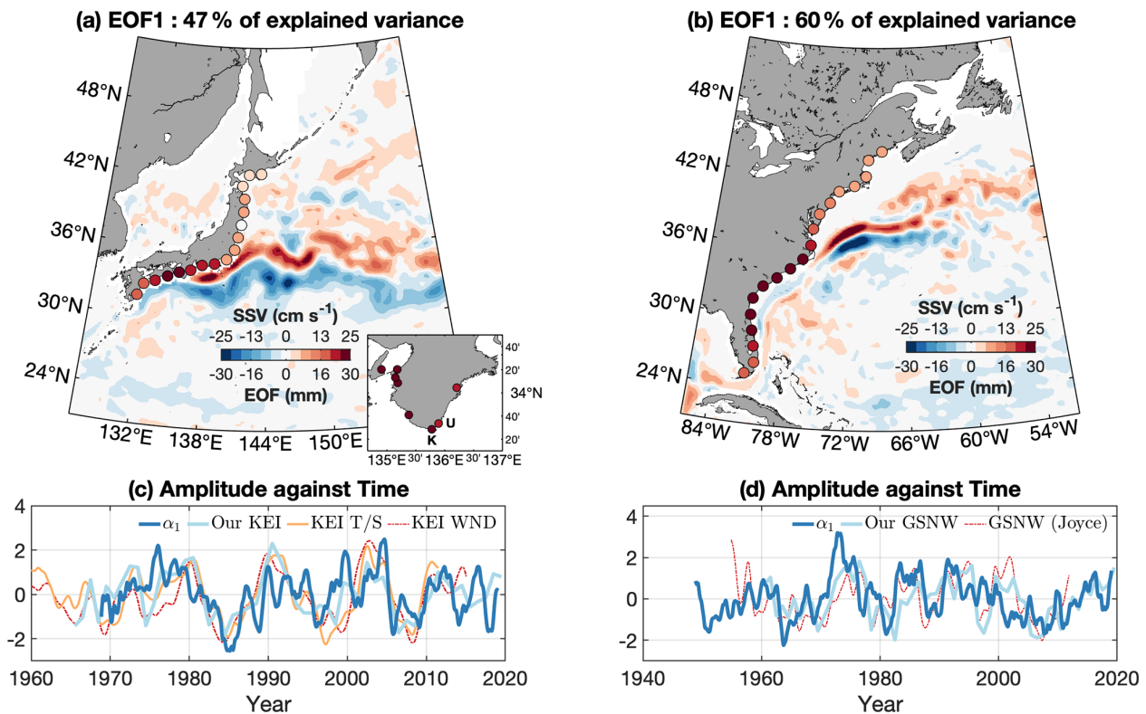
Figure 5. The leading EOF ( \phi_1 ) of the gridded tide-gauge-based sea-level anomaly (circular markers) from the Pacific (a) and the Atlantic (b). The associated principal components \alpha_1 are shown as thick dark blue lines for the Pacific (c) and Atlantic (d), together with indices of the WBC extension meridional location: this study (thick light blue line), Qiu et al. (2016) T / S -based (thin orange line) and wind-based (thin dot-dashed red line) KEIs, and Joyce et al. (2000) GSNW (thin red dot-dashed). All time series in (c) and (d) are normalized. For each basin, colour shading in (a) and (b) is the sea surface velocity magnitude composite difference based on the principal component \alpha_1 (period of \alpha_1 > +2/3 minus period of \alpha_1 < -2/3 ). The arbitrary threshold of \pm 2/3 was used, but taking any number between 0 and 1 leads to similar patterns. The inset in (a) presents the regression coefficient obtained when the principal component is regressed on the original tide gauges, with a zoom-in on the Kii peninsula.
