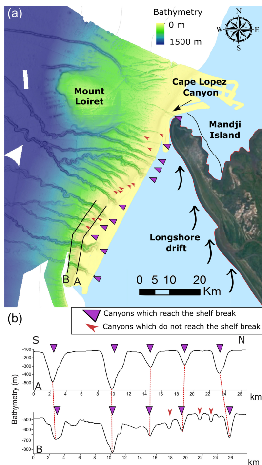
Figure 3. (a) Close-up view of the Gabon shelf and canyons ramp. Bathymetry is from the Optic Congo2005 and MOCOSSED2010 surveys; satellite view is from Google Earth. (b) Two bathymetric profiles across the canyons showing the two types of canyons which are present along the Gabonese slope.
