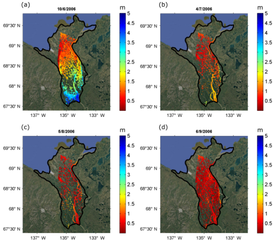
Figure 9. Water level maps in the Mackenzie Delta in 2006 (historic flood) obtained by combining inundated surfaces determined using MODIS images with altimetry-derived water levels (a) in June, (b) in July, (c) in August and (d) in September.
