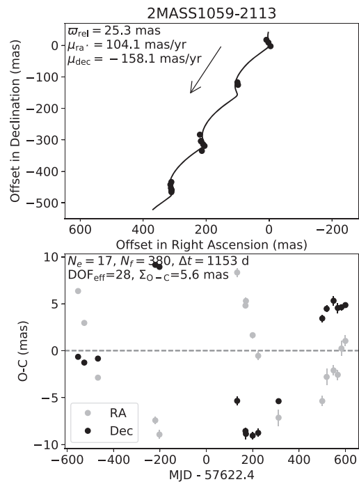
Figure 4. Results of fitting the six-parameter model (PPM+DCR) to 2M1059–21. The on-sky motion (top) and the epoch residuals (bottom) are shown. Significant excess signal is evident.
