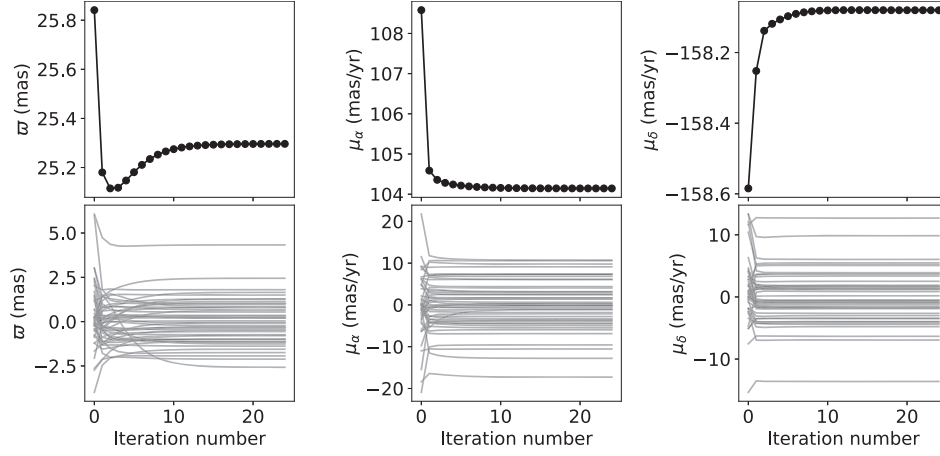
Figure 2. Effects of the iterative analysis for 2M1059–21. The evolution of the best-fitting parallax (left), proper motion in RA (middle), and Dec. (right) is shown as a function of iteration number for the target (top row) and the reference stars (bottom row).
