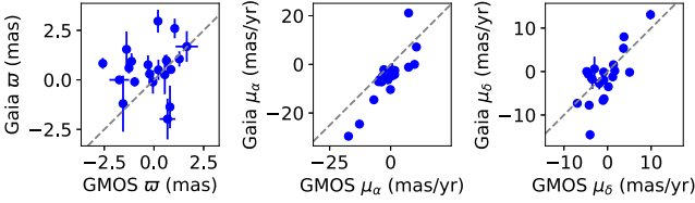
Figure 3. Comparison of parallaxes and proper motions between our determinations and GDR2 in the 2M1059–21 field. In this case, there are 21 reference stars that are both in GDR2 and are used in the final iteration. These are used to derive the corrections to absolute.
