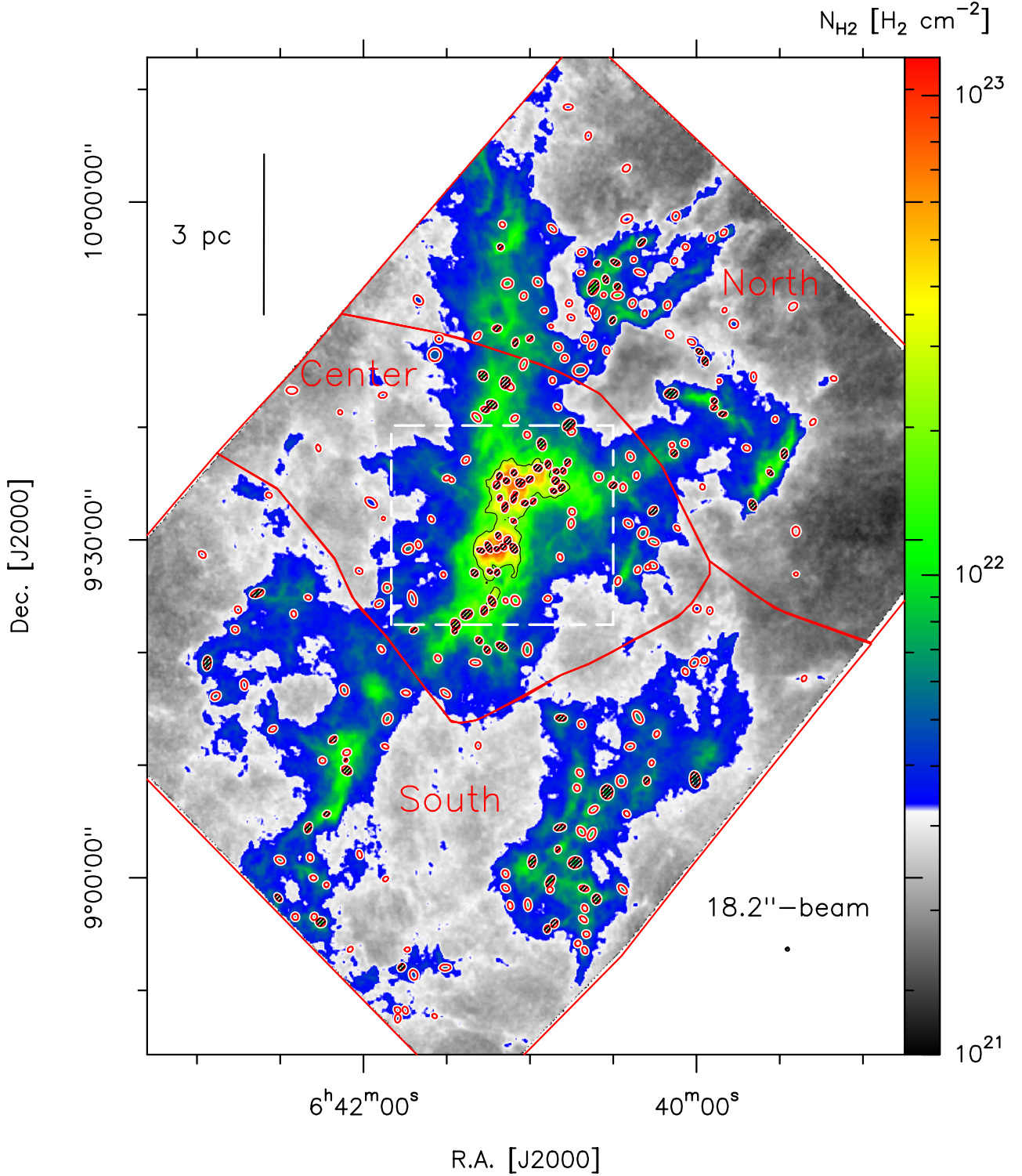
Fig. 2. NGC 2264 cloud traced by its Herschel column density. The clumps extracted by getsf are indicated by hatched ellipses for gravitationally bound clumps and open ellipses empty for unbound clumps. The contour at 2 \times 10^{22} \text{ cm}^{-2} highlights the brightest parts. The resolution of the map, 18.2'' , is shown in the lower right corner and a scale bar is given in the upper left corner. The outline and labels of the three subregions defined in Sect. 3.1 and used in the analysis are shown in red. The location of the zoom of Fig. 3 is shown with a white box.
