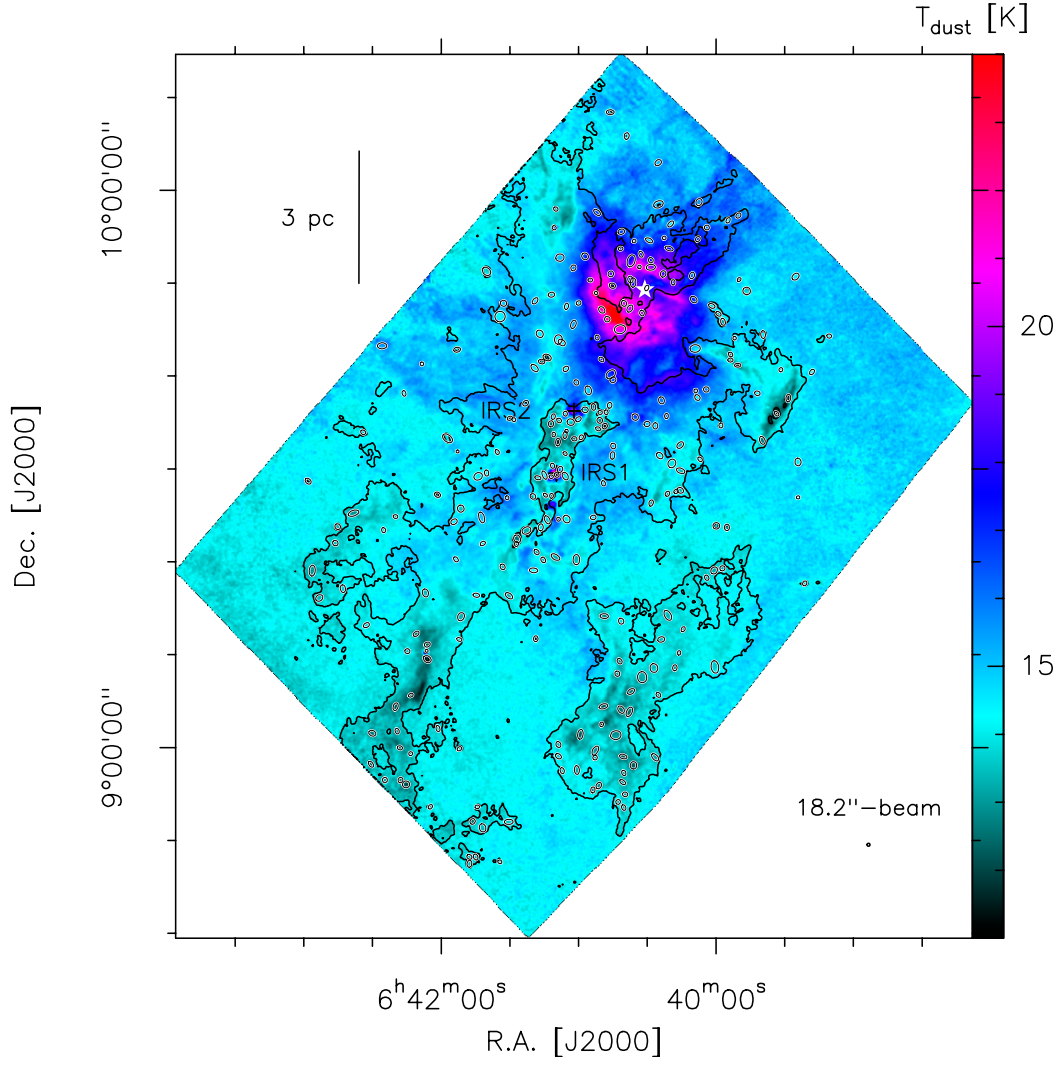
Fig. A.1. Herschel dust temperature image of the NGC 2264 cloud, with 3.4 \times 10^{21} \text{ H}_2 \text{ cm}^{-2} and 1.6 \times 10^{22} \text{ H}_2 \text{ cm}^{-2} contours taken from the column density image of Fig. 2. The resolution of the map, 18.2'', is shown in the lower right corner and a scale bar is given in the upper left corner. A white star locates the OB star cluster, which heats its surrounding cloud over several parsecs. The IRS1 and IRS2 protoclusters are also indicated.
