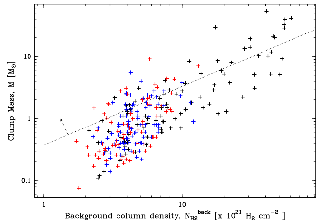
Fig. A.5. Correlation observed between the clump mass and its background column density. The color code highlighting the spatial location of the clumps is the same as in Fig. 7. The completeness curve in dotted line is calculated using a 90% completeness contrast of 1.1 and the M-N_{\text{H}_2}^{\text{peak}} relation (see Figs. A.2 and A.3): M = 0.34 (1.1 \times N_{\text{H}_2}^{\text{back}})^{0.95} .
