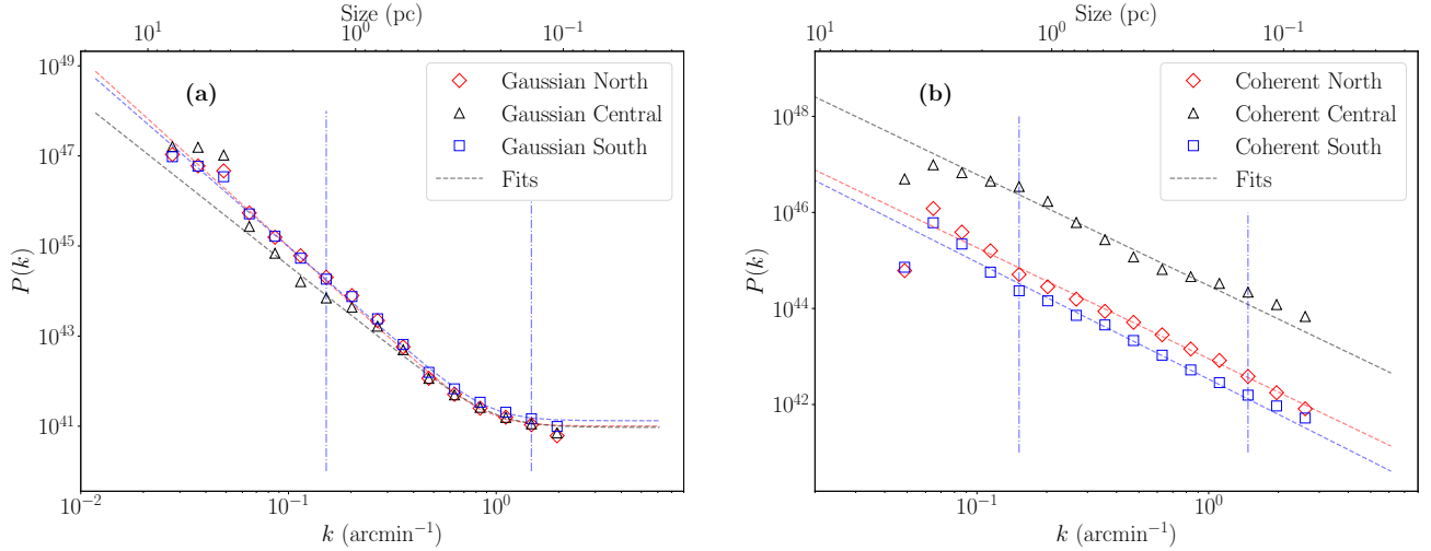
Fig. 6. Random Gaussian ( panel a ) and coherent ( panel b ) wavelet power spectra calculated by MnGseg for the three NGC 2264 subregions. The dotted black and red curve represents the fitted power law relations to the northern and central subregions. The coherent power spectrum of the central subregion stands out with \sim 100 times more power and bumps located at 1.4 and 0.1 pc (vertical blue dashed lines).
