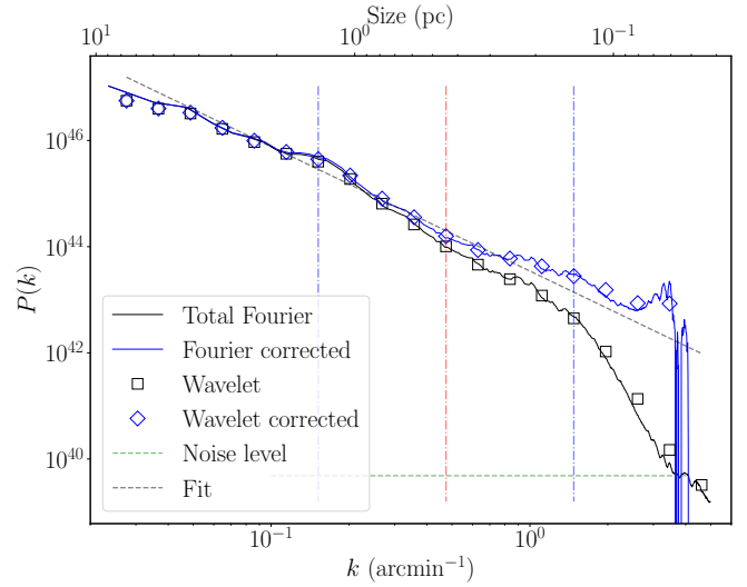
Fig. 4. Fourier (solid lines) and wavelet (symbols) power spectra of the NGC 2264 region. Before fitting a P(k) = A k^\gamma relation (dashed curve), the corrected power spectra are subtracted by the noise level (plateau at the end of the original power spectrum, dotted horizontal green line) and divided by the empirical SPIRE 250 \mu\text{m} beam. The power spectra present two bumps, located at 1.4 and 0.1 pc (dot-dashed vertical blue lines). The intermediate scale chosen to separate the three NGC 2264 subregions is indicated by a dot-dashed vertical red line.
