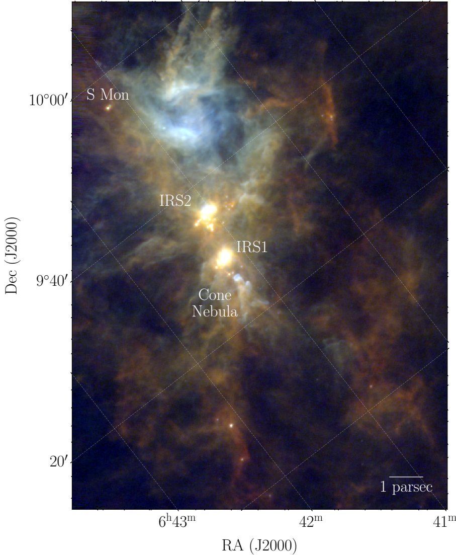
Fig. 1. Composite three-color Herschel image of NGC 2264: PACS 70 and 160 \mu\text{m} in blue and green; SPIRE 250 \mu\text{m} in red. The massive star S Mon, the central protoclusters NGC 2264 IRS1 and IRS2 and the Cone Nebula are labeled. The blue component traces heated regions while earlier stage star-forming sites, such as clumps and filaments, are traced by the red component. The image has been rotated from the RA–Dec grid.
