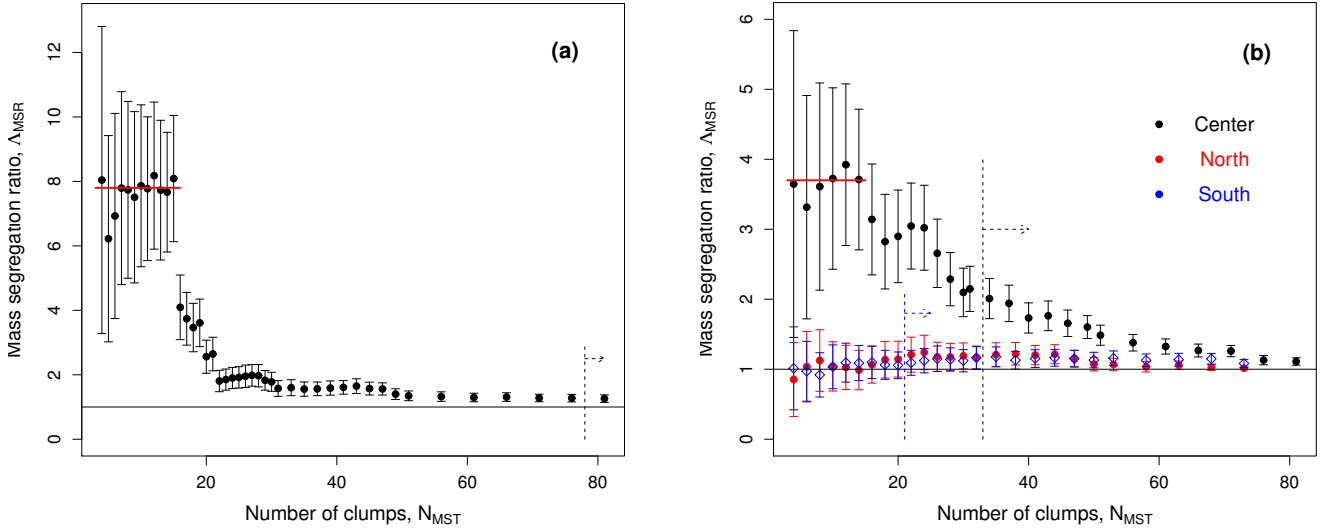
Fig. 11. Mass segregation ratio, \Delta_{\text{MSR}} , as a function of the numbers of clumps, N_{\text{MST}} , in the NGC 2264 cloud ( panel a ) and in its three subregions ( panel b ). Error bars represent the \pm 2\sigma uncertainties. Values above \Delta_{\text{MSR}} \approx 1 (black solid line) suggest mass segregation. Completeness levels are indicated with vertical dashed lines. Panel a : median segregation ratio for the 15 most massive clumps of NGC 2264, calculated over N_{\text{MST}} = 4 to 15, is \Delta_{\text{MSR}}^{\text{med}} = 7.8 (red segment). Panel b : the \Delta_{\text{MSR}} function of clumps in the central subregion (black symbols) is three to two times higher than that in the northern and southern subregions (in red and blue, respectively) over the range of N_{\text{MST}} = 4 –33.
