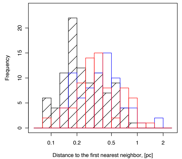
Fig. 9. Distribution of the distance to the first nearest neighbor for clumps in the central (black hatched histogram), northern (red histogram), and southern (blue histogram) subregions of NGC 2264. Clumps are 1.6 times more closely packed in the central subregion than in the two others.
