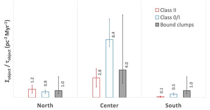
Fig. 14. Surface density per lifetime, \Sigma_{\text{object}}/\tau_{\text{object}} , of Class II YSOs, Class 0/I protostars, and clumps in the three NGC 2264 subregions. Statistical lifetimes of 2, 0.2, and 0.3 Myr were assumed for Class IIs, Class 0/Is, and clumps, respectively. Error bars take into account statistical uncertainties, contamination level of 30% for Class IIs, an incompleteness level of 25% for the Class 0/I population in the central subregion, and a factor of two of uncertainty for the clumps. While the star formation activity of the northern subregion appears to be constant, it displays a burst in the central subregion and shows a tentative increase in the southern subregion.
