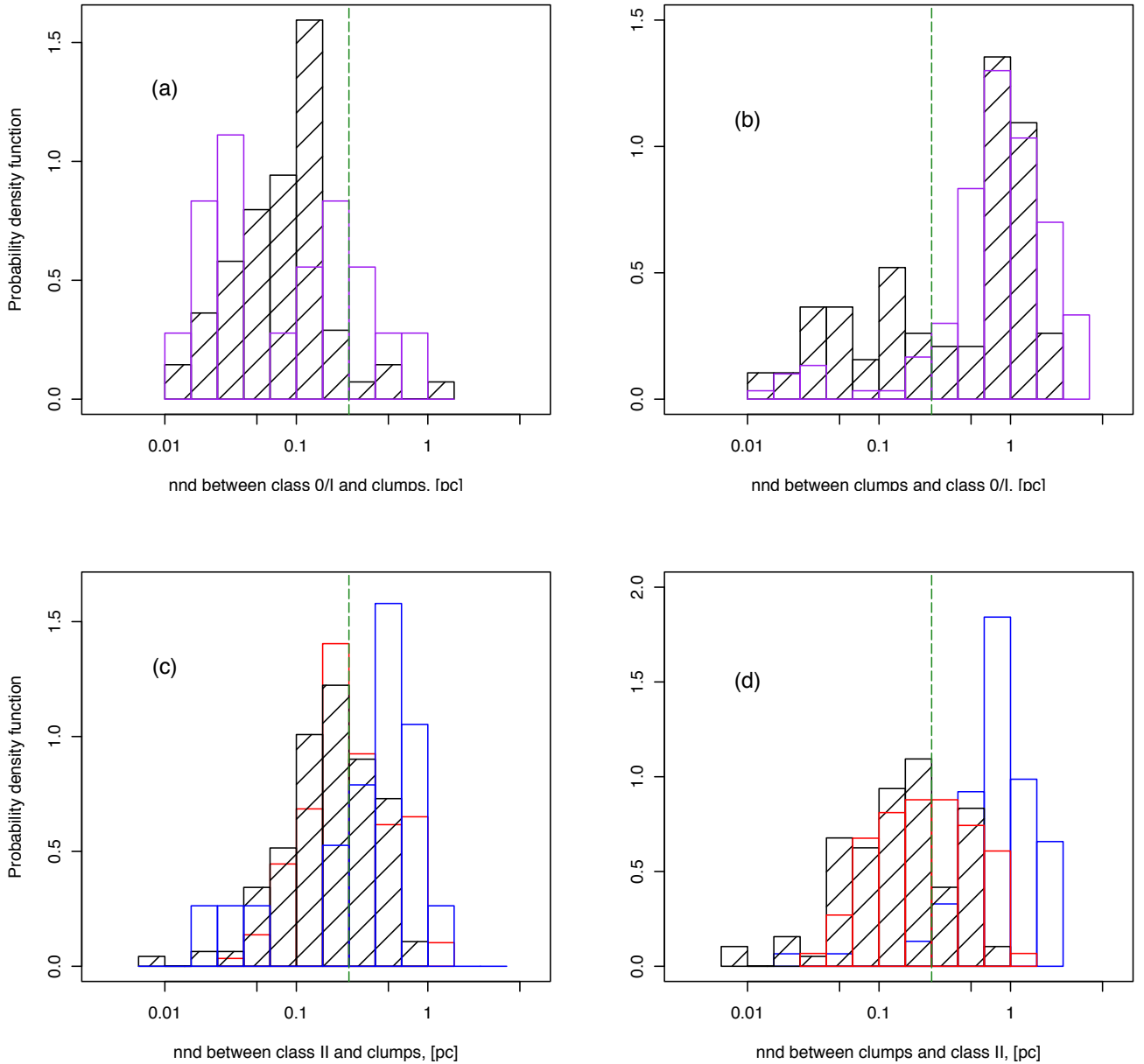
Fig. 13. Distribution of the distance to the first nearest neighbor, nnd , from YSOs to clumps (panels a and c ) and from clumps to YSOs (panels b and d ). The YSOs are Class 0/I in the upper panels ( a and b ), Class II in the lower panels ( c and d ). Distributions are presented for the central subregion (hatched black histograms) and for the northern and southern subregions, combined in the upper panel (purple histogram) and separated in the lower panel (red and blue histograms, respectively). Distributions are normalized to facilitate the comparison involving small populations of YSOs (Class 0/I from northern and southern subregions in panel a , Class II from southern subregions in panel c ). The dashed vertical red line indicates the median outer radius of clumps, calculated as twice the median FWHM: R_{\text{out}}^{\text{med}} = 2 \text{FWHM}^{\text{med}} = 0.25 pc.
