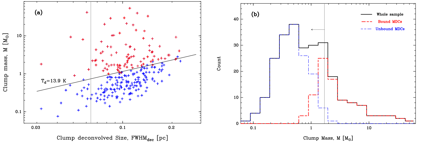
Fig. 8. Mass vs. size diagram ( panel a ) and mass distribution ( panel b ) for the 256 clumps detected in the NGC 2264 cloud. Gravitationally bound and unbound clumps, with \alpha_{\text{BE}} < 2 and \alpha_{\text{BE}} \geq 2 , respectively are located with red (resp. blue) markers ( panel a ) and sum up in a red (resp. blue) histogram ( panel b ). Panel a : the critical Bonnor-Ebert sphere model ( \alpha_{\text{BE}} = 2 ) at the median clump temperature, T_{\text{dust}} = 13.9 \text{ K} , is plotted as a black solid line. The physical size of the beam at a distance of 723 pc is plotted as a vertical dotted line. Panel b : the global 90% completeness level is indicated with a dotted line.
