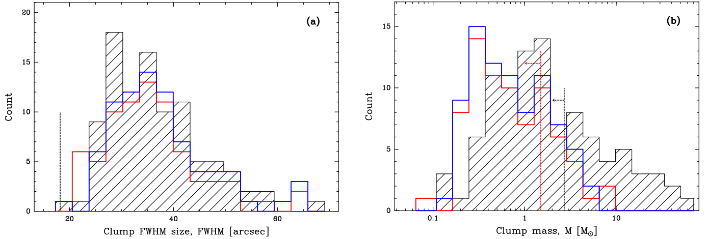
Fig. 7. Distribution of clump size ( panel a ) and clump mass ( panel b ) for the three subregions of NGC 2264: central (hatched black histograms), northern (red histograms), and southern (blue histograms) subregions. The central subregion has an excess of high-mass clumps compared the northern and southern subregions. The angular resolution of our observations, 18.2'' , is given in panel a . The completeness levels, \sim 2.7 M_{\odot} in the central subregion and \sim 1.5 M_{\odot} in the northern and southern subregions, are indicated in panel b with dotted lines.
