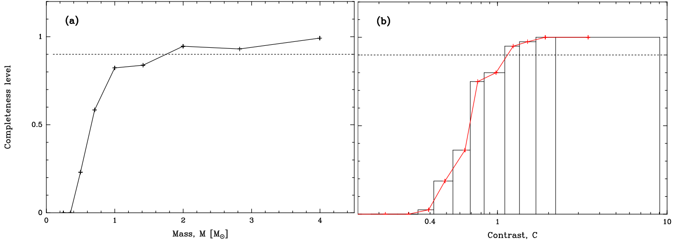
Fig. A.2. Completeness level of the clumps extraction as a function of the clump mass ( panel a ) and of the contrast of the clump column density over its local background ( panel b ). The 90% completeness level is indicated with a dashed horizontal line. Panel a : the clump sample is 90% complete above 1.7 M_{\odot} . Panel b : the histogram has been constructed with a constant number of 80 synthetic sources in the 11 first bins, plus a bin containing the remaining 290 sources that have all been detected. The red curve connects the median contrast value in each bin. Of the clumps, 90% are detected for a contrast larger than 1.1.
