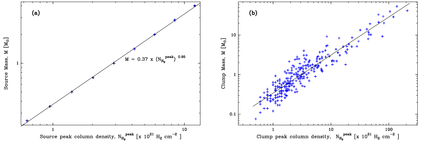
Fig. A.3. Mass as a function of peak column density for synthetic sources ( panel a ) and for observed clumps ( panel b ). A simple regression gives the relation M = \beta (N_{\text{H}_2}^{\text{peak}})^{0.95} with \beta = 0.37 in panel a over a [0.6 - 12 \times 10^{21} \text{ cm}^{-2}] range, \beta = 0.34 in panel b over a [0.5 - 200 \times 10^{21} \text{ cm}^{-2}] . The similarity in the fitted parameters confirms that the synthetic sources correctly represent the observed clumps.
