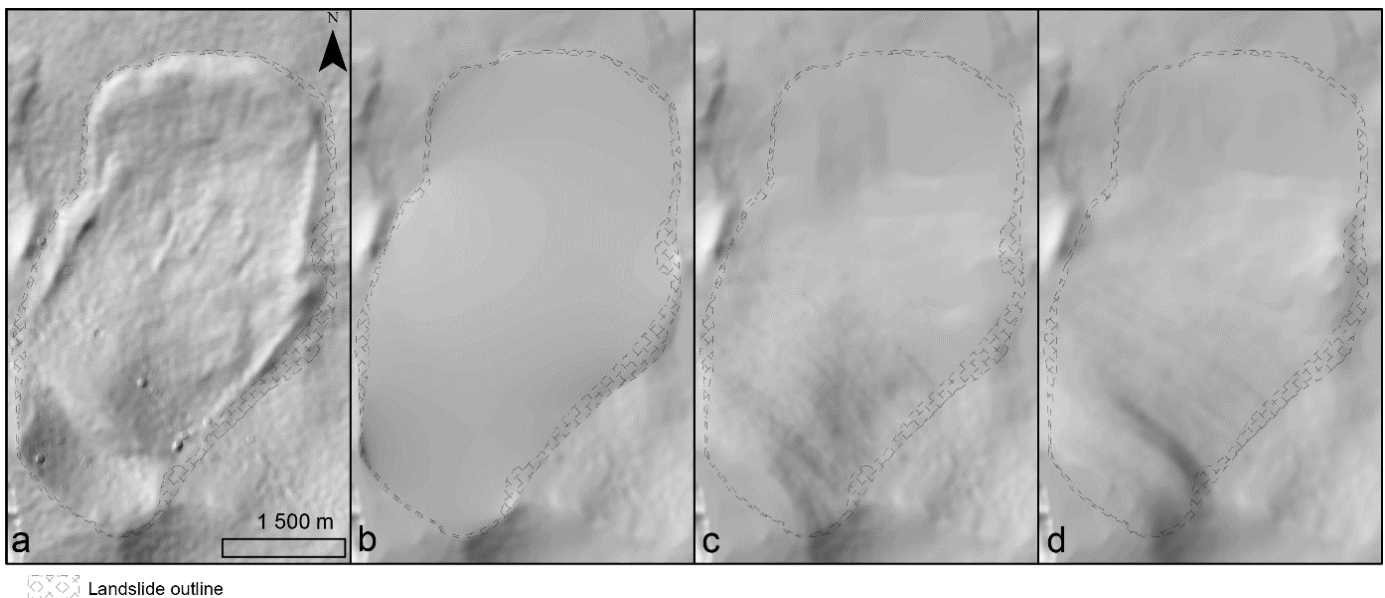
Figure 8 – Hillshaded relief view of (a) the original CaSSIS DEM with Baetis Chaos landslide. Hillshaded relief view of the topographic reconstructions using (b) the semi-automatic method, (c) the morphology-based method and (d) tilted method.
