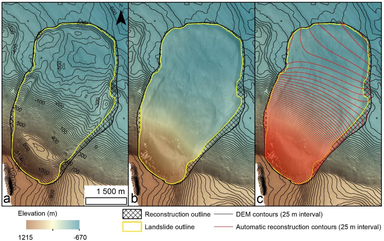
Figure 4 – Key steps in the semi-automatic reconstruction method (a) Colour-coded original CaSSIS DEM of Baetis Chaos landslide with contour lines at 25-m interval overlain by the semi-transparent PAN orthoimage. (b) Same as panel a without the contour lines inside the landslide reconstruction outline. (c) Automatically reconstructed contour lines in red produced from a DEM interpolated using the Natural Neighbour interpolation algorithm. Credit: ESA/Roscosmos/Unibe/INAF
