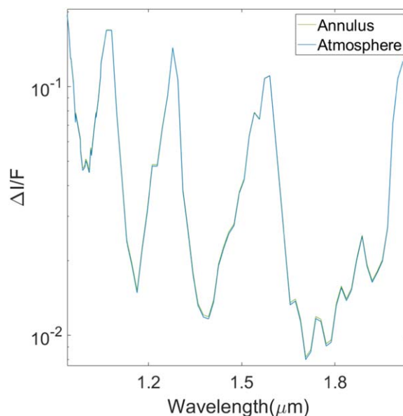
Figure C. Zoom-in of the modeled atmospheric spectra and the modeled annulus spectra from Figure 3. The difference between the two spectra is less than the line width at certain wavelengths.
