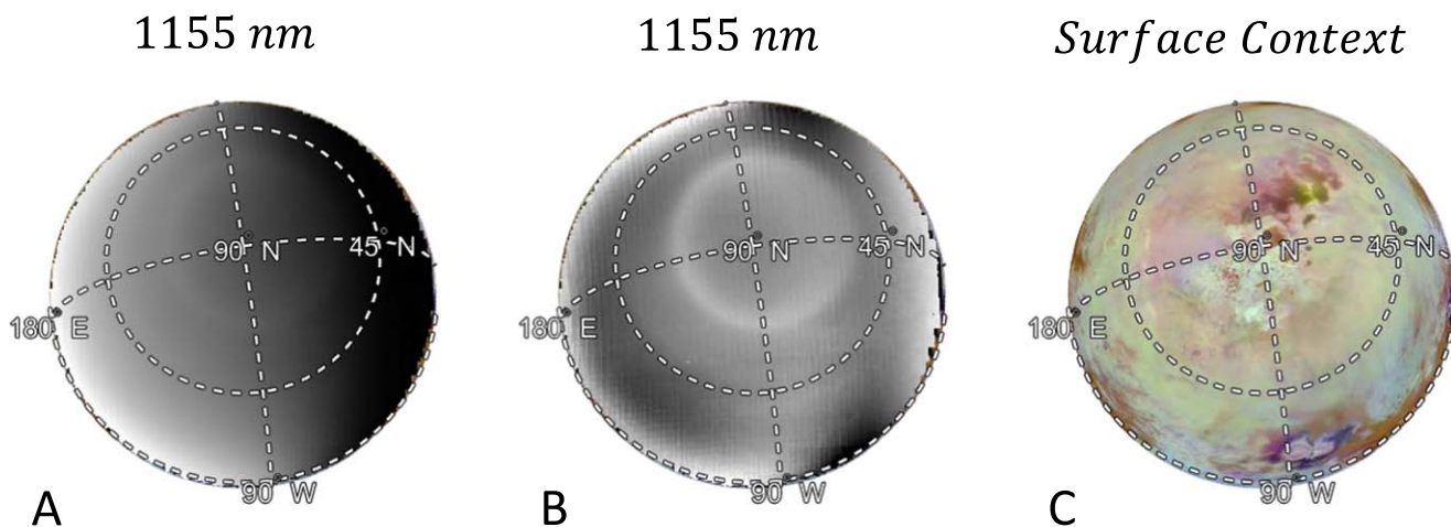
Figure 1. Orthographic mosaics of T096, 2013-12-01, L_S = 51.2 . (A) 1155 nm mosaic. (B) 1155 nm mosaic with manifold correction. (C) Context using VIMS-ISS map (Seignovert et al. 2019).
