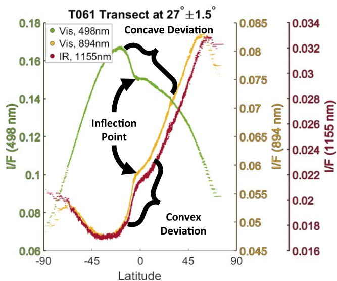
Figure 3. Transect of pixels from mosaic of T61 flyby [2009-08-25] (see Figure 2). The deviation in each of the three curves is attributed to the EQA. The inflection point of each deviation is attributed to the center of the annulus, and the Gaussian tail on either side of the inflection point is the uncertainty in locating the annulus. The north–south asymmetry appears as the smooth parabolic curve between the hemispheres. The EQA adds a sharp deviation in the curve, without which the north–south asymmetry would appear as a gradient between the hemispheres, rather than the asymmetry we see.
