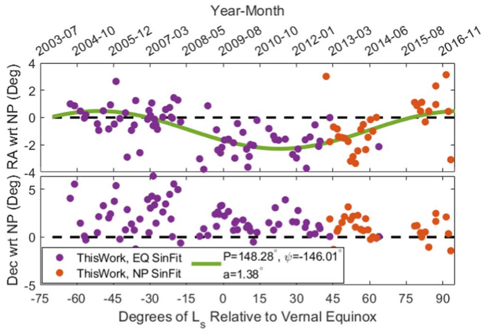
Figure 12. Top: the R.A. offset of the normal vector of the annuli from the solid-body rotation axis in an inertial reference frame (ICRF). The R.A. of Titan’s solid-body rotation axis is R. A. = 39°48 (Stiles et al. 2008). The green sinusoid through the flyby has a goodness-of-fit metric of R^2 = 0.411 . Bottom: the decl. offset of the normal vector of the annuli from the solid-body rotation axis in an inertial reference frame (ICRF). The decl. of Titan’s solid-body rotation axis is R.A. = 83°43 (Stiles et al. 2008).
