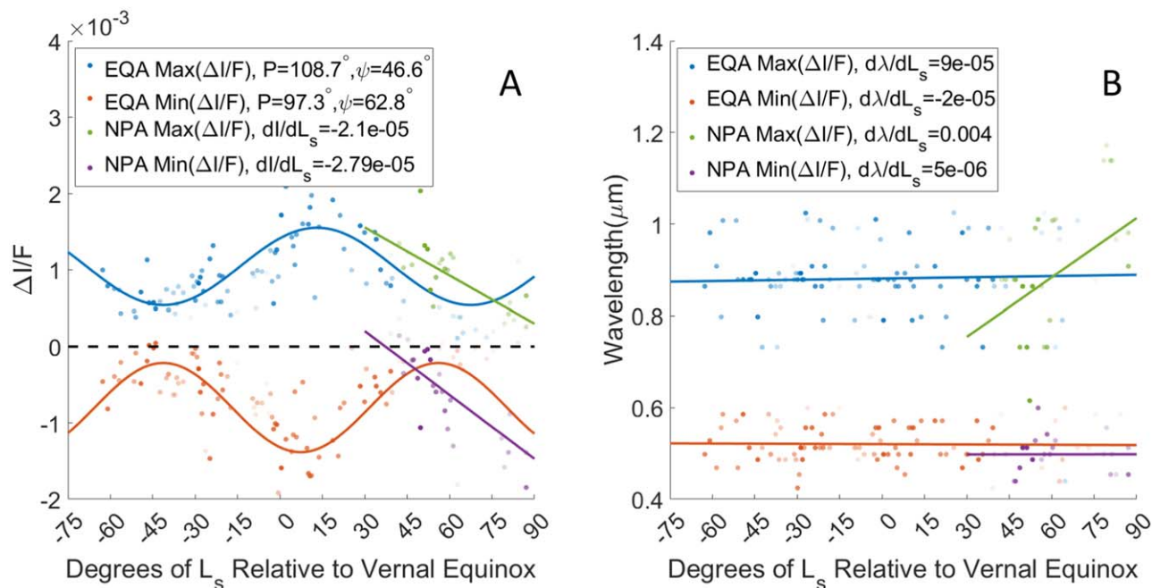
Figure 10. (A) Blue: maximum value of \Delta I/F of the EQA differential spectrum. Orange: minimum value of \Delta I/F of the EQA differential spectrum. Green: maximum value of \Delta I/F of the NPA differential spectrum. Purple: minimum value of \Delta I/F of the NPA differential spectrum. (B) Blue: the wavelength of the maximum \Delta I/F of the EQA differential spectrum. Orange: the wavelength of the minimum \Delta I/F of the EQA differential spectrum. Green: the wavelength of the maximum \Delta I/F of the NPA differential spectrum. Purple: the wavelength of the minimum \Delta I/F of the NPA differential spectrum. The opacity of the data points correlates to the relative weight of the data. Data are weighted according to the number of transect detections. For details on the curves, see Table 2.
