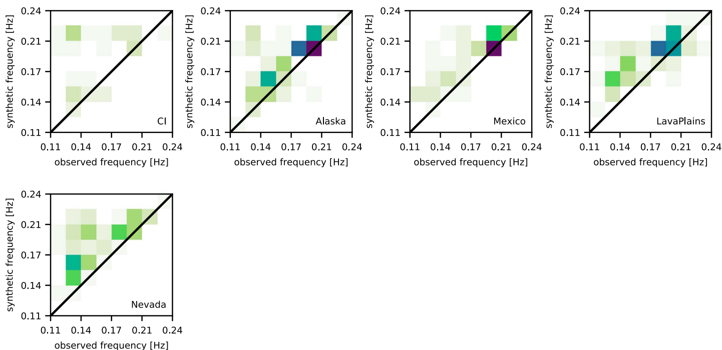
Figure A2. Comparison of the matching observed strongest source frequencies with model R for arrays (a) CI, (b) Alaska, (c) Mexico, (d) LavaPlains, and (e) Nevada.
