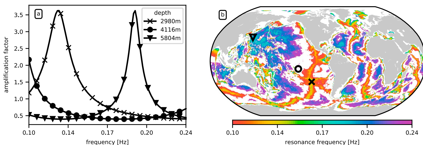
Figure 3. (a) P wave amplitude amplification due to water column resonance as a function of frequency for three different ocean depths, computed for slowness 0.05 s/km in a simple two-layer model. (b) Map of the corresponding resonance frequencies in the frequency band of interest (0.10–0.24 Hz) and at slowness 0.05 s/km. The position of the three examples from Figure 3a are indicated with the corresponding symbols in the map.
