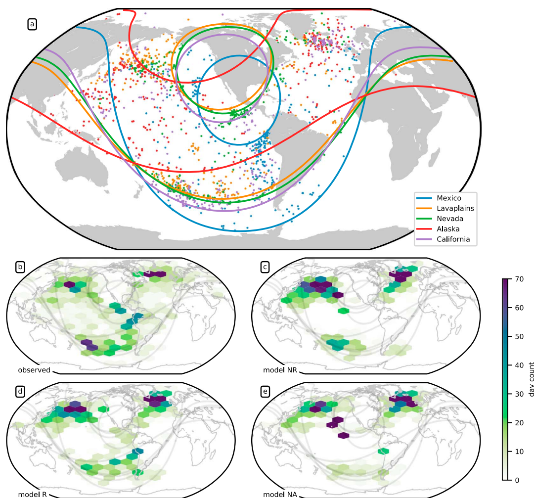
Figure 5. Geographical distribution of the strongest sources. (a) The observed strongest source positions colored by the array that observed them. We have added a small jitter ( 2^\circ ) to the positions to make clusters better visible. Observations that cluster at the observation limits of an array have to be interpreted with caution. (b–e) The source density is shown for observations, model NR, model R, and model NA. The observation limits of the arrays are indicated with lines from Figures 5a and 5e. The observed and modeled source density is biased by the number of arrays that can observe a particular region (see Figure 1b). Model R fits best with the observations. Model NR and NA are missing the coastal reflections along the South American Pacific coast. Model NA has the worst overall fit with the observations.
