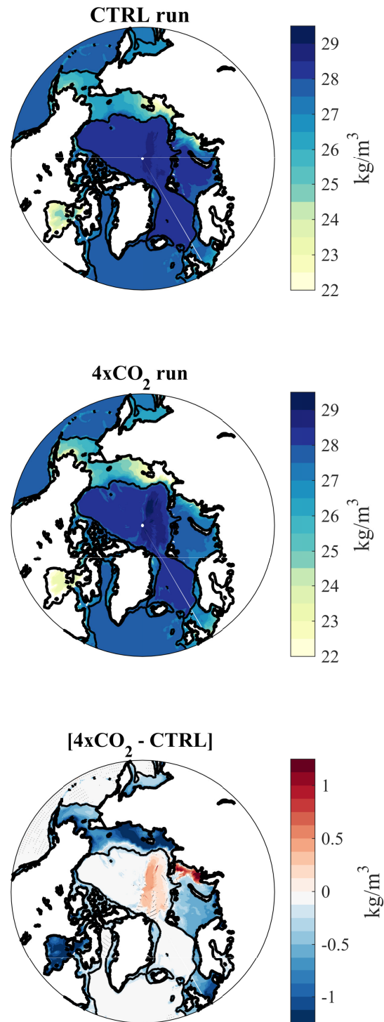
Fig. 9: 10-year average of the bottom density (in kg/m^3 ) for the CTRL and the 4 \times CO_2 runs and the difference between the two runs. For the bottom row, black hatching indicates areas where the difference between the two runs is not significant. Bottom density corresponds to the density of the last ocean model vertical level at each grid point, and is computed relative to the surface. The black contour shows the 500m isobath.
