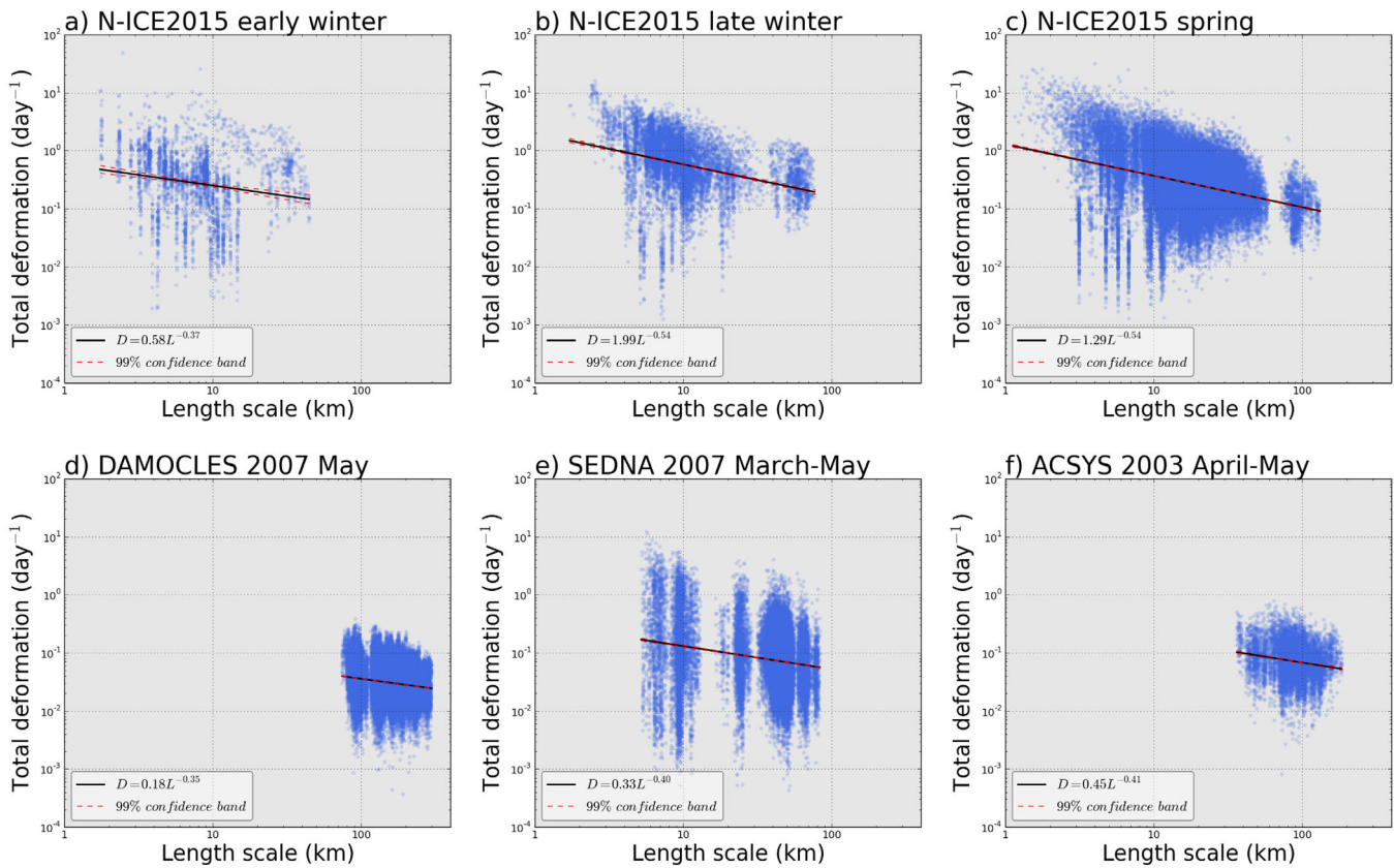
Figure 5. Scatter plots of length scale and total deformation for N-ICE2015 (a—winter before the storm, b—after the storm, and c—spring), d—DAMOCLES 2007, e—SEDNA 2007, and f—ACSYS 2003. The exponential fit to the data is depicted with the black line that follows the power law. Note the logarithmic scale on both axis. Refer to Figure 1 for locations of the array deployments.
