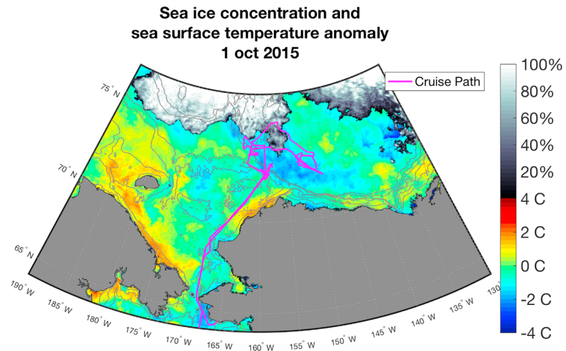
Figure 10. Sea surface temperature anomaly (colors, derived from SST data available at https://mur.jpl.nasa.gov ) and ice cover (grayscale, derived from AMSR2, data available at https://seaice.uni-bremen.de/start/data-archive ) in the western Arctic at the start of Sikuliaq research cruise (magenta is track line).
