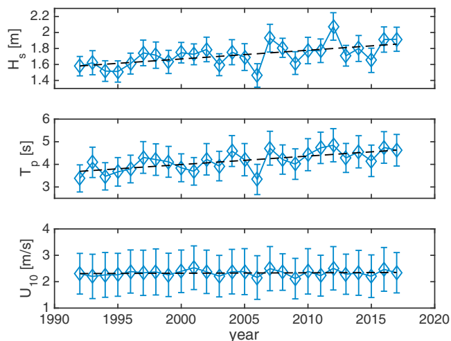
Figure 1. Trends in the wave heights, wave periods, and wind speeds over the Beaufort and Chukchi seas in autumn. Updated from (Thomson et al., 2016) with values for 2015, 2016, and 2017. Values are the shape and scale parameter of Weibull distributions fit to hindcast waves across the months of September, October, and November.
