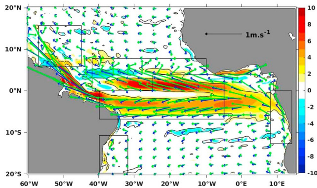
Figure 8. Surface current seasonal mean ( \bar{u} , blue arrows), sum of the seasonal mean and interannual anomalies related to the meridional mode ( \bar{u} + 10u' , green arrows), and amplitude of the interannual anomalies related to the meridional mode (cm/s, shading). Interannual anomalies related to the meridional mode correspond to regression coefficients of interannual anomalies onto the meridional mode time function shown in Figure 2c. The multiplicative coefficient 10 is chosen arbitrarily to highlight currents anomalies. This somewhat distorts the direction of these current vectors. The black contours represent the 90% significance threshold and boxes are as in Figure 3a.
