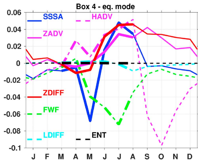
Figure 14. Time series of SSS anomalies (blue line), horizontal advection (magenta dashed line), vertical advection (magenta line), diffusion (red line), freshwater flux (green dashed line), lateral diffusion (light blue dashed line), and entrainment (black dashed line) in the south equatorial box ( 30^{\circ}\text{W} – 10^{\circ}\text{E} , 4^{\circ}\text{S} – 1^{\circ}\text{N} ) during a positive equatorial mode. All the time series are obtained by regressing the box-averaged interannual anomalies for each calendar month onto the summer equatorial mode time series shown in Figure 2f. The period from April to August corresponds to the development and the mature phase of the mode (heavy lines). SSS = sea surface salinity; SSSA = sea surface salinity anomaly.
