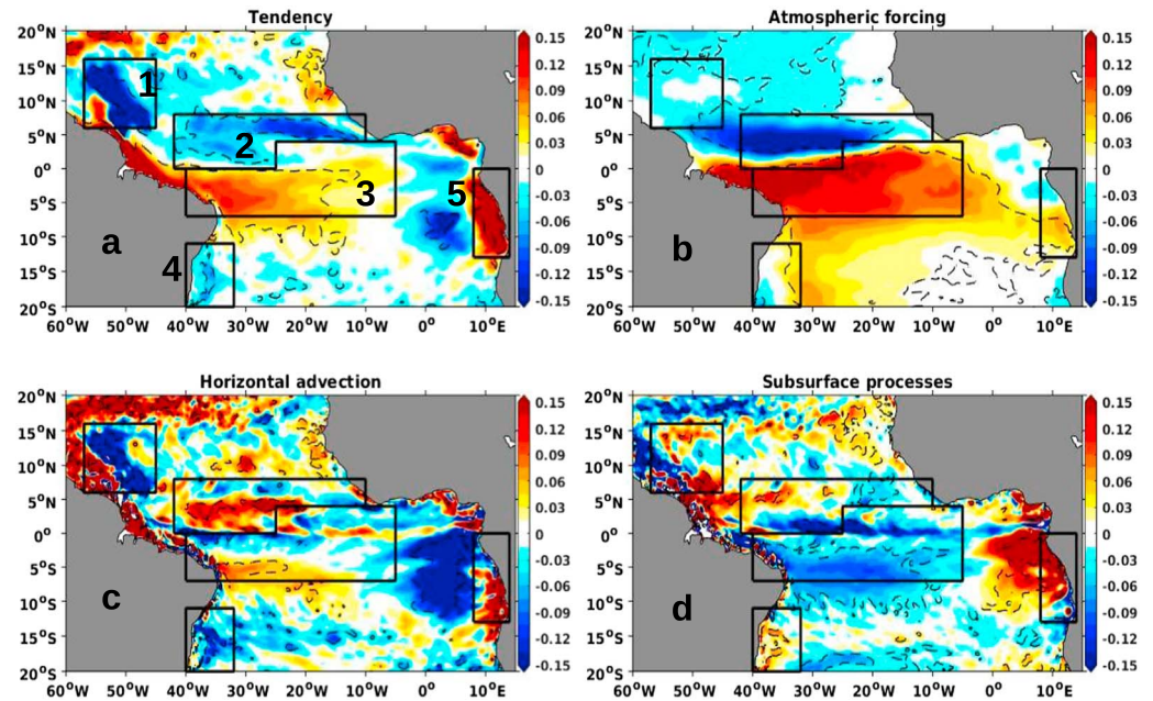
Figure 6. Winter to spring mixed-layer salinity budget (psu) for the meridional mode: (a) tendency term, (b) atmospheric forcing, (c) horizontal advection, and (d) subsurface processes. Figures 6a–6d represent regression coefficients of salinity budget term anomalies onto the meridional mode time function shown in Figure 2c. The dashed black contours and regions 1 to 5 are as in Figures 3a and 3b.
