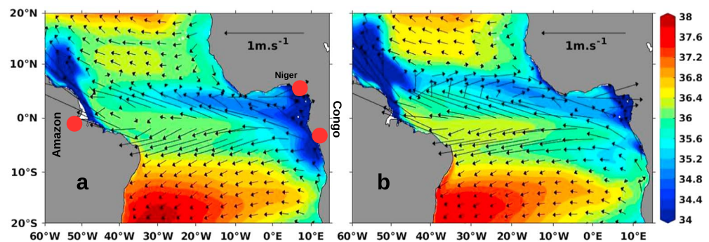
Figure 1. Boreal (a) spring and (b) summer SSS (shadings) and surface current (arrows) from model. The positions of the three major rivers (the Amazon, the Congo, and the Niger) are indicated as red circles in Figure 1a. SSS = sea surface salinity.
