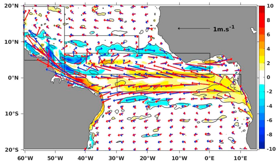
Figure 12. Surface current seasonal mean ( \bar{u} , blue arrows), sum of the seasonal mean and interannual anomalies related to the equatorial mode ( \bar{u} + 10u' , red arrows), and amplitude of the interannual anomalies related to the equatorial mode anomalies (cm/s, shading). Interannual anomalies related to the equatorial mode correspond to regression coefficients of interannual anomalies onto the equatorial mode time function shown in Figure 2f. The multiplicative coefficient 10 is chosen arbitrarily to highlight currents anomalies. This somewhat distorts the direction of these current vectors. The black contours represent the 90% significance threshold, and boxes are as in Figure 3a.
