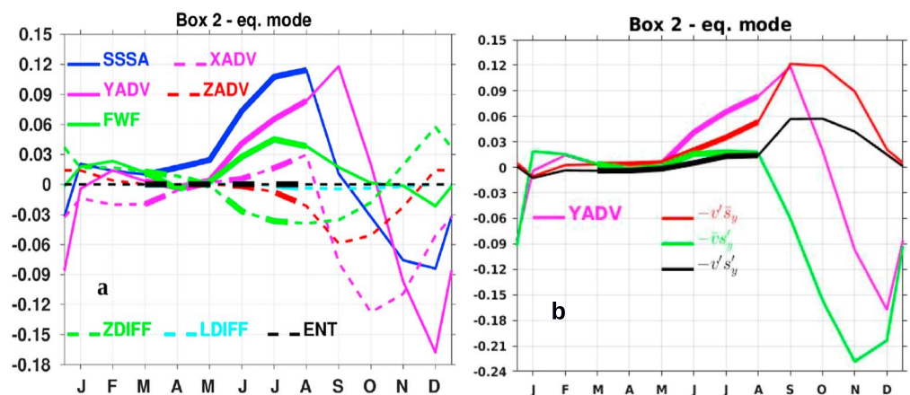
Figure 13. (a) Time series of SSS anomalies related to a positive equatorial mode (blue line); zonal (magenta dashed line), meridional (magenta line), and vertical (red dashed line) advection; freshwater flux (green line); vertical diffusion (green dashed line); lateral diffusion (light blue dashed line); and entrainment (black dashed line). And (b) the different terms of the meridional advection (magenta line) decomposition following equation (4), with term II (red line), term III (green line), and term IV (black line) in box 2 (47–23°W, 7–12°N). All the time series are obtained by regressing the box-averaged interannual anomalies for each calendar month onto the summer equatorial mode time series shown in Figure 2f. The period from April to August corresponds to the development and the mature phase of the mode (heavy lines). SSS = sea surface salinity; SSSA = sea surface salinity anomaly.
