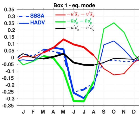
Figure 11. As Figure 7a but related to a positive equatorial mode in the western box 1 (60–47°W, 5–20°N), where only negative anomalies are averaged. All the time series are obtained by regressing the box-averaged interannual anomalies for each calendar month onto the summer equatorial mode time series shown in Figure 2f. The period from April to August corresponds to the development and the mature phase of the mode (heavy lines). SSSA = sea surface salinity anomaly; HADV = horizontal advection.
