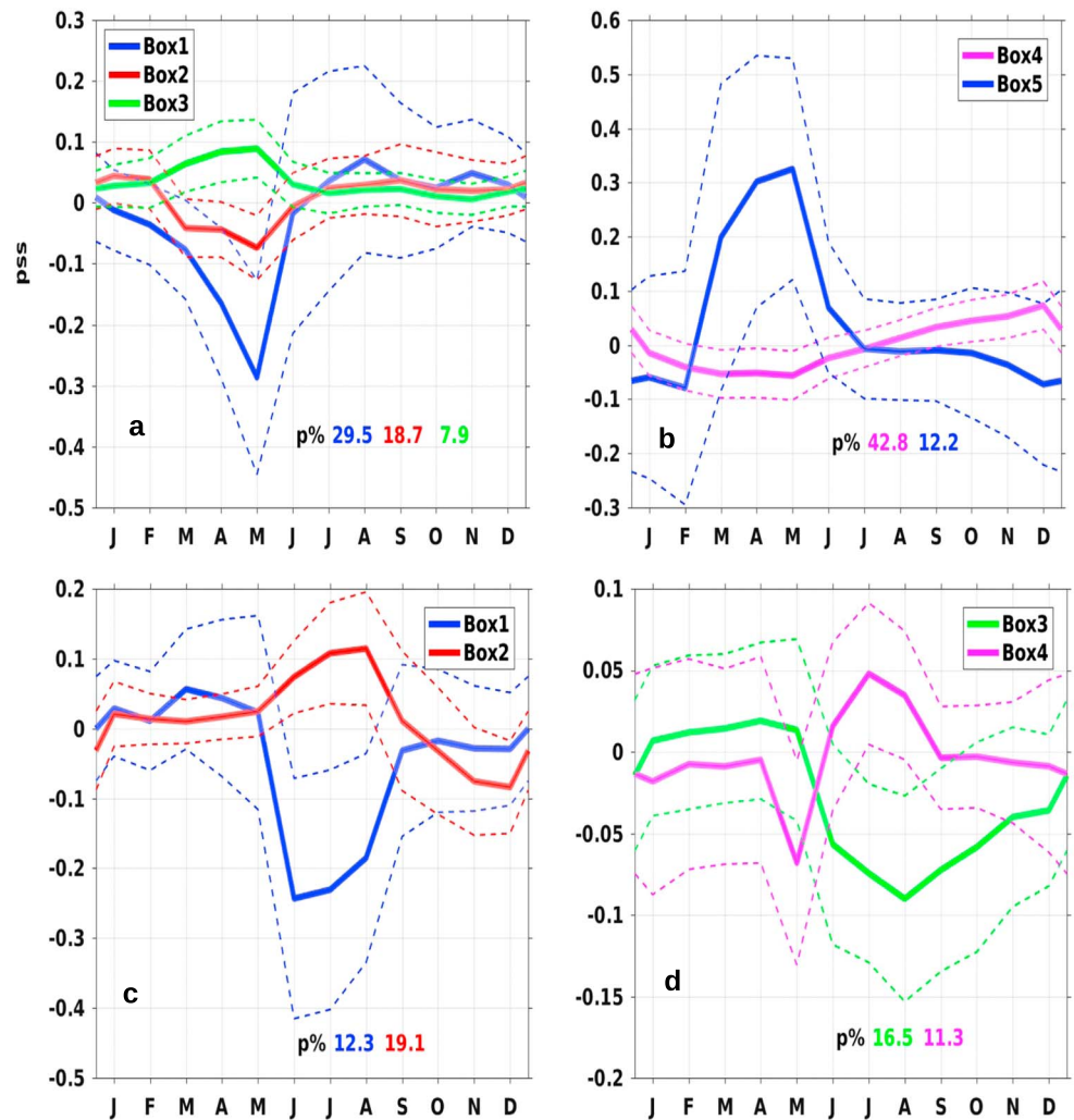
Figure 5. Time series of model SSS anomalies in boxes 1 to 5 (see Figure. 3) related to the (a, b) meridional and (c, d) equatorial modes, obtained by regressing the box-averaged interannual SSS anomalies for each calendar month onto the spring meridional mode or summer equatorial mode time series shown in Figures 2c and 2f. In Figure 5c, only negative anomalies are averaged in box 1. The dashed lines represent the uncertainty range at 90% significance threshold. The explained variance ( p in percentage) of SSS anomalies in meridional mode season (spring; a, b) or equatorial mode season (summer; c, d) by their preseason SSS anomalies winter and spring, respectively). SSS = sea surface salinity.
