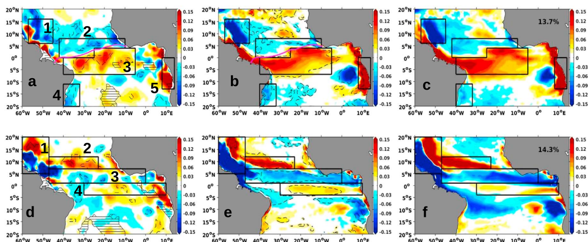
Figure 3. SSS signature of the positive phase of the (a–c) meridional and (d–f) equatorial modes from (a, d) in situ observations and (b, c, e, f) model. Figures 3a, 3b, 3d, and 3e represent regression coefficients of SSS anomalies onto the meridional and equatorial modes' time function, respectively (Figures 2c and 2f, black lines), and Figures 3c and 3f represent the dominant pattern mode of the EOF analysis performed on SSS anomalies in spring and summer, respectively. The front between positive/negative SST anomalies in Figure 2a is superposed on Figures 3a and 3b (magenta line). Regions 1 to 5 delimited by heavy black lines are discussed in the main text. The (a, d) hatched zones denote regions where the available data density is less than 50%. The dashed black contours represent the 90% significance threshold. SSS = sea surface salinity; EOF = empirical orthogonal function; SST = sea surface temperature.
