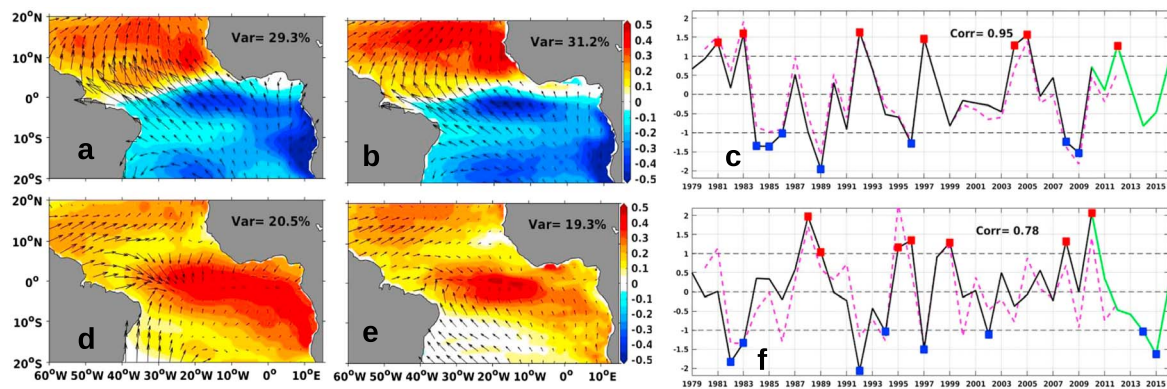
Figure 2. First combined EOF analysis maps performed on SST-wind anomalies in boreal (a, b) spring and (d, e) summer from ERA-Interim reanalysis (a, d; black lines in the time series), model (b, e; dashed magenta lines in the time series), and (c, f) their respective normalized time series for the 1979–2016 period. The green lines in the time series correspond to the SMOS period. Red and blue dots in the time series denote values in excess of \pm 1 standard deviation. EOF = empirical orthogonal function; SST = sea surface temperature; ERA = European Center for Medium Range Weather Forecasts (ECMWF) Reanalysis; SMOS = Soil Moisture–Ocean Salinity.
