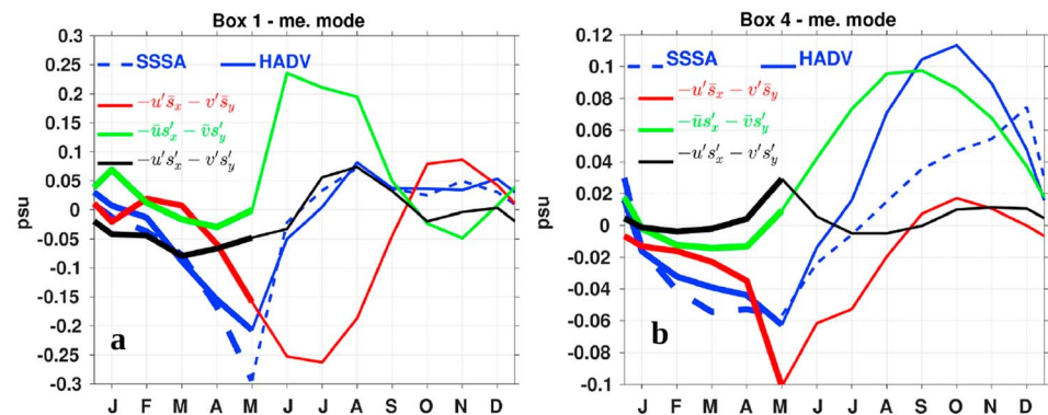
Figure 7. Time series of model SSS anomalies related to the meridional mode (blue dashed line), integrated horizontal advection anomalies (blue line) and their decomposition following equation (4) into term II (red line), term III (green line), and term IV (black line) in (a) box 1 (45–57°W, 6–16°N) and (b) box 4 (40–32°W, 11–20°S). All the time series are obtained by regressing the box-averaged interannual anomalies for each calendar month onto the spring meridional mode time series shown in Figure 2c. The January to May period corresponds to the development and the mature phase of the mode (heavy lines). SSS = sea surface salinity; SSSA = sea surface salinity anomaly; HADV = horizontal advection.
