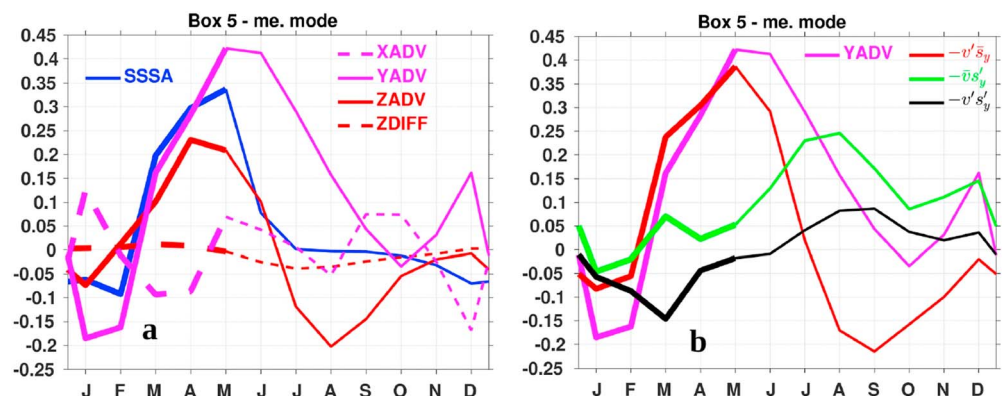
Figure 9. (a) Time series of SSS anomalies related to a positive meridional mode (blue line), zonal (magenta dashed line), meridional (magenta line) and vertical (red line) advection, and vertical diffusion (red dashed line); and (b) the different terms of the meridional advection (magenta line) decomposition following equation (4), into term II (red line), term III (green line), and term IV (black line) in box 5 (8–14°E, 13–0°S). All the time series are obtained by regressing the box-averaged interannual anomalies for each calendar month onto the spring meridional mode time series shown in Figure 2c. The period from January to May corresponds to the development and the mature phase of the mode (heavy lines). SSS = sea surface salinity; SSSA = sea surface salinity anomaly.
