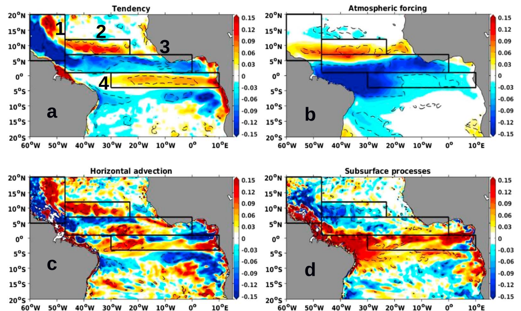
Figure 10. Spring to summer mixed-layer salinity budget (pss) for the equatorial mode: (a) tendency term, (b) atmospheric forcing, (c) horizontal advection, and (d) subsurface processes. Figures 10a–10d represent regression coefficients of salinity budget term anomalies onto the equatorial mode time function shown in Figure 2f. The dashed black contours and regions 1 to 4 are as in Figures 3d and 3e.
