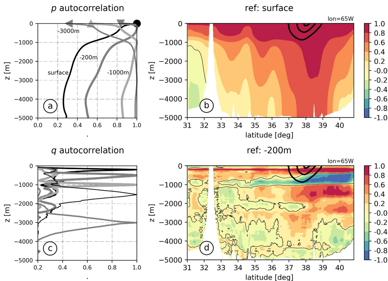
Figure 3. Autocorrelation vertical profiles of (a, b) pressure and (c, d) PV. (left) Horizontal average for several test levels: (a) surface, -200 , -1,000 , and -3,000 m (see labels) and (c) -200 , -500 , -1,000 , -1,500 , and -3,000 m (in the order of curves reaching autocorrelation = 1). (right) Vertical section at -65 W overlaid with the current velocity time mean (thick line, interval: 0.2 m/s) of (b) pressure autocorrelation with the surface reference and (d) PV autocorrelation with the -200 m reference. In Figure 3a, symbols mark the value of autocorrelation at the surface level.
