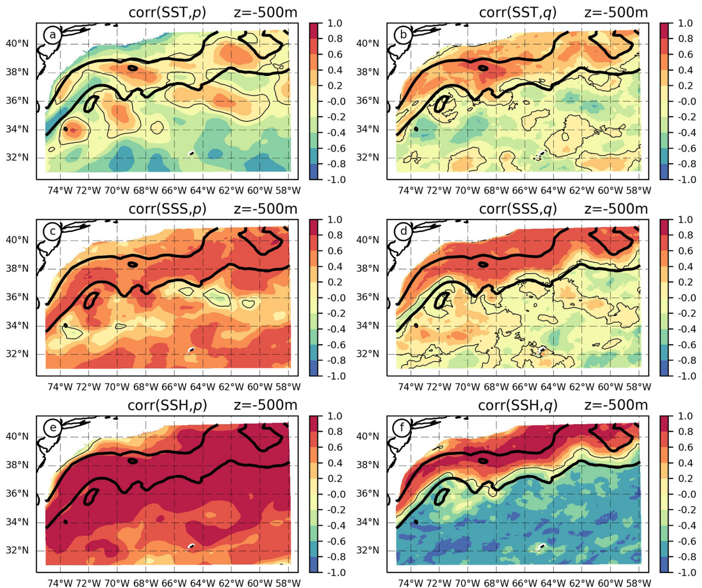
Figure 5. Horizontal sections at -500\text{ m} of the correlation coefficient of (left) pressure and (right) PV with (a, b) SST, (c, d) SSS, and (e, f) SSH, overlaid with the line 0.2\text{ m/s} of the surface current time mean.
