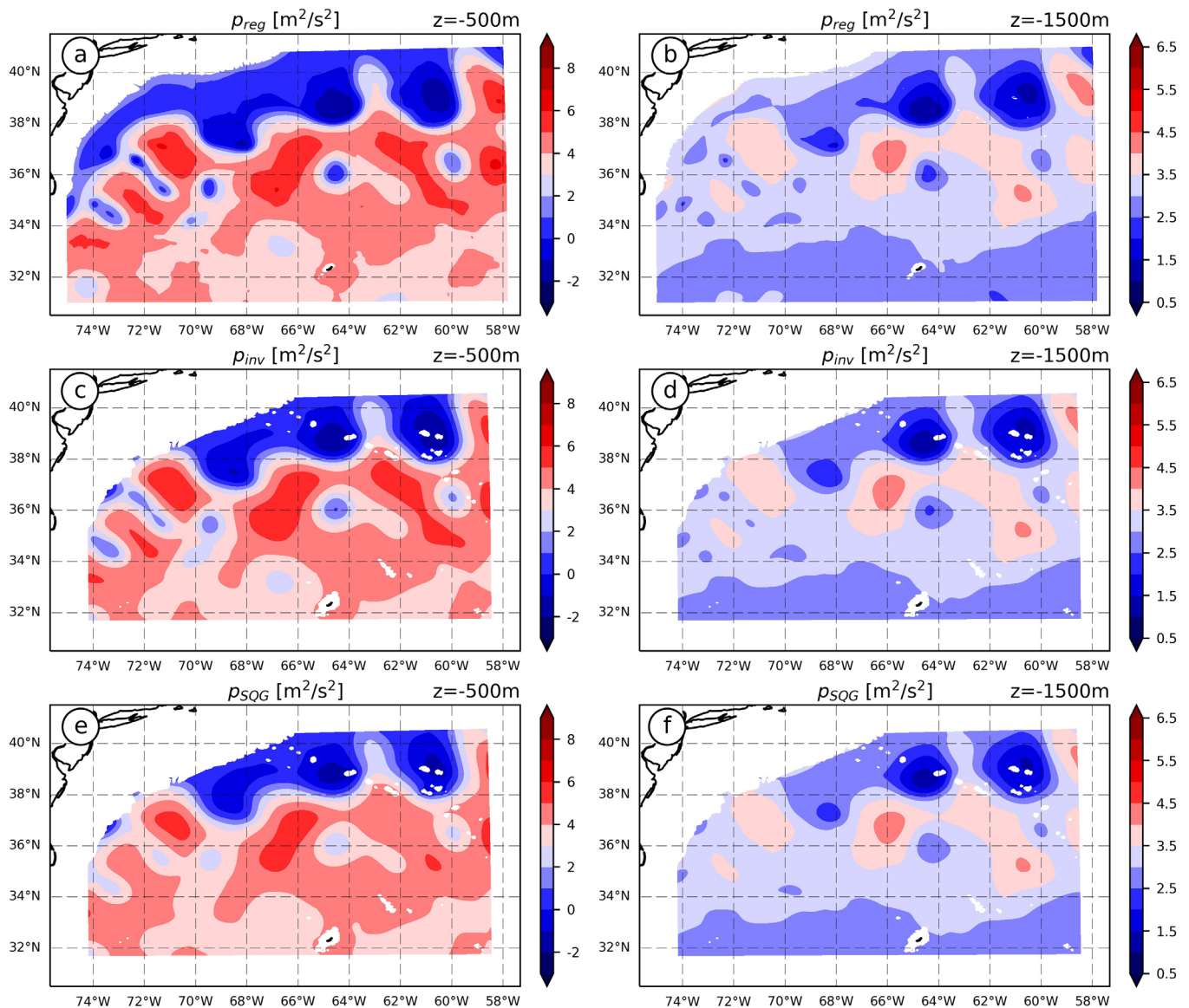
Figure 6. Horizontal sections at (left) -500 m and (right) -1,500 m of pressure reconstructions (a, b) p_{reg} , (c, d) p_{inv} and (e, f) p_{SQG} . Units: m^2/s^2 .
