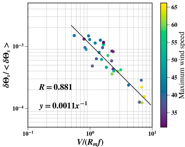
Figure 12. Observed sea surface temperature anomalies scaled by \langle \delta \theta_s \rangle = u_m N^{3/2} / (g \alpha f^{1/2}) versus tropical cyclone-Rossby number Ro = V / (fR_m) . Color indicates maximum wind speed. Solid line is the fit \delta \theta_s / \langle \delta \theta_s \rangle = 1.1 \times 10^{-3} Ro^{-1} .
