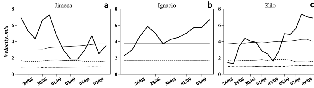
Figure 11. The along-track evolution of (thick solid lines) tropical cyclone translation velocity and internal waves phase velocity for three first modes (thin solid, dashed, and dash-dotted lines correspondingly) for tropical cyclones (a) Jimena, (b) Ignacio, and (c) Kilo.
