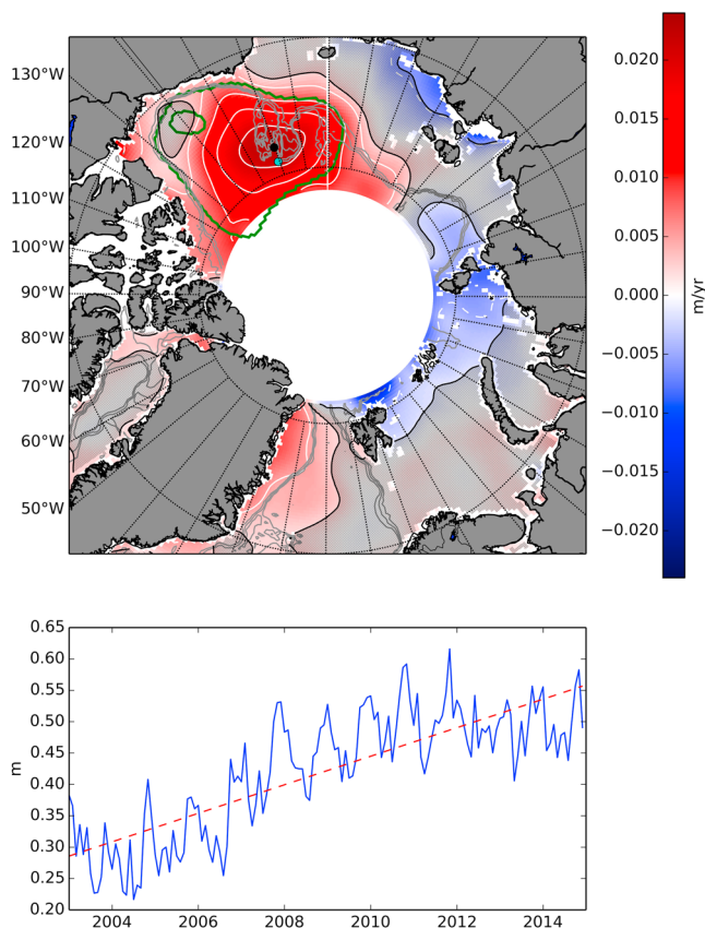
Figure 7. Map showing the linear trend (m/year) of the dynamic ocean topography time series at each location from 2003–2014. Time series of the dynamic ocean topography where the maximum trend occurs (black dot, over the Northwind Ridge) is shown below. The maximum trend found by Giles et al. (2012) is shown by a cyan dot. White contours indicate 0.005 m/year intervals, and areas which are not significant at the 95% level are hatched. The minimum and maximum gyre extent (in August 2004 and March 2013, respectively) are shown in green.
