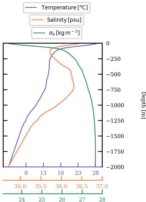
Figure 2. Background (blue) temperature, (red) salinity and (green) potential density. (Colour online)
