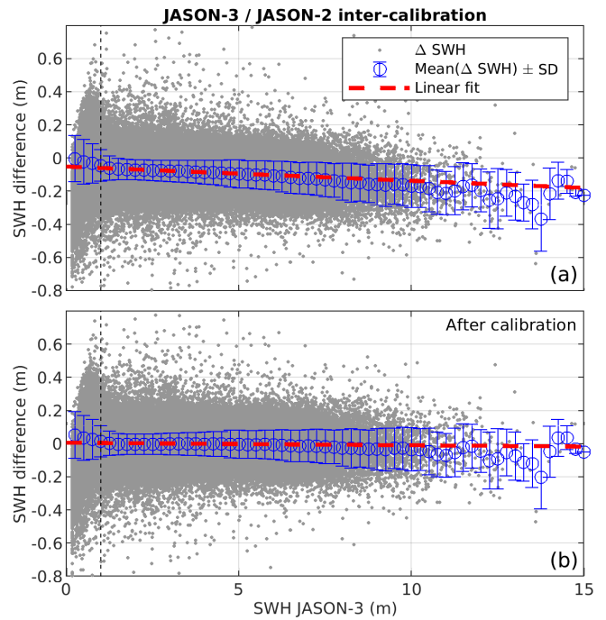
Figure 6. Residual of JASON-3 SWH – JASON-2 SWH as a function of JASON-3 SWH before (top) and after (bottom) calibration. The dashed red line is a linear fit through the data.
