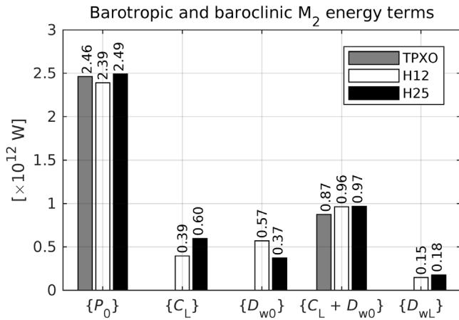
Fig. 5. Globally- and depth-integrated tidal-mean M 2 barotropic and baroclinic energy terms from Eqs. (2)–(4) for TPX08-atlas and the H12 and H25 simulations (. indicates area-integrated quantities). {P 0 } is computed for all seafloor depths, while the other terms are computed for seafloor depths deeper than 250 m.
