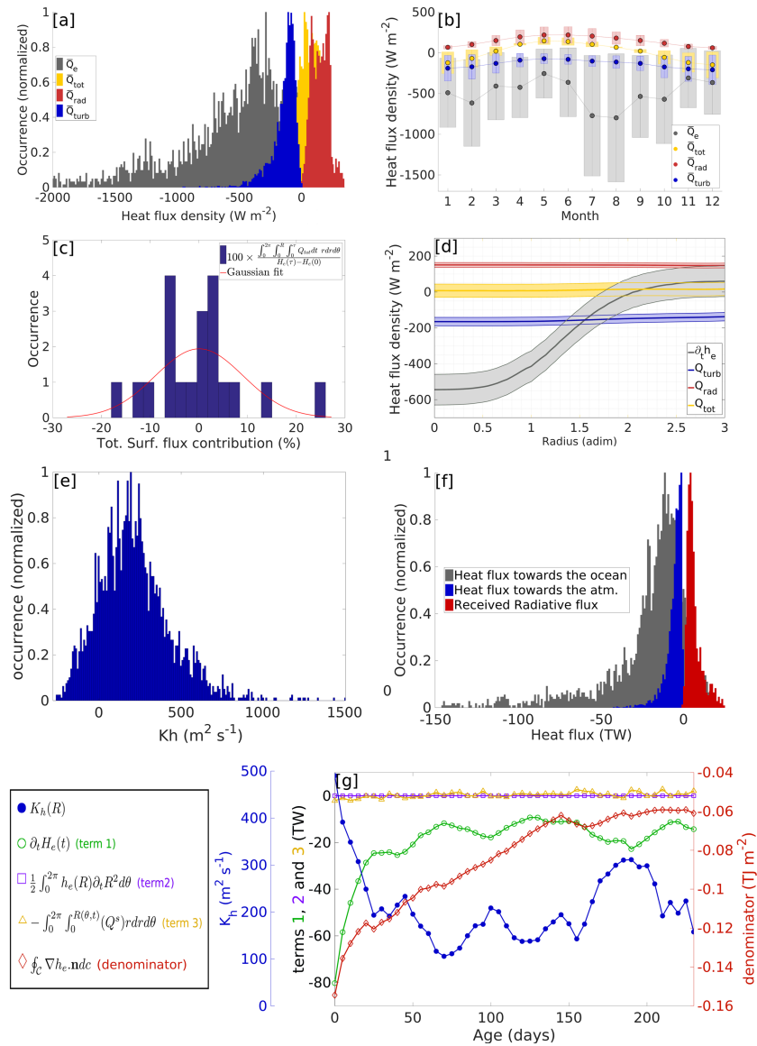
Figure 3. (a) Distribution of eddy-averaged rate of heat loss (gray bars), total surface heat flux density (yellow bars), radiative surface heat flux density (red bars), and turbulent surface heat flux density (blue bars). (b) Monthly means of eddy-averaged rate of heat loss (gray dots), total surface heat flux density (yellow dots), radiative surface heat flux density (red dots), and turbulent surface heat flux density (blue dots). The standard deviations are plotted as light color bars. (c) Distribution of the contribution of the total surface heat flux to the eddy's heat loss (blue bars). The red line represents a Gaussian fit. (d) Composite radial distribution of the eddy's rate of heat loss (gray line), total surface heat flux density (yellow line), radiative surface heat flux density (red line), and turbulent surface heat flux density (blue line). The shaded areas represent the standard deviation between the observed eddies. (e) Distribution of the depth-averaged effective lateral diffusivity coefficient ( K_h ). (f) Distribution of the heat flux toward the surrounding ocean (diffusive flux, gray bars), heat flux toward the atmosphere (turbulent surface flux and upward long-wave radiation), and the radiative heat flux received by the eddy (downward short and long wave radiations). (g) Time evolution of the mean K_h (blue line and dots), and of the different terms in equation (13).
