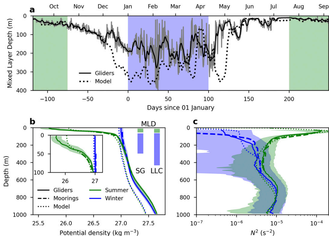
FIG. 2. (a) MLD from glider (gray line; black line is filtered through a Gaussian window with standard deviation of 1 day) and model (black dotted line, as an average over the model region marked in Fig. 1a). For the gliders, the date is in reference to 1 Jan 2013; the model reference is to 1 Jan 2012. Summer and winter times are indicated by green and blue shading, respectively. Average (b) potential density and (c) vertical stratification N^2 = b_z for summer (green) and winter (blue) from glider measurements (solid line), moorings (dashed line), and the model (dotted line). Shading indicates the 50% confidence interval for glider measurements. Inset in (b) highlights the upper 100 m of the water column. Bars in (b) represent the MLD of 90% of the measurements for winter (blue) and summer (green) from gliders (SG) and the model (LLC).
