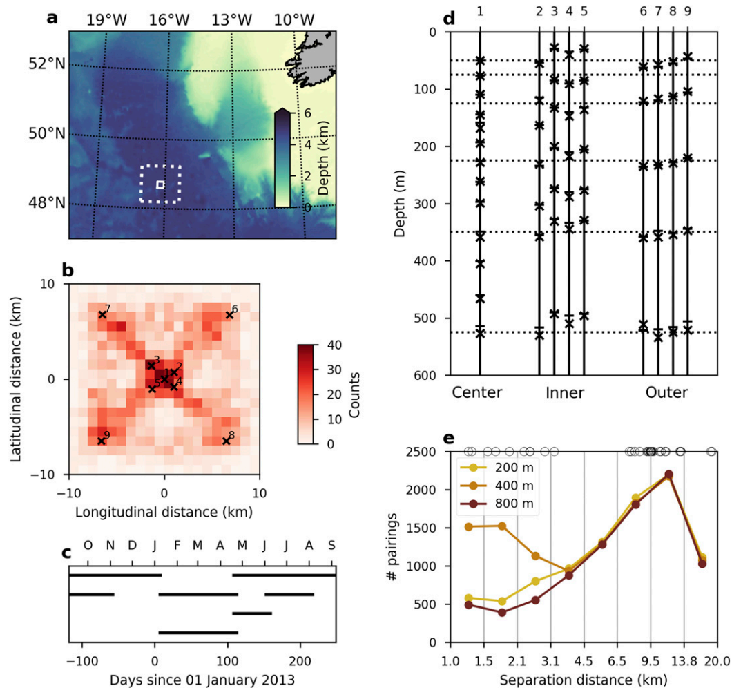
FIG. 1. (a) Bathymetry from ETOPO in the northeast Atlantic. The OSMOSIS region is shown in the white box at 48.7°N, 16.2°W. The larger region from the model is shown as the dotted white box. (b) Highlight on the OSMOSIS region, showing a histogram of glider surface locations (colors) and the positions of the nine moorings (x marks). (c) Periods of time in which the gliders were active. (d) Depth placement of the ACMs (x marks) and CTDs (dash marks) for each mooring. Dotted horizontal lines denote the depths over which mooring structure functions were calculated. (e) Histogram of structure function pairings from glider measurements at 200-, 400-, and 800-m depth. Bins are equally spaced logarithmically. Circle markings at the top axis show the separations between moorings.
