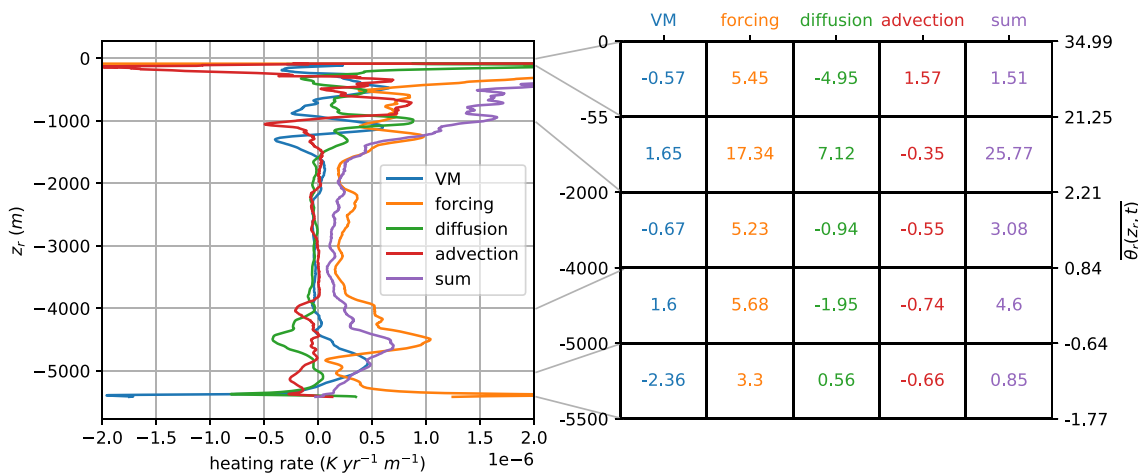
Fig. 10 Left panel: difference between the 2xCO 2 and Control runs of the temperature tendencies terms divergence (positive values mean that temperature in the 2xCO 2 increases compared to CR) as a function of reference depth ( z_r ). VM is in blue, forcing in orange, diffusion in green, advection in red and the sum of all terms in purple. Right panel: vertical integral of the left panel terms over five ranges
