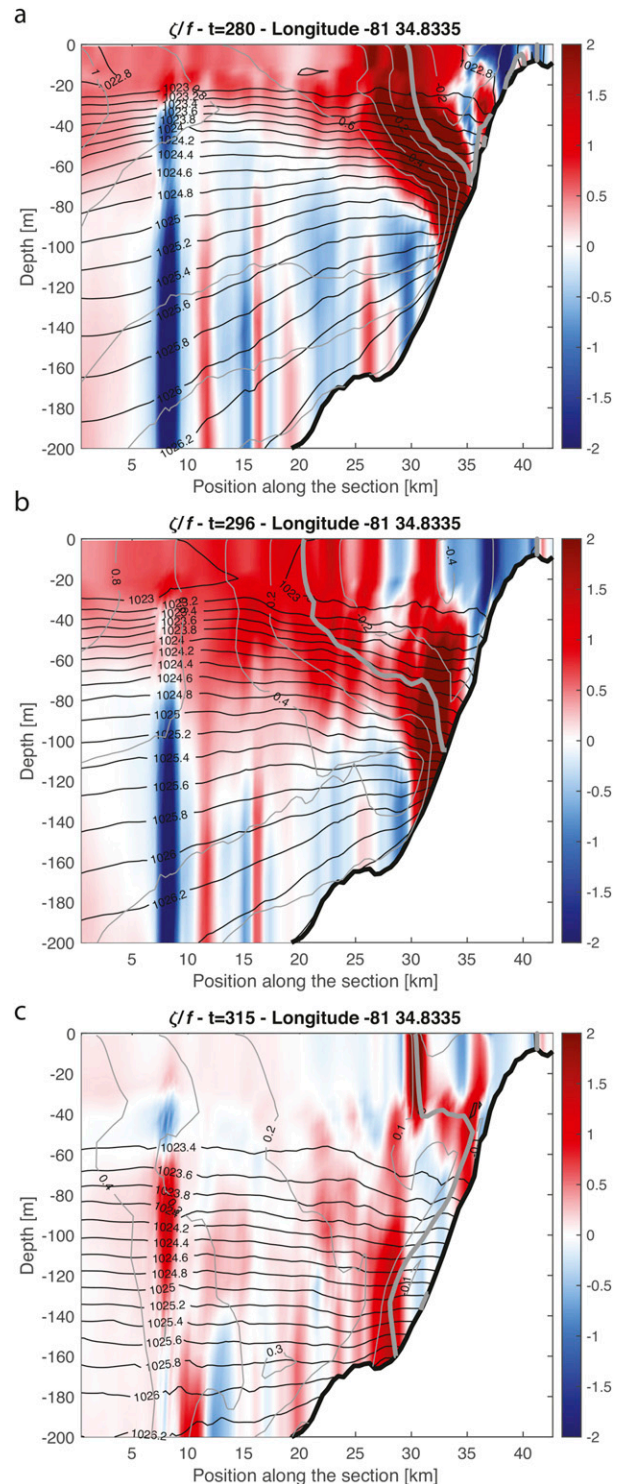
FIG. 13. Relative vorticity ( \zeta/f ) cross sections at 81^{\circ}34.8335'W showing the position of the Florida Current relative to the shelf slope before the passage of (a) LSE1, (b) LSE2, and (c) ME1.
