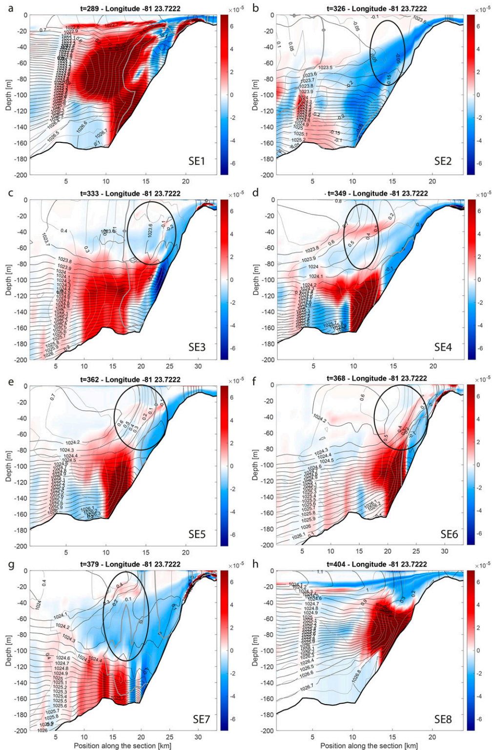
FIG. 10. Sequence of Ertel's vorticity anomaly ( s^{-3} ) cross sections at 81^{\circ}23.7222'W 1 or 2 days prior to the formation of the subsynoptic eddies (a) SE1, (b) SE2, (c) SE3, (d) SE4, (e) SE5, (f) SE6, (g) SE7, and (h) SE8. The time t in model days is indicated above each panel. Black contours show the density in kg\ m^{-3} . The density interval is 0.1\ kg\ m^{-3} . Gray contours show the zonal velocity in m\ s^{-1} . Gray thick line shows the zero-velocity contour. The velocity interval is 0.05\ m\ s^{-1} . The circled area shows the region where Ertel's vorticity anomaly changes sign vertically.
