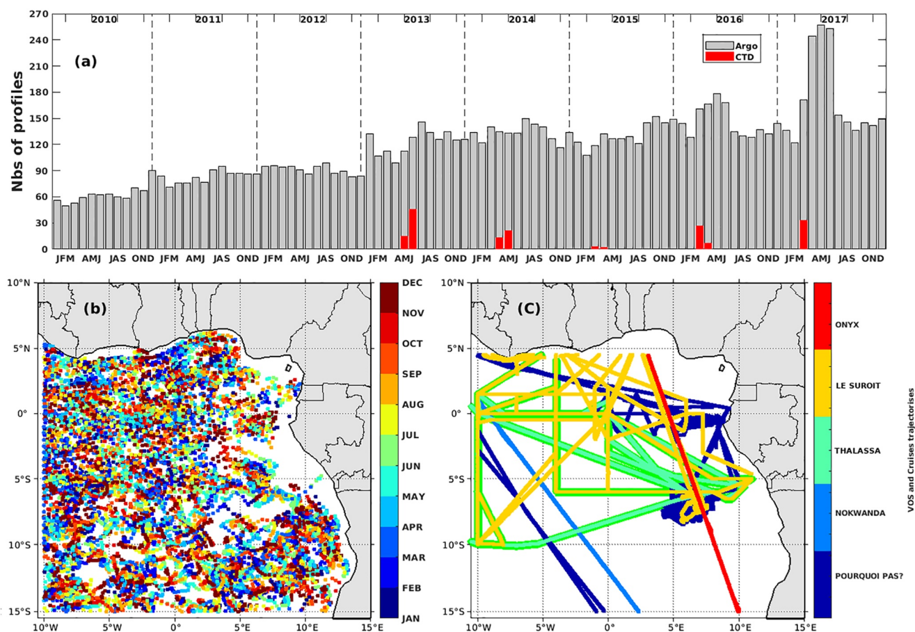
Figure 2. (a) History of Argo float and CTD PIRATA FR profiles from 2010 to 2017 in the Gulf of Guinea; (b) Spatial distribution of the profiles per month; (c) VOS (ONYX, NOKWANDA, and POURQUOI PAS?) trajectories for TSG SSS measurements and PIRATA (LE SUROIT and THALASSA) cruises in the GG. CTD, Conductivity Temperature Depth; GG, Gulf of Guinea; SSS, Sea Surface Salinity.
