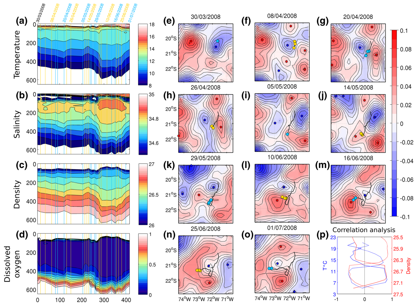
Figure 3. Vertical sections of (a) temperature (°C), (b) salinity, (c) density (kg/m 3 ), and (d) DO (ml/L) as a function of the accumulated distance between consecutive profiles (x-axis) from the “CL001072” profiling float in the PFL data set (March 30 to July 1, 2008, WOD2013), together with selected snapshots (e–o) of sea level anomalies (Pujol et al., 2016) within the time period of the section. Temperature, density and DO values out of the ranges 3–23°C, 25.5–27.5 kg/m 3 , and 0–1 ml/L, respectively, are shaded white. In each snapshot, stars indicate the eddy center, circles show the coordinates of all the stations sampled since the date of the preceding snapshot, and the color scale represents the sea level anomaly (blue in CE, red in AE). Vertical lines and circles in subplots a–d and e–o, respectively, are alternately differentiated in color to distinguish different sets of profiles (a–d) in each snapshot (e–o). The bottom-right corner diagram (p) represents the individual patterns of Pearson’s correlation between the depth of isopycnals in the 25.5–27.5 kg/m 3 range, shown in red (isotherms in the 3–23°C range, shown in blue) and the depth of the upper/lower limits of the OMZ (dashed and solid lines, respectively), considering the profiles in subplots 3a to 3d. DO, dissolved oxygen; OMZ, oxygen minimum zone; WOD, World Ocean Database.
