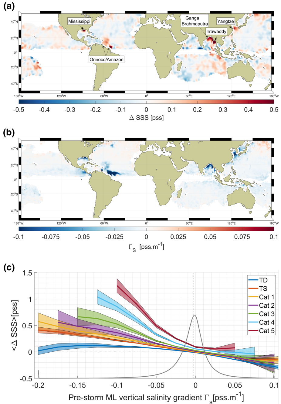
Figure 3. (a) Temporal average (2010–2019) of all storms SSS response in 1^\circ \times 1^\circ boxes. (b) Average pre-storm mixed-layer vertical salinity gradient \Gamma_s in 1^\circ \times 1^\circ boxes. (c) Radially integrated (within |r/R_{\max}| \leq 10 ) SSS response to Tropical Cyclones bin-averaged as function of SSS storm intensity (colors) and of \Gamma_s (x-axis, bin width of 0.025 pss/m). The gray curve and black dashed vertical line are the distribution of \Gamma_s (scaled to fit the graphic) and its median value, respectively. The color patches indicate the extent of the 95% confidence interval for the mean (thin black curves) in each bin. SSS, sea surface salinity; SSWS, Saffir-Simpson Wind Scale.
