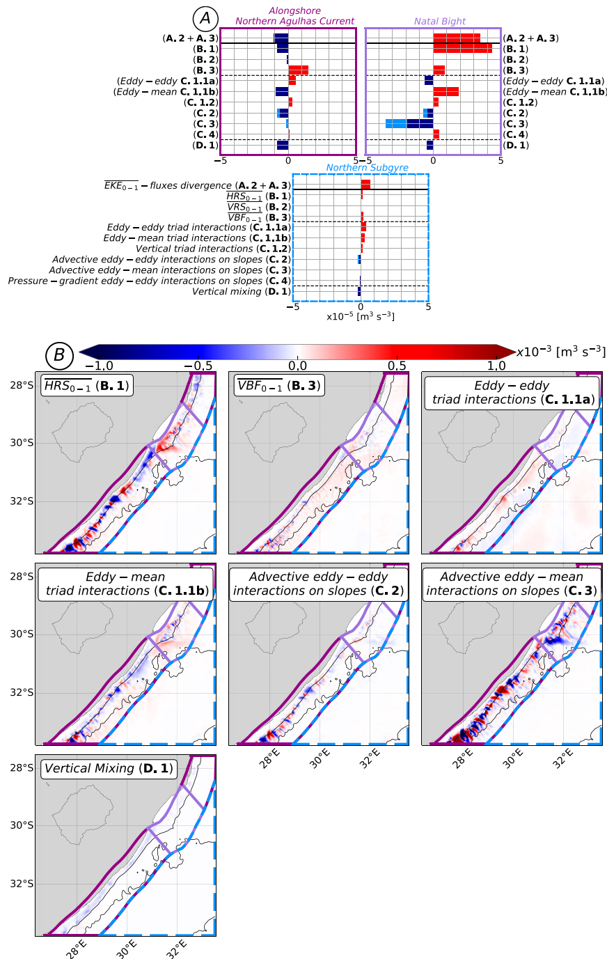
FIG. 6. (a) Spatial averages of the contributions of the \overline{EKE}_{0-1} budget [Eq. (29) for n = 0 + 1 ] ( \text{m}^3 \text{ s}^{-3} ) over the three NAC subareas. It is constituted of the net \overline{EKE}_{0-1} budget (A terms) denoted by a solid black line from the \overline{EKE}_{0-1} sources and sinks (B, C, and D terms) denoted from each other by dotted black lines. The bars color denotes the sign of the spatially averaged terms (red/blue: positive/negative). For the C.2 and C.3 terms, the dark (light) blue color denotes the n = m \neq l, n = l \neq m, n \neq m = l, n \neq m = l ( n = m = l ) cases. (b) Maps of the main \overline{EKE}_{0-1} sources and sinks [B, C, and D terms in Eq. (29) for n = 0 + 1 ] ( \text{m}^3 \text{ s}^{-3} ) in the NAC. The black isolines denote the 1000- and 3000-m isobaths. The Alongshore Agulhas Current (dark purple area) \overline{EKE}_{0-1} sink is constituted of the B.1, eddy-mean C.1.1b, C.2, and D.1 contributions; the Natal Bight (light purple area) \overline{EKE}_{0-1} source is mainly constituted of the B.1 contribution; and the Northern Subgyre (dashed light blue area) \overline{EKE}_{0-1} source is mainly constituted of the eddy-eddy C.1.1a contribution.
