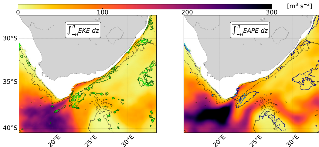
FIG. B1. Vertically integrated (left) \overline{EKE} and (right) \overline{EAPE} ( m^3 s^{-2} ). The green contours denote the 1% (dark), 2% (light), and 5% (extra light) isolines of \overline{EKE} residual (left panel), the blue contours denote the 5% (dark), 10% (light), and 20% (extra light) isolines of \overline{EAPE} residual (right panel), and the black contours denote the 1000- and 3000-m isobaths (all panels). Residuals are a measure of the validity of the modal decomposition of the modeled eddy energies using the 10 first vertical modes. They are defined as the difference between the total energies and their modal expansions normalized by the total energies and converted into percentages (%). With the \overline{EKE} and \overline{EAPE} residuals locally peaking at 5% and 20%, respectively, over limited areas, the 10 first vertical modes accurately represent the modeled eddy energies.
