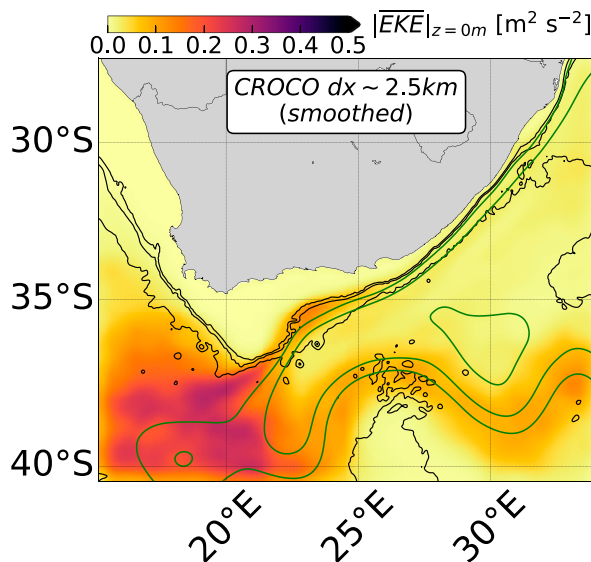
FIG. A1. Surface \overline{EKE} [ m^2 s^{-2} ] for CROCO dx \sim 2.5 km. \overline{EKE} is defined from geostrophic velocities diagnosed from the smoothed (length scale of 100 km) sea surface height fluctuations and time fluctuations are defined relatively to a 1-yr running with a 1-month stepping over the 1994–99 period. The green contours denote the 0.25-, 0.5-, 0.75-, and 1-m isolines of mean sea surface height and the black contours denote the 500-, 1000-, and 3000-m isobaths. The patterns and amplitudes of the smoothed modeled \overline{EKE} denote an Agulhas Current variability in high agreement with the observed one (Fig. 2, top left).
