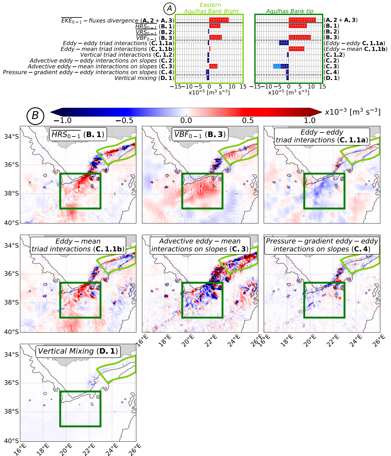
FIG. 7. (a) Spatial averages of the contributions of the \overline{\text{EKE}}_{0-1} budget [Eq. (29) for n = 0 + 1 ] ( \text{m}^3 \text{s}^{-3} ) over the two SAC subareas. (b) Maps of the main \overline{\text{EKE}}_{0-1} sources and sinks [B, C, and D terms in Eq. (29) for n = 0 + 1 ] ( \text{m}^3 \text{s}^{-3} ) in the SAC. The black isolines denote the 1000- and 3000-m isobaths. The Eastern Agulhas Bank Bight (light green area) and Agulhas Bank tip (dark green) \overline{\text{EKE}}_{0-1} sources are constituted of the B.1, B.3, and C.1.1b contributions, but the C.3 term has an opposite contribution between the two areas. The eddy–eddy C.1.1a has a positive contribution away from the mesoscale eddies generation locations, the C.4 negative contribution is localized around topography and the D.1 negative contribution is spread over the region.
