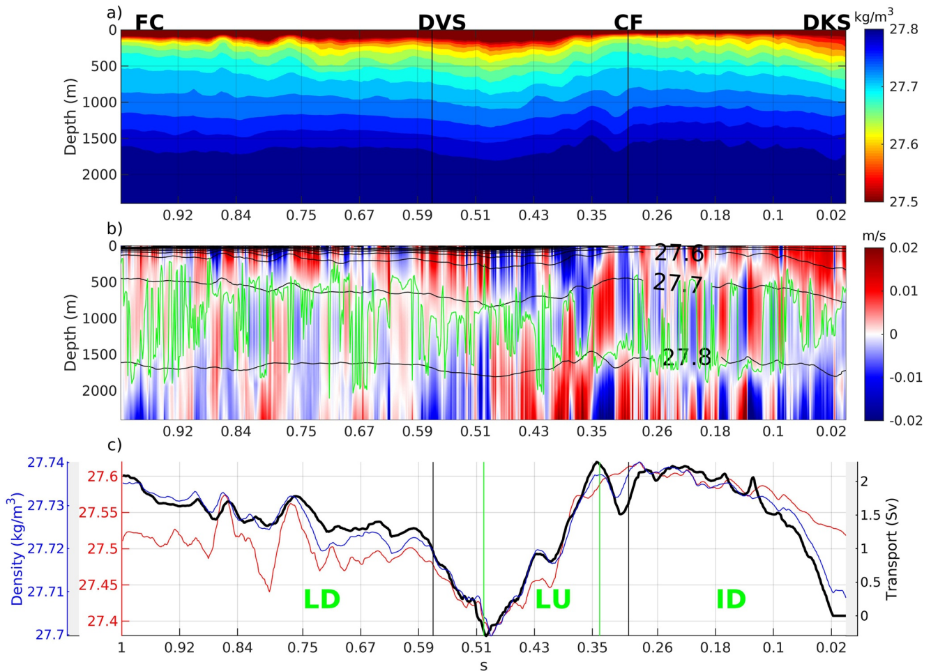
Figure 3. (a) Optimal interpolation-derived multiproduct density ( \sigma_0 ) field along isobath 2400 m. (b) The cross-shore geostrophic velocity field along isobath 2400 m. The positive (negative) values indicate inshore (offshore) flows. The green line indicates the depth at which the maximum (accumulated) vertical transport is found (i.e., levels of no motion). The \sigma_0 = 27.6, 27.7, 27.8 \text{ kg m}^{-3} isopycnals are contoured in black. (c) The density along the boundary from s = 0 to s = 1 averaged in the upper layer (1–300 m, red curve) and the intermediate layer (301–1500 m, blue curve). The maximum vertical transport (black curve) accumulated along the boundary from s = 0 to s = 1 . The upward slopes indicate the downwelling (LD-Labrador Downwelling, s = 0.5-1 , ID-Irminger Downwelling, s = 0-0.33 ), and the downward slope indicates upwelling (LU-Labrador Upwelling, s = 0.33-0.5 ).
