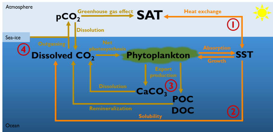
Figure 1. Representation of the four different biologically induced pathways that affect the atmospheric temperature. (1) Marine biota via phytoplankton light absorption increases the SST, changing therefore the air–sea heat exchange and the atmospheric temperature. (2) Changes in SST also alter the solubility of CO 2 and its dissolved concentration. In turn, changes in dissolved CO 2 concentrations alter the air–sea CO 2 exchange and thus the greenhouse gas effect. (3) Phytoplankton light absorption modifies the marine biogeochemical cycles and particularly the export production of carbon. These changes in export production of carbon modify the dissolved CO 2 concentration and the greenhouse gas effect. (4) A warmer surface of the ocean can decrease the sea-ice extent. A reduction of sea-ice cover increases the air–sea CO 2 exchange area, changing the greenhouse gas concentrations. SAT: surface atmospheric temperature. SST: sea surface temperature. CaCO 3 : calcium carbonate. POC: particulate organic carbon. DOC: dissolved organic carbon.
