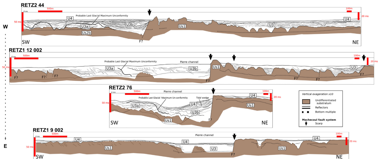
Figure 8. Representative sample of interpreted seismic profiles of RETZ1 and 2 cruises (Le Roy et al. 2016; Kaub et al. 2017), with a 10-times vertical exaggeration (see Fig. 4 for profiles location and appendices Figs. A1 and A2 for raw data, and appendix Fig. A3 for seismic facies description).
