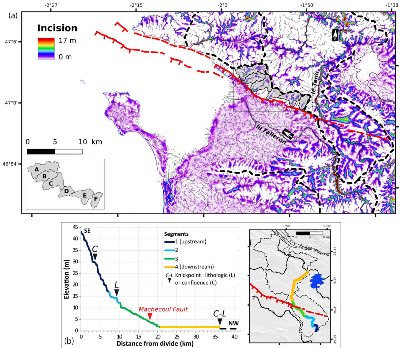
Figure 6. (a) Incision map, hydrographic network with main catchments (black dashed lines) and catchments draining the morphological scarp of the Machecoul Fault (grey, a to f from west to east, see also insert map), Machecoul Fault (red). (b) Long profile of Tenu river.
