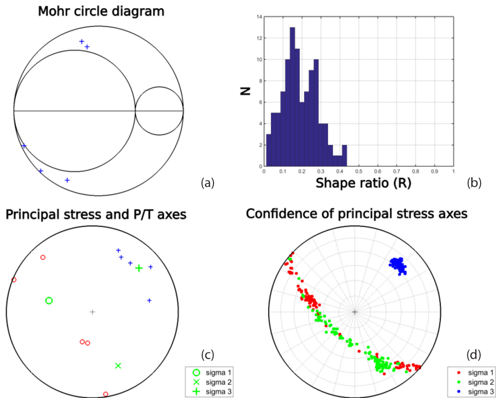
Figure C1. Stress inversion from fault plane solutions (Fig. 11b, except the n^{\circ}27 focal mechanism) using the Vavryčuk (2014) method. (a) Mohr's circle diagram, (b) Histograms of the shape ratio R , (c) P/T axes and (d) Confidence limits of the principal stress directions.
