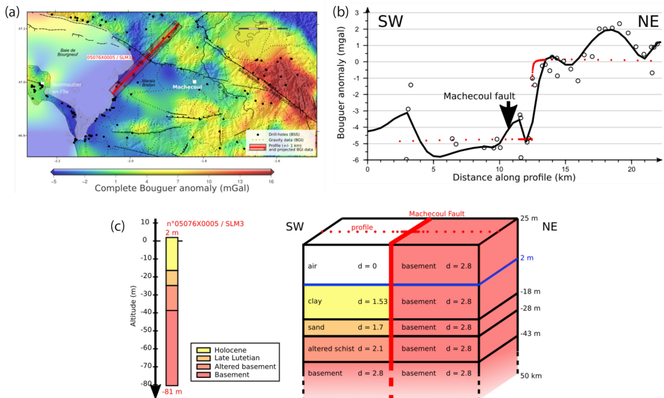
Figure B1. (a) Zoomed map (see Fig. 9 for the same map but bigger size) of complete Bouguer anomaly interpolation calculated from the free air anomaly provided by the BGI around Machecoul Fault. A slight white mask is applied to the offshore interpolation, considering the lack of data offshore. Small black circles are gravity data points from BGI, big black circles are drill holes from BSS used in this study. Red line is the profile and encircled small black circles are projected data points represented on the profile. (b) Profile. Small black circles are gravity data points from BGI. Calculated complete Bouguer anomaly response of our model (red dots) and observed complete Bouguer calculated from BGI data (black line). (c) 2-D density structure model of the Marais Breton and the Machecoul Fault in the considered area. The depths and densities of each layer were constrained by the 5076X0005/SLM3 drill hole (BSS) visible in (a).
