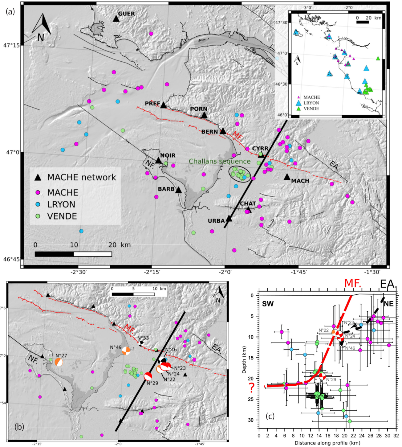
Figure 11. (a) Spatial distribution of earthquakes collected between 2011 July and 2017 October in the Marais Breton and Baie de Bourgneuf area (error in depth equal or less than 10 km). Colours represent catalogues of the three different networks (location of stations are represent on the onset map: VENDE network (green), LRYON network (blue) and MACHE network (pink); see electronic supplement for catalogue and uncertainties). MF: Machecoul Fault. NF: Noirmoutier Fault. EA: Les Essarts Accident. (b) Representation of the eight focal mechanisms determined for internal events of the MACHE (2016–2017) network. Colours depending on quality (A black, B orange, C red, see electronic supplement for focal solutions). (c) Cross section normal to the surface expression of the Machecoul Fault. Hypocentres in a 10 km wide area on both sides of the cross-section are projected with error bars (depth and epicentral location, see electronic supplement for catalogue and uncertainties).
