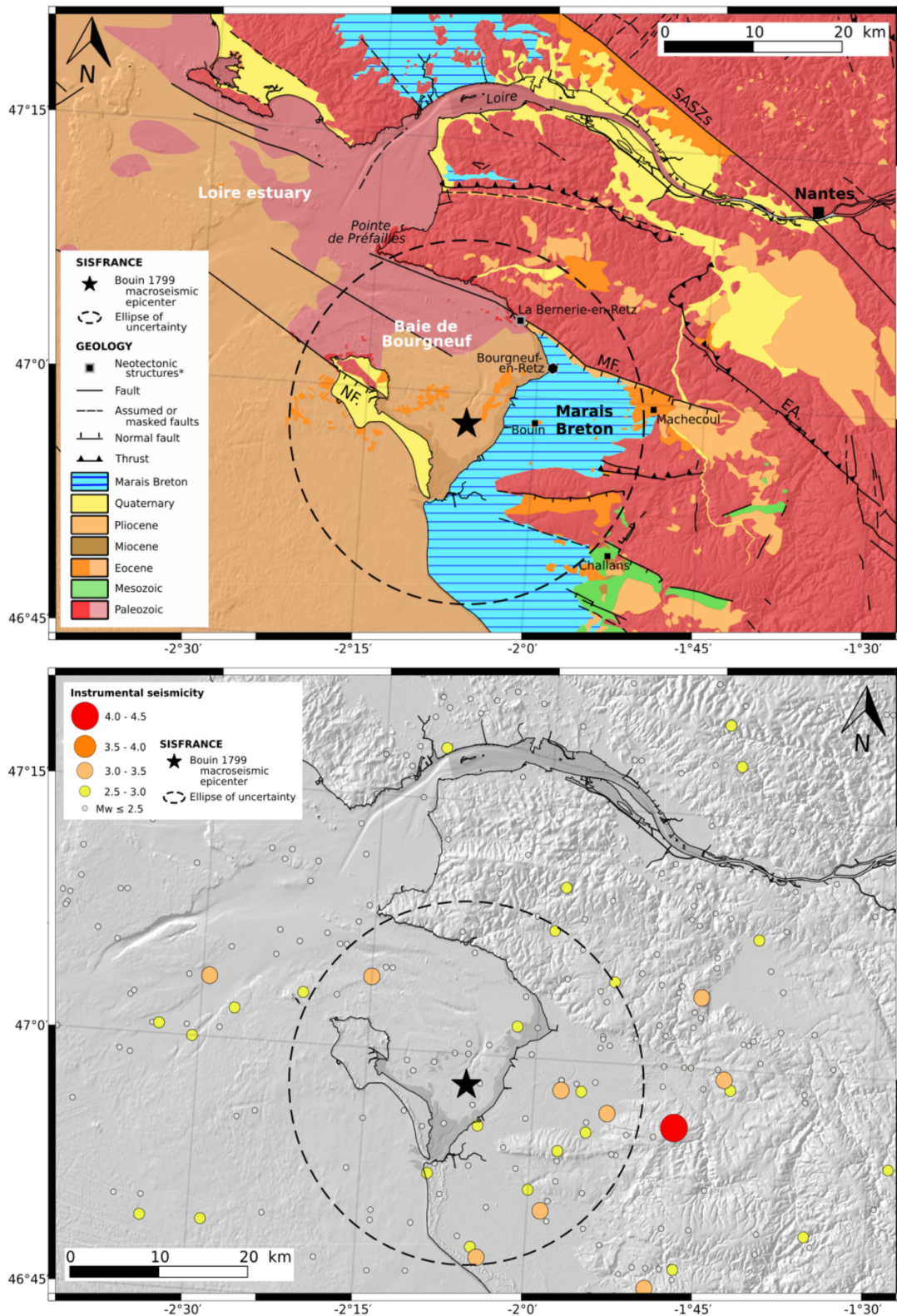
Figure 3. Simplified geological map of coastal Vendée (top panel) and seismological data available from 1962 to 2014 (Si-Hex and CEA-LDG catalogues, bottom panel). The SISFRANCE macroseismic epicentre of the 1799 Bouin earthquake and its 20 km ellipse of uncertainty are represented (SisFrance, https://sisfrance.irsn.fr/ ). The location of the neotectonic structures in La Bernerie-en-Retz, previously described by Baize et al. (2002) is specified (see text and Appendix Fig. D1). MF: Machedoul Fault. NF: Noirmoutier Fault. EA: Les Essarts Accident. SASZs: South Armorican crustal Shear Zone south.
