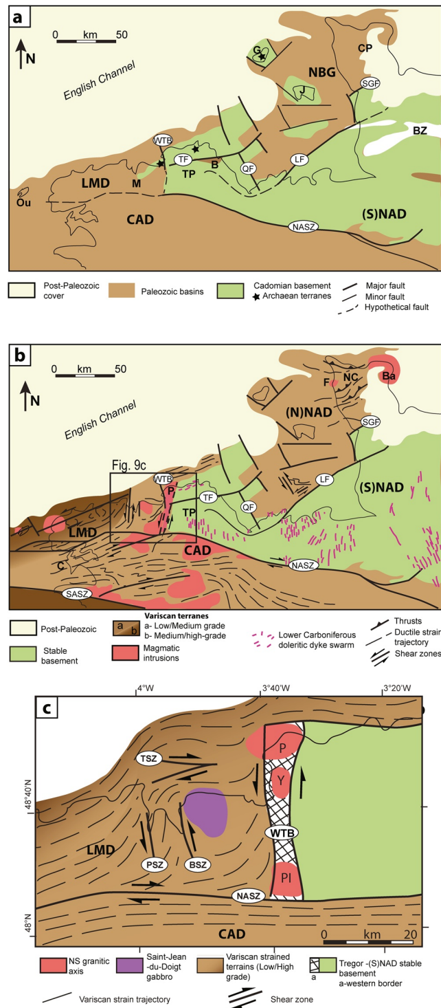
Figure 9. Evolution of Northern Armorica in Paleozoic times. (a) Structural arrangement of the Cadomian-floored NAD into a northern basin (NBG) and its southern basement margin (SNAD) at a pre-Carboniferous basinal stage. Present-day coastline drawn as geographical coordinates. Same abbreviations as in Figure 2a. (b) Variscan structural pattern (340–300 Ma). Location of Figure 9c is shown. Same abbreviations as in Figures 2a and 8b. (c) Indenter kinematic model showing the anomalous sigmoid trajectory of Variscan ductile strain against the western edge of the (S)NAD Cadomian block (Morlaix-Tregor transition zone). Variscan granites are not shown for clarity, excepted the NS magmatic axis along the WTB structure. Same abbreviations as in Figure 8b. Location in Figure 9b.
