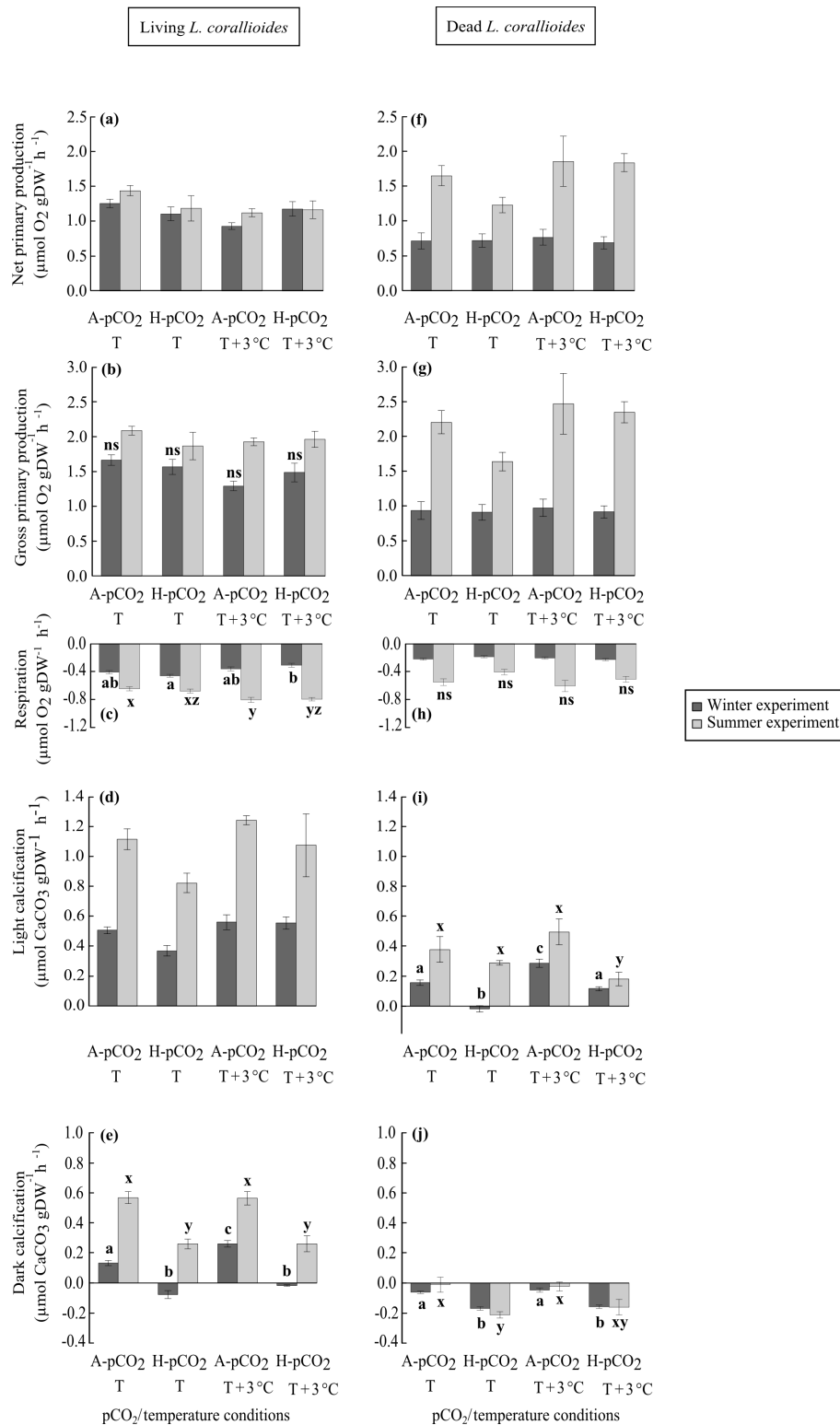
Figure 2. Net and gross primary production, respiration, and light and dark calcification rates (mean ± SE, n = 5 ) of living (a–e) and dead thalli (f–j) of L. corallioides in the different p\text{CO}_2 (A- p\text{CO}_2 is ambient p\text{CO}_2 ; H- p\text{CO}_2 is high- p\text{CO}_2 ) and temperature ( T is ambient temperature; T + 3^\circ\text{C} is high temperature) treatments after 3 months in winter (dark gray) and summer conditions (light gray). Letters indicate significant differences between the four treatments in winter (a, b, c) and summer (x, y, z) conditions (Tukey HSD test). ns is not significant. Tukey tests were performed when a significant effect of temperature or p\text{CO}_2 was detected using two-way ANOVAs.
