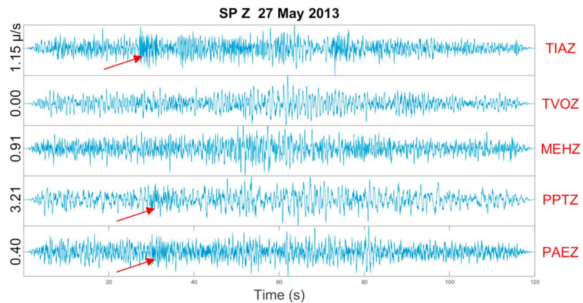
Figure 2. Sequence of short-period volcanic tremor consisting of Pb and Pn waves of fluctuating amplitude at Rocard volcano. The red arrows point to parts of the signals with high-frequency volcanic tremor that are missing from the stations of Mehetia (MEH) and Taravao (TVO). The location of the 2013 epicenters was determined by data received by the Rangiroa network at a distance of 200 km, which also recorded the Pn waves of these rare impulsive events.
