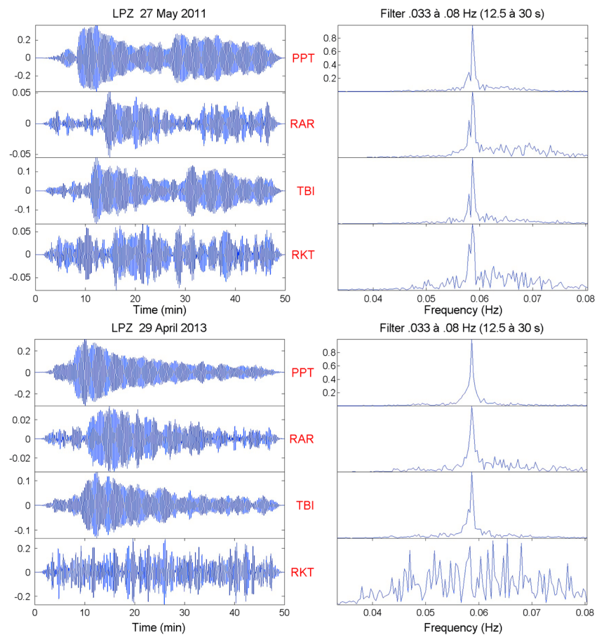
Figure 3. Rayleigh wave trains of long period visible at PPT (Tahiti: Society archipelago), TBI (Austral Islands), RAR (Cook Islands), and RKT (Gambier Islands). Two successive although overlapping sequences occurred in 2011. In 2013, only one was observed, its amplitude a little weaker and masked at RKT by strong microseismic noise. The frequency of the signal was perfectly monochromatic, at 0.0589 Hz (17.0 s), and was identical in the two cases.
