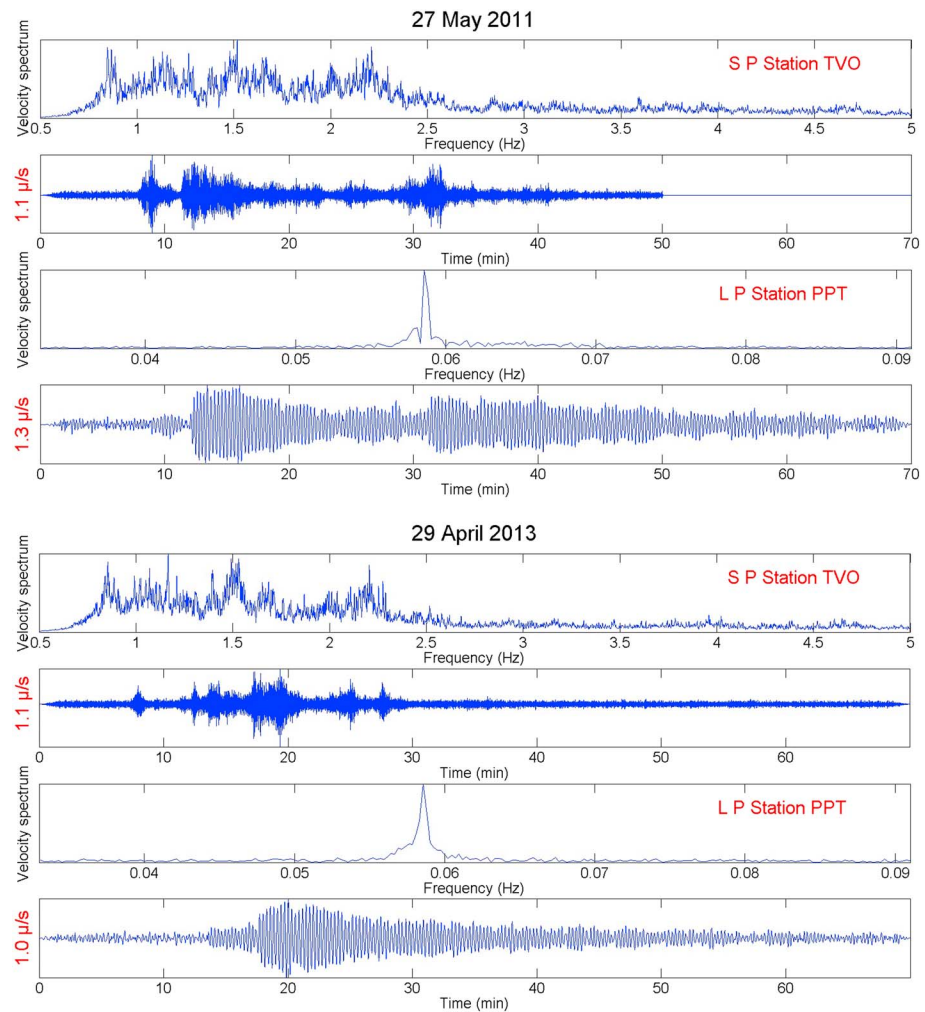
Figure 4. Comparison of the 2011 (top) and 2013 (bottom) seismic events: (a) frequency spectrum and (b) short-period events recorded at TVO (80 km away from the source); (c) frequency spectrum and (d) long-period events recorded at PPT (110 km away from the source). In 2011 and 2013, the short-period events preceded the long-period Rayleigh wave train by about 10 min. Short and long-period records are referenced at the same time.
