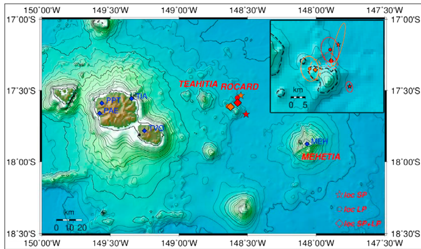
Figure 1. Map showing the locations (in blue) of the seismic stations on three different volcanic edifices of the Tahiti-Mehetia hot spot (Mehetia MEH, Taravao TVO, and Tahiti TIA, PPT, and PAE) and the epicenters deduced from the data of (i) short-period events (Pb, Pn) shown as stars, (ii) long-period events (Rayleigh) shown as circles, and (iii) associated events of both short and long periods shown as diamonds. The inset shows the confidence ellipses (red: 2013; orange: 2011) which frame the submarine volcano Rocard but do not provide a precise location of the sources with respect to the edifice. Thick lines denote the -3300 m isobath.
