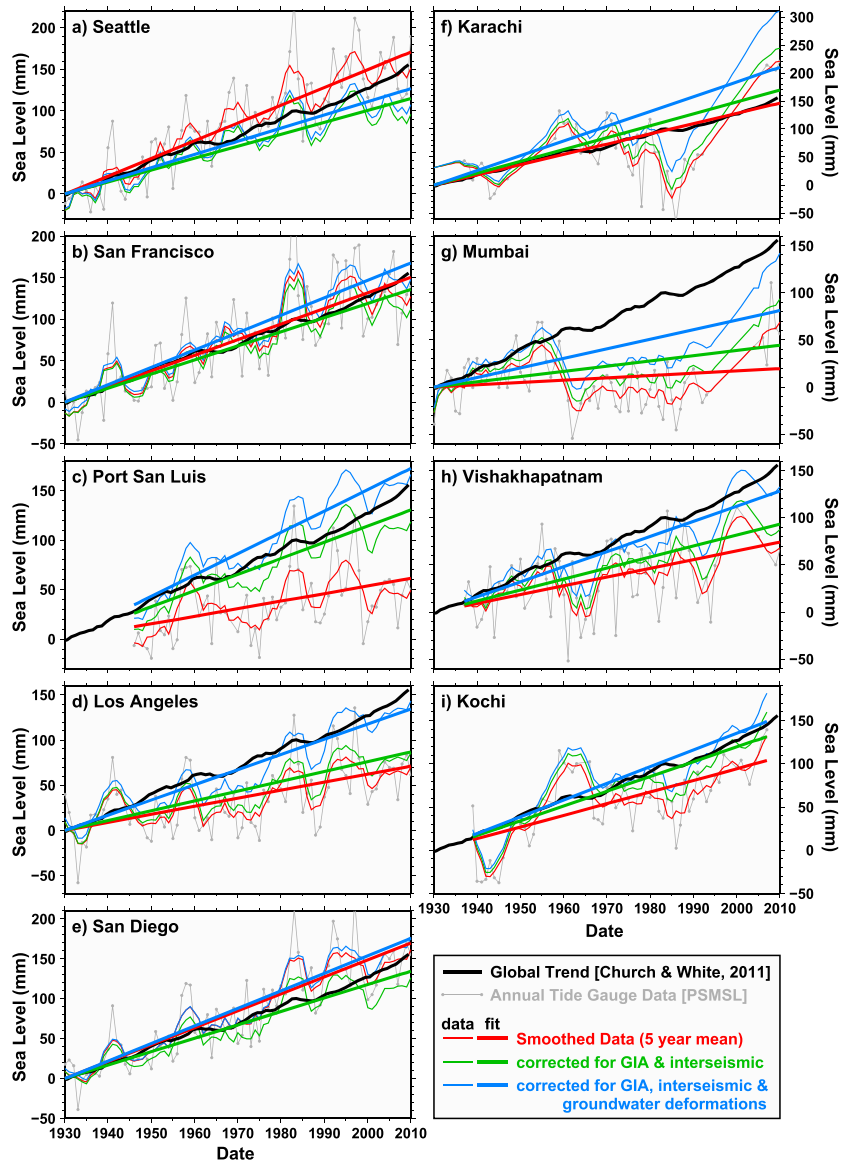
Figure 3. Comparison of selected tide gauge records (locations in Figure 1), both before and after the application of the successive corrections (colored lines), with Church and White's [2011] global sea level reconstruction (black curve). Annual mean sea level data from the PSMSL (grey dots), with gaps filled by linear interpolation, are expressed here relative to their values in 1930 in raw form (grey lines), after application of a 5 year running mean (red lines), after correcting for GIA and interseismic deformations (green lines), and after additionally correcting for deformation due to groundwater depletion (blue lines). Estimates of long-term rates of sea level rise (Table 1) are computed from these curves using a linear fit (thick lines) to the sea level records (thin lines) between 1930 and 2010.
