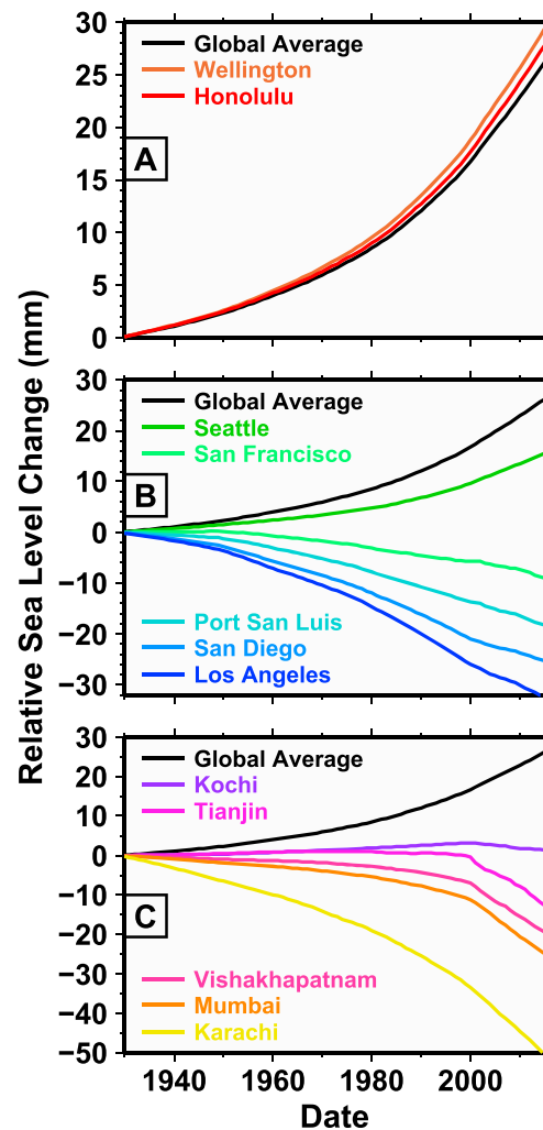
Figure 2. Model prediction of the relative sea level change caused by groundwater depletion since 1930. Here global average rise (black curves) is compared with trends at individual tide gauges (colored curves, labeled in order, locations in Figure 1) that are (a) far from depletion zones or close to regions of intense groundwater depletion in (b) western North America and (c) southern Asia.
