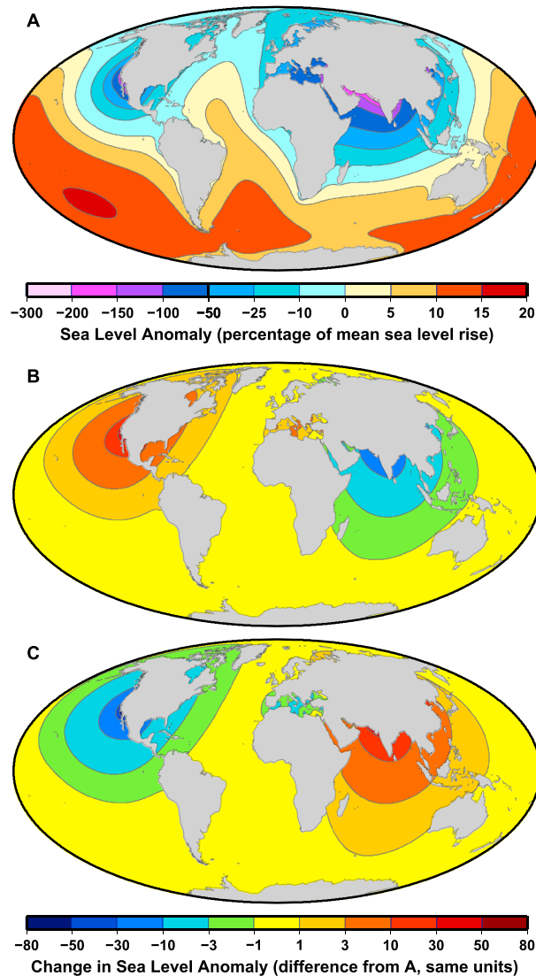
Figure 4. Spatial variations in relative sea level change for different models of groundwater depletion in the year 2000. (a) Deviations from mean sea level, shown as a percentage of the global average rise of 0.57 mm caused by Wada et al. 's [2010] estimate of 204 km 3 of groundwater loss. Changes to this pattern result from different distributions of continental groundwater loss, as shown here relative to Figure 4a for models in which the ~20% uncertainty range estimated by Wada et al. [2010] is either (b) maximized in Asia and minimized in North America or (c) maximized in North America and minimized in Asia.
