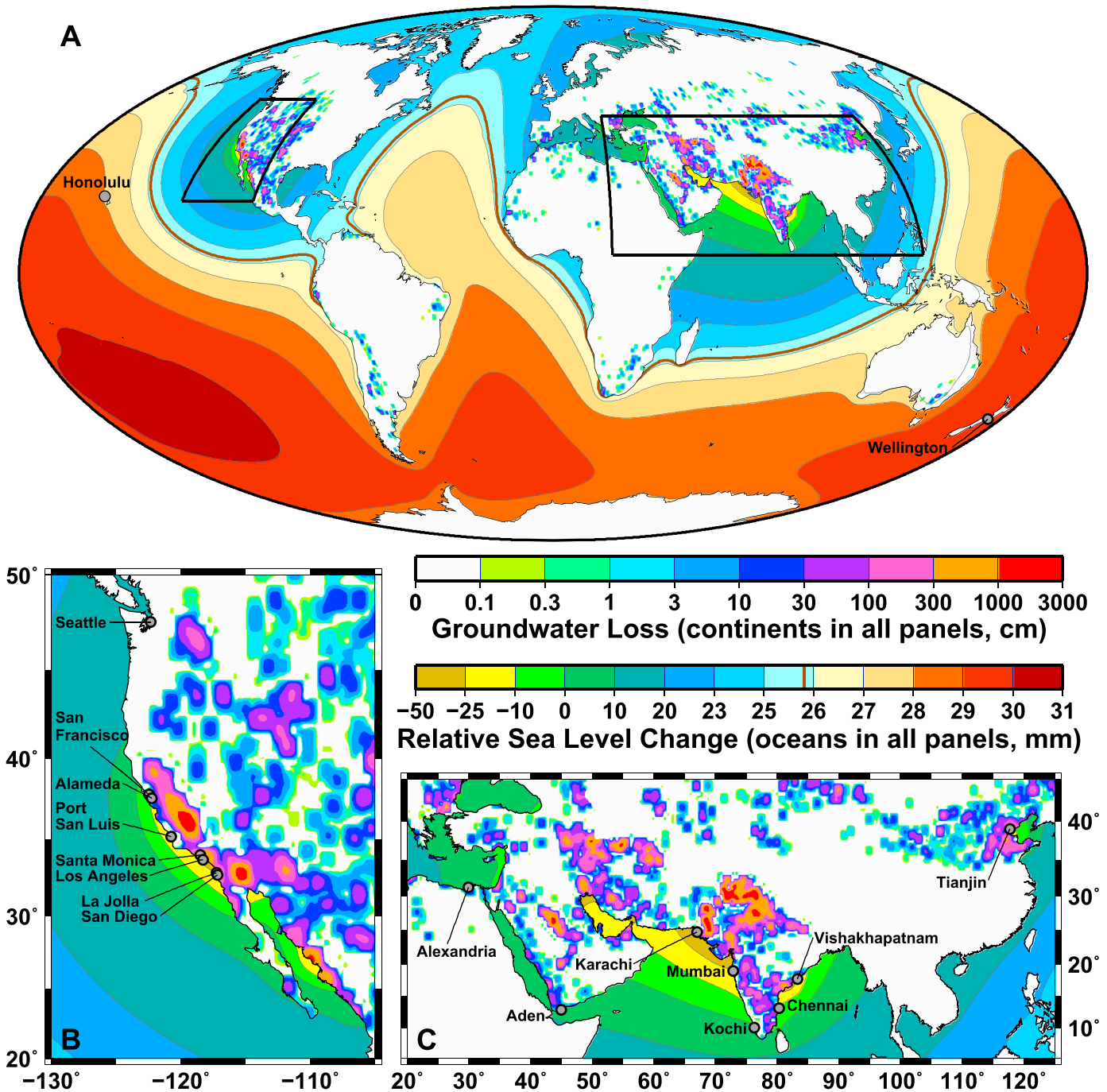
Figure 1. Cumulative groundwater loss from the continents from 1930 to 2015 (shown as colors in continental regions as a thickness of equivalent water layer removed, based on updated data from Wada et al. [2012]), and the spatially varying relative sea level rise that results from this groundwater loss to the oceans (shown as colors in oceanic regions, global average of 25.8 mm denoted by brown line). (a) Global patterns and details of (b) western North America and (c) southern Asia show depressed relative sea level near regions of large groundwater loss. Grey circles give locations of tide gauge stations examined for this study (Table 1).
