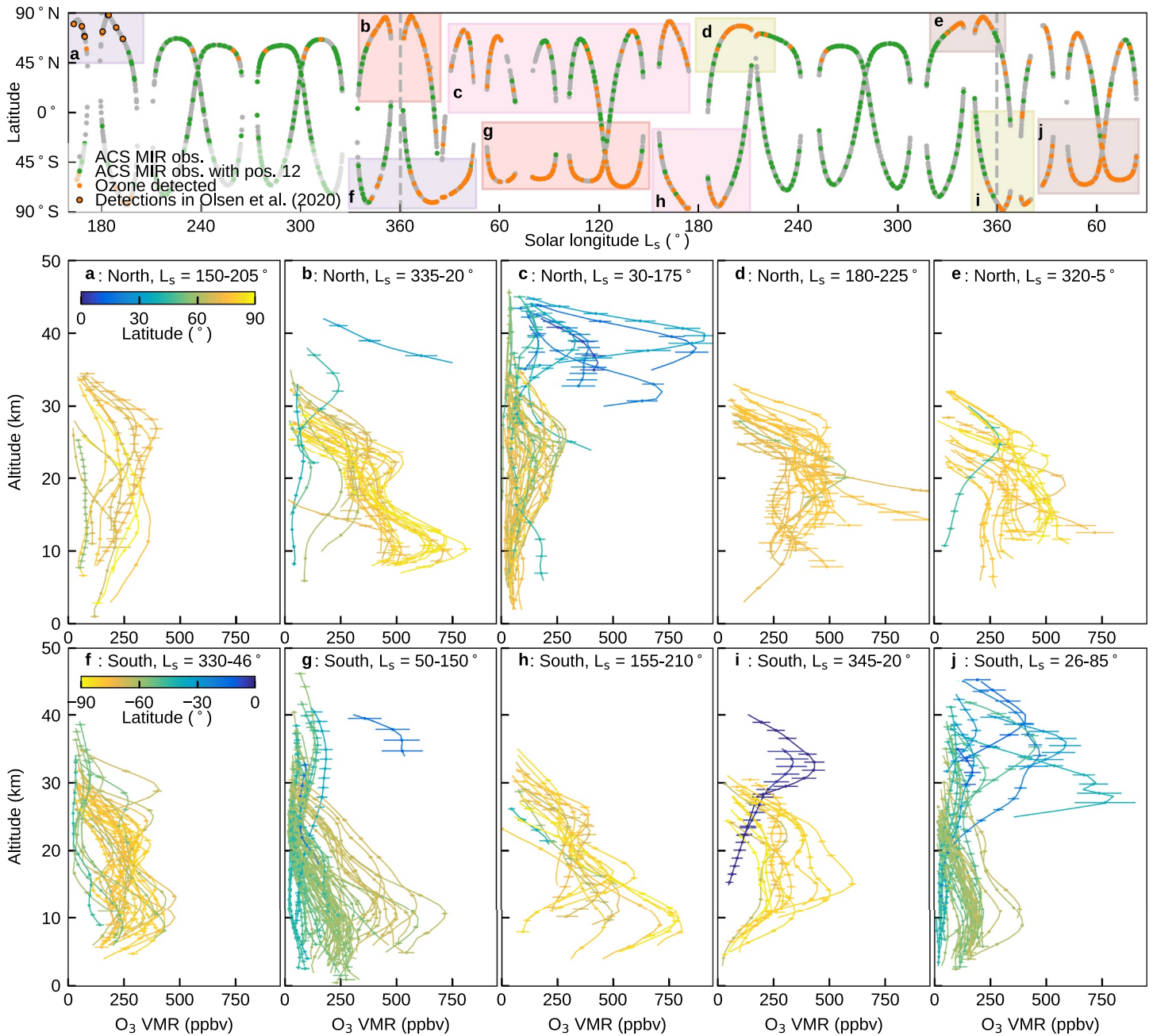
Figure 2. Overview of ozone detections with atmospheric chemistry suite mid-infrared (ACS MIR). The top panel shows the distribution of latitudes probed by ACS over time (solar longitude L_s ) since the start of the mission on L_s 163° in Mars year (MY) 34 through to the end of MY 35 and into the beginning of MY 36. All ACS occultations are indicated in gray, those using secondary grating position 12 green, and those with 3\sigma ozone detections are highlighted in orange. Positive detections are grouped by L_s and latitude, and the retrieved vertical profiles are shown in the lower panels. Panels a–e cover the northern hemisphere, and panels f–j cover the southern hemisphere.
