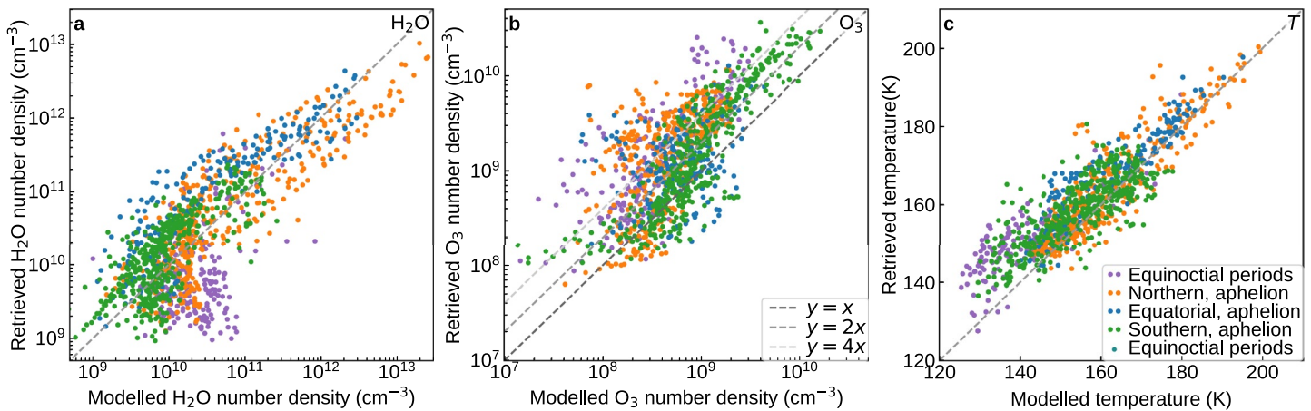
Figure 10. Comparison of H 2 O, O 3 , and temperature retrieved from ACS data and computed by the LMD global climate model (GCM). Each retrieved tangent height where O 3 retrievals were made in an occultation sequence are shown. Pressure levels of the profiles extracted from the LMD GCM are interpolated to those of ACS tangent heights. Panels show: (a) H 2 O number density retrieved from ACS MIR and modeled by the LMD GCM; (b) O 3 number density retrieved from ACS MIR and modeled by the LMD GCM; (c) temperature retrieved from ACS near-infrared channel (Fedorova et al., 2020, 2022) and modeled by the LMD GCM. Dashed gray lines indicated one-to-one correlation. Panel b also has lines indicating when the retrieved O 3 values are twice, or 4-times the modeled values. Colors indicate groupings of latitude and season.
