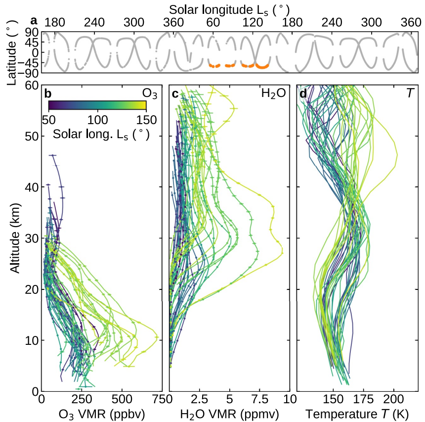
Figure 4. Aphelion ozone observations during southern winter. Panel a shows the latitude and L_s of observations, volume mixing ratio vertical profiles of ozone (panel b) and water vapor (panel c) retrieved from atmospheric chemistry suite mid-infrared (ACS MIR), and temperature retrieved from ACS near-infrared channel (panel d). Colors indicate L_s . These profiles were measured at middle southern latitudes ( 55^{\circ}\text{S} – 66^{\circ}\text{S} ) during the aphelion period (southern winter) and correspond to Figure 2g.
