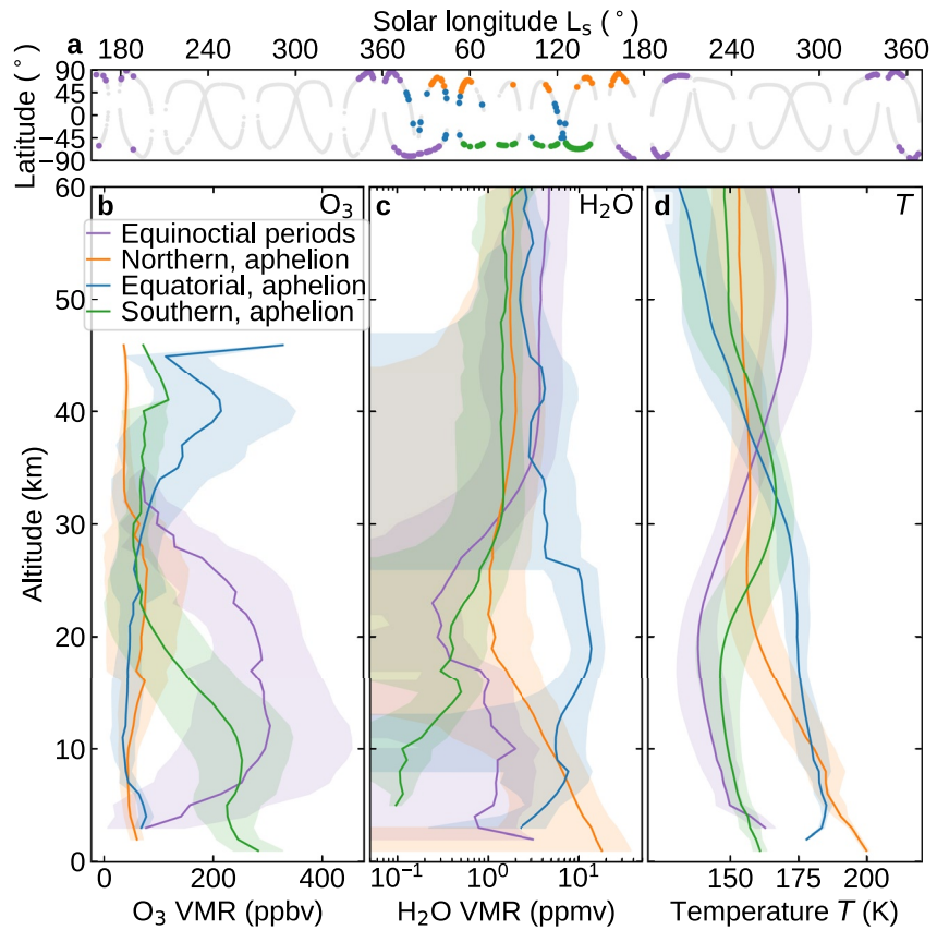
Figure 8. Mean vertical profiles of ozone and water vapor volume mixing ratios and temperature from the equinoctial periods (Figure 6), and over the aphelion period in the northern hemisphere (Figure 5), the equatorial region (Figure 7), and the southern hemisphere (Figure 4). The shaded regions indicate one standard deviation of the averaged profiles.
