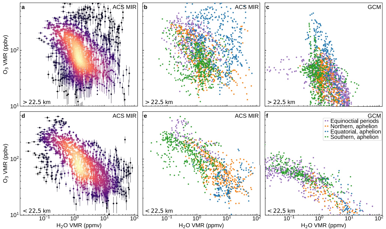
Figure 11. Correlation between water vapor and ozone. Panels a, b, d, and e show the simultaneous retrieved O_3 and H_2O data at each tangent height, where both gases were measured by ACS MIR. The upper panels show data from above 22.5 km, while the lower panels show lower altitude data. Panels a and d include measurement uncertainties and are colored using a Gaussian kernel density estimate, using the full data set (brighter means high density of data points). Panels b and e show the same data as panel a and d, but using colors to indicate the latitude and L_s groupings used in Figures 4–8. Panels c and f use vertical profiles of H_2O and O_3 volume mixing ratios extracted from the LMD global climate model for the terminator times at the latitude and L_s of the ACS MIR occultations used in the other panels (colored as in panels b and e).
