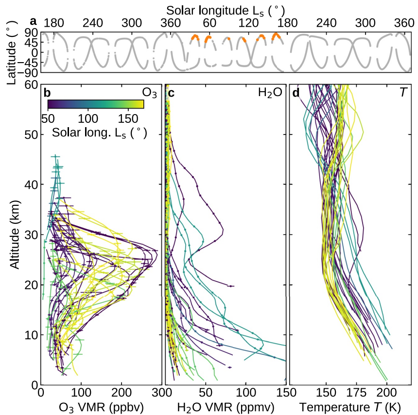
Figure 5. Aphelion ozone observations during northern late spring and summer. Panel a shows the latitude and L_s of observations, volume mixing ratio vertical profiles of ozone (panel b) and water vapor (panel c) retrieved from atmospheric chemistry suite mid-infrared (ACS) MIR, and temperature retrieved from ACS near-infrared channel (panel d). Colors indicate L_s . These profiles were measured at northern latitudes (55°N–66°N) during the aphelion period (northern summer) and correspond to Figure 2c.
