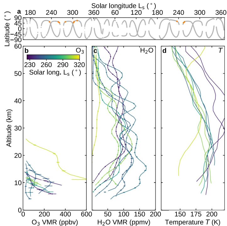
Figure 3. Perihelion ozone observations during northern fall and winter. Panel a shows the latitude and L_s of observations, retrieved volume mixing ratio vertical profiles of ozone (panel b) and water vapor (panel c) retrieved from atmospheric chemistry suite mid-infrared (ACS MIR), and temperature retrieved from ACS near-infrared channel (panel d). Colors indicate L_s . These profiles were measured at middle northern latitudes (47°N–66°N) around the perihelion period (northern winter).
