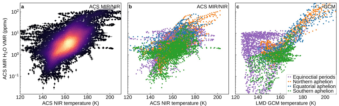
Figure 12. The correlation between water vapor and temperature. Panels a and b show the retrieved H_2O from ACS MIR and the coincident measurements of temperature made with ACS near-infrared channel (NIR). The ACS NIR data was interpolated to the pressure levels of the ACS MIR tangent heights. Panel a includes measurement uncertainties and is colored using a Gaussian kernel density estimate (brighter means high density of data points). Panel b shows the same data as panel a, but using colors to indicate the latitude and L_s groupings used in Figures 4–8. Panel c uses vertical profiles of H_2O and O_3 volume mixing ratios extracted from the LMD global climate model for the terminator times at the latitude and L_s of the ACS MIR occultations used in panels a and b (colored as in panel b).
