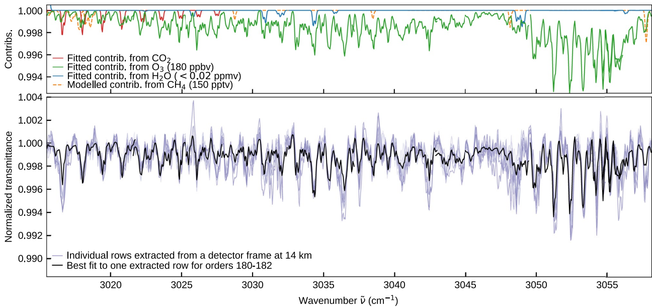
Figure 1. Example atmospheric chemistry suite mid-infrared (AIC MIR) spectra showing ozone absorption features. The top panel shows contributions to the best-fit line for different gases. The P and R branches of the 003←000 vibration rotation band of O 3 are distinct and dominate the spectral range. Water vapor lines are not present and a portion of the newly identified magnetic dipole band of CO 2 is visible at lower wavenumbers. Also indicated are the locations of CH 4 absorption lines that are targeted in this configuration of ACS MIR. The lower panel shows normalized spectra from orders 180–182 extracted from 11 rows of the ACS MIR detector images (shades of purple) and a best-fit line for one row (black). Each row corresponds to a unique tangent height, separated by ~175 m.
