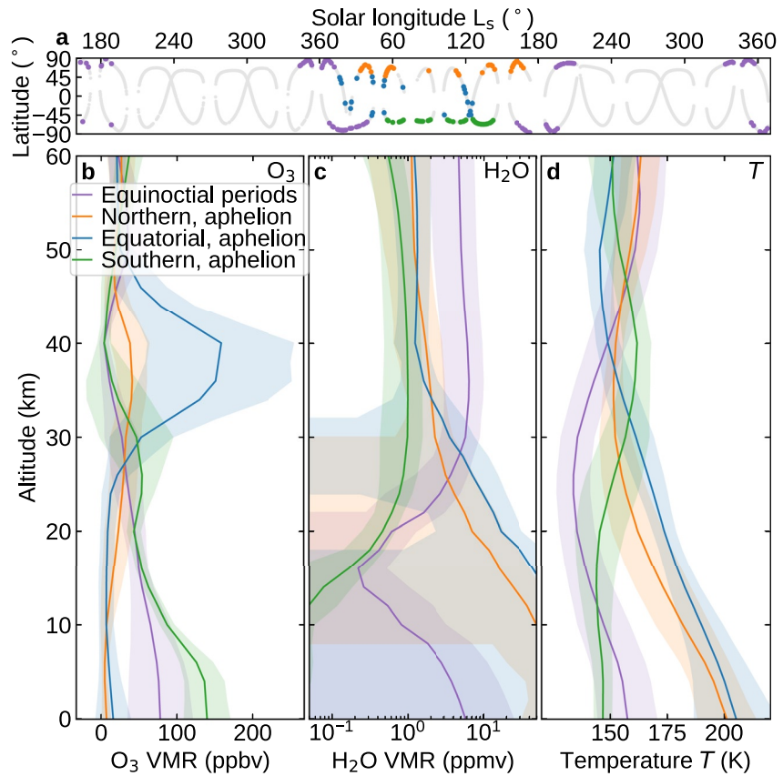
Figure 9. Mean vertical profiles extracted from the LMD global climate model (GCM). Shown are ozone volume mixing ratio (VMR) in panel b, water vapor VMR in panel c, and temperature in panel d, as in Figure 8. Each profile was modeled at the local solar terminator time and location of an ACS MIR solar occultation. Profiles are grouped into the equinoctial periods (Figure 6), and over the aphelion period in the: northern hemisphere (Figure 5), the equatorial region (Figure 7), and the southern hemisphere (Figure 4). The shaded regions indicate one standard deviation of the averaged profiles. Lefèvre et al. (2021) noted that for a given column of H_2O , the LMD GCM underestimated SPICAM O_3 column abundances by about 2 times when using the standard gas-phase chemistry. However, after the inclusion of heterogeneous uptake of OH, HO_2 and H_2O_2 on water ice aerosols was included, differences between the GCM and SPICAM were largely overcome, but these processes remain uncertain.
