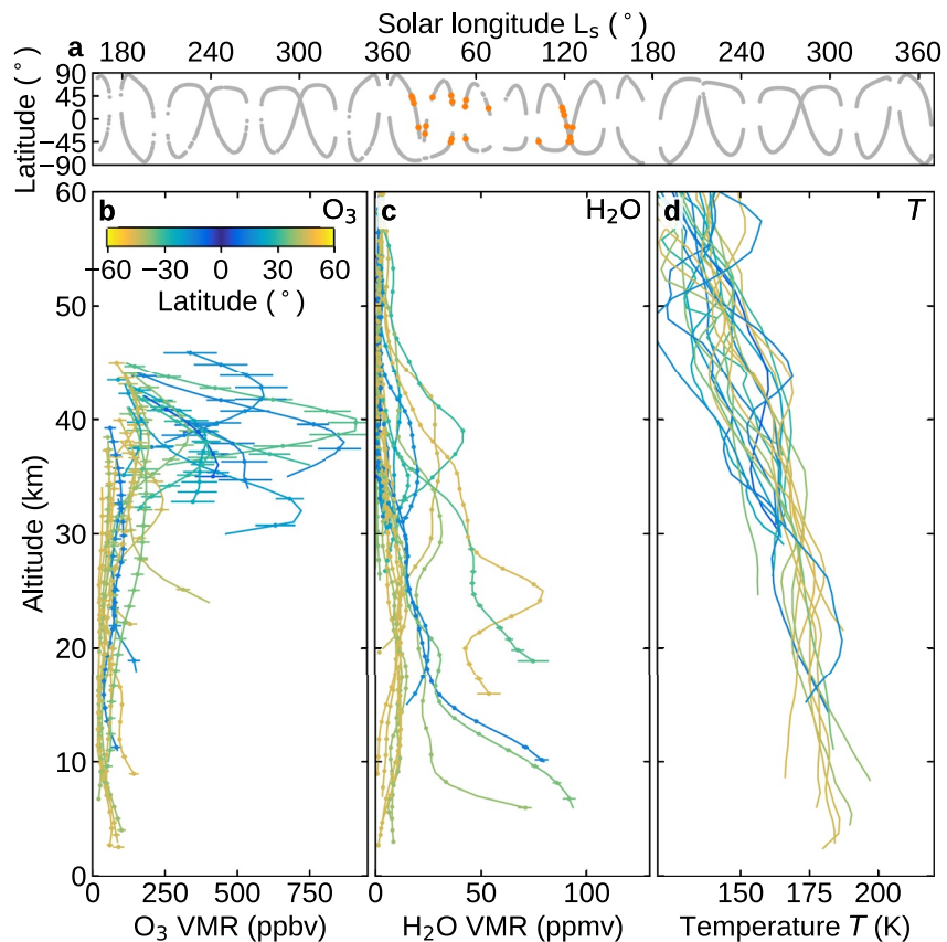
Figure 7. Ozone observations made at equatorial and low middle latitudes during the aphelion period. Panel a shows the latitude and L_s of observations, volume mixing ratio vertical profiles of ozone (panel b) and water vapor (panel c) retrieved from atmospheric chemistry suite mid-infrared (ACS MIR), and temperature retrieved from ACS near-infrared channel (panel d). Colors indicate latitude. These profiles were measured at low latitudes (40°S–40°N) during the aphelion period (southern winter/northern summer) and correspond to panels c and g of Figure 2.
