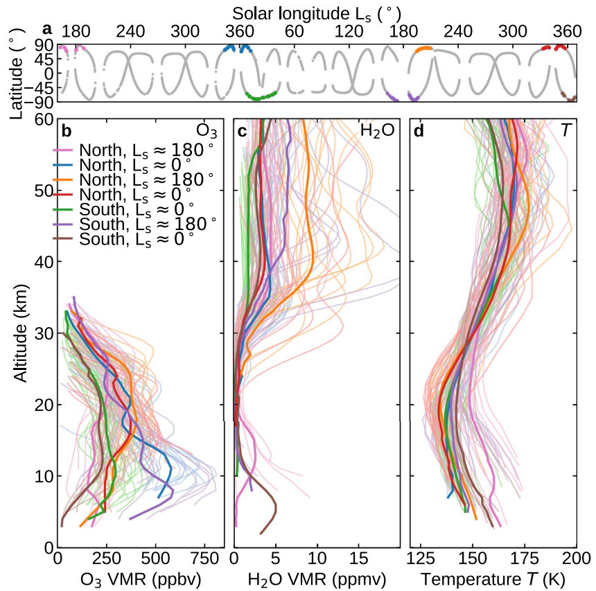
Figure 6. Ozone observations during the equinoctial periods. Panel a shows the latitude and L_s of observations, volume mixing ratio vertical profiles of ozone (panel b) and water vapor (panel c) retrieved from atmospheric chemistry suite mid-infrared (ACS MIR), and temperature retrieved from ACS near-infrared channel (panel d). Colors indicate grouping by time period and hemisphere. These profiles were measured toward the north and south poles around L_s 0^\circ and 180^\circ and correspond to panels b, d, e, f, h and i of Figure 2.
