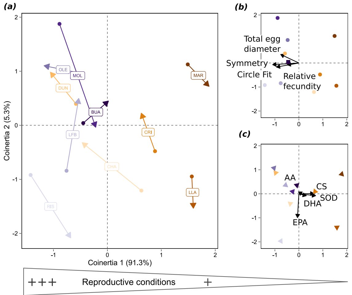
Figure 2. Graphical results of the co-inertia analysis of the reproductive and biochemical variables for winter 2018. The left-hand plot (a) (normed site-scores) shows the position of the sites on the co-inertia axes using the reproductive (origins of the arrows) and biochemical (arrowheads) co-inertia weights. The shorter the arrows, the better the match between the two projections. The right-hand pair of plots shows the contribution of the two groups of variables to the canonical space (reproductive traits (b) on the top; biochemical variables on the bottom (c)). Vectors pointing in the same direction are correlated and longer vectors contribute more to the structure. Site name abbreviations are as follows: Maryport MAR, Llanddulas LLA, Criccieth CRI, Champeaux CHA, Douarnenez, plage du Ris RIS, La Fontaine aux Bretons LFB, Oléron OLE, Moledo MOL, Buarcos BUA. Biochemical abbreviations as in Fig. 1.
