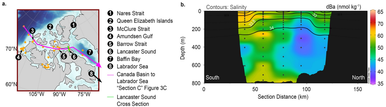
Figure 8. Dissolved Ba distributions in the Canadian Arctic Archipelago. (a) Geography of the CAA with pertinent features numbered and labeled. Sections investigated in this study are identified by purple and green lines. The purple line moves from the Canada Basin, through the Parry Channel, into Baffin Bay. (b) A cross-section of the Lancaster Sound depicting dBa on the z -axis; this cross section includes salinity contours from 32 to 34.5 at intervals of 0.5 (dBa data published in Mears et al., 2020).
