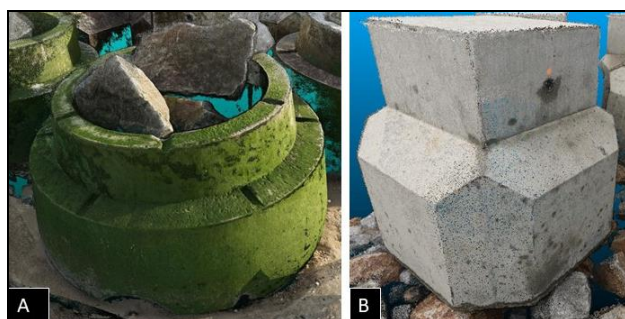
Figure 1. A: Accroberm™ II (2.24 m diameter); B: 'double cube' unit (1.3 m nominal diameter)
