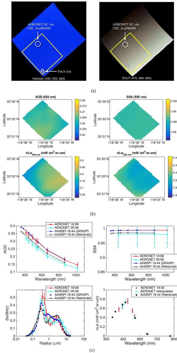
Figure 11. (a) Nadir AirMSPI intensity image from spectral combination of 445, 555, and 660 nm bands (left image) and DoLP image from spectral combination of 470, 660, and 865 nm bands (right image). The bright spot inside the white circle marked on the intensity image (dark spot inside the white circle marked on the DoLP image) is the AERONET USC_SeaPRISM ocean color station, located on the Eureka oil platform. AirMSPI observations were acquired at 19:44 UTC on 6 February 2013. The yellow frame bounds the area viewed in common from all nine angles (observations over this area are used for retrieval). (b) Maps of retrieved AOD at 555 nm (top left), SSA at 555 nm (top right), nLw at 445 nm (bottom left), and nLw at 555 nm (bottom right). (c) Comparisons of retrieved spectral AOD (top left), SSA (top right), aerosol size distribution (bottom left), and nLw (bottom right) using the GRASP and JPL algorithms to AERONET reported values.
