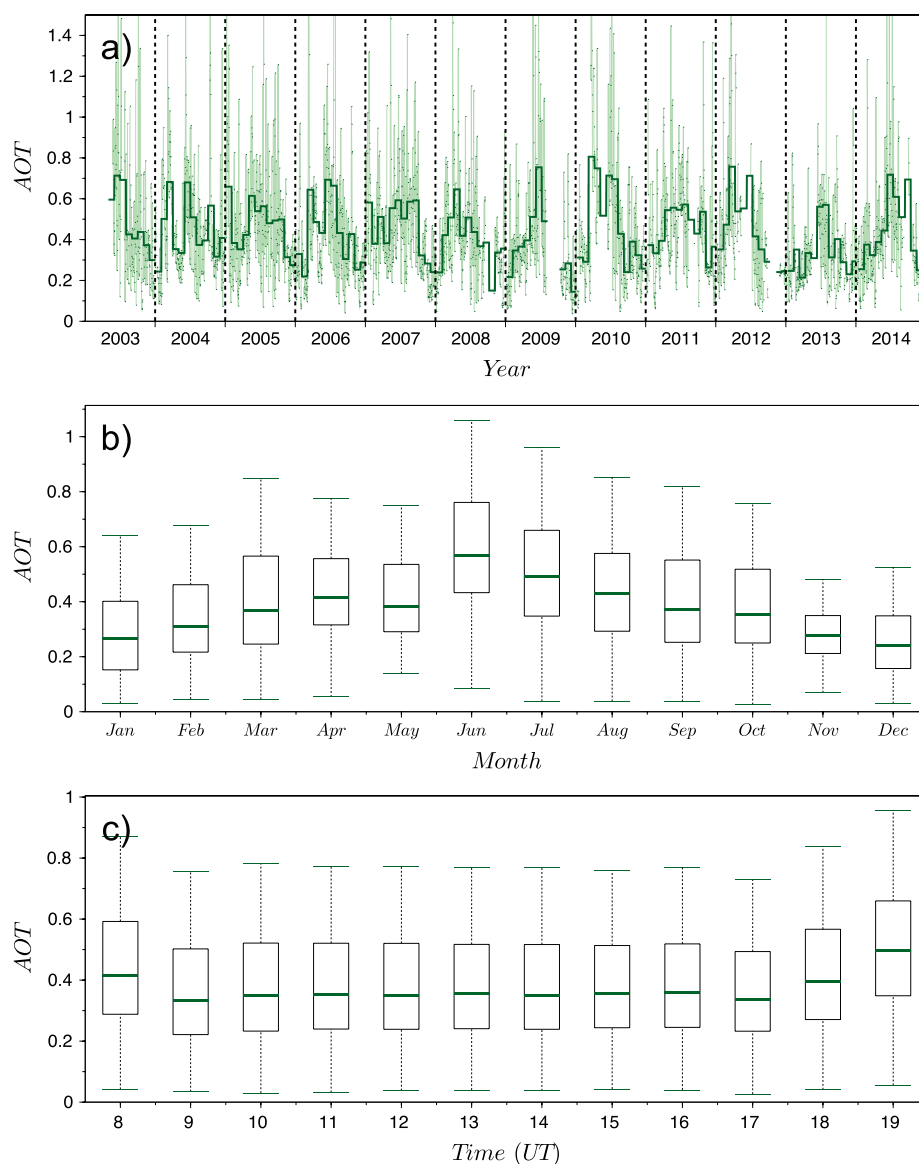
Figure 2. Aerosol optical thickness measured at Mbaur and interpolated at 532 nm. (a) The time series shows daily averages (light green) and monthly averages (dark green) of the parameter. (b and c) Boxplots for different time scales. The boxes extend from the first to the third quartile (IQR). The colored line is the median. Whiskers, highlighting variability, extend from minimal and maximal values include in (median-1.5 IQR; median + 1.5 IQR).
