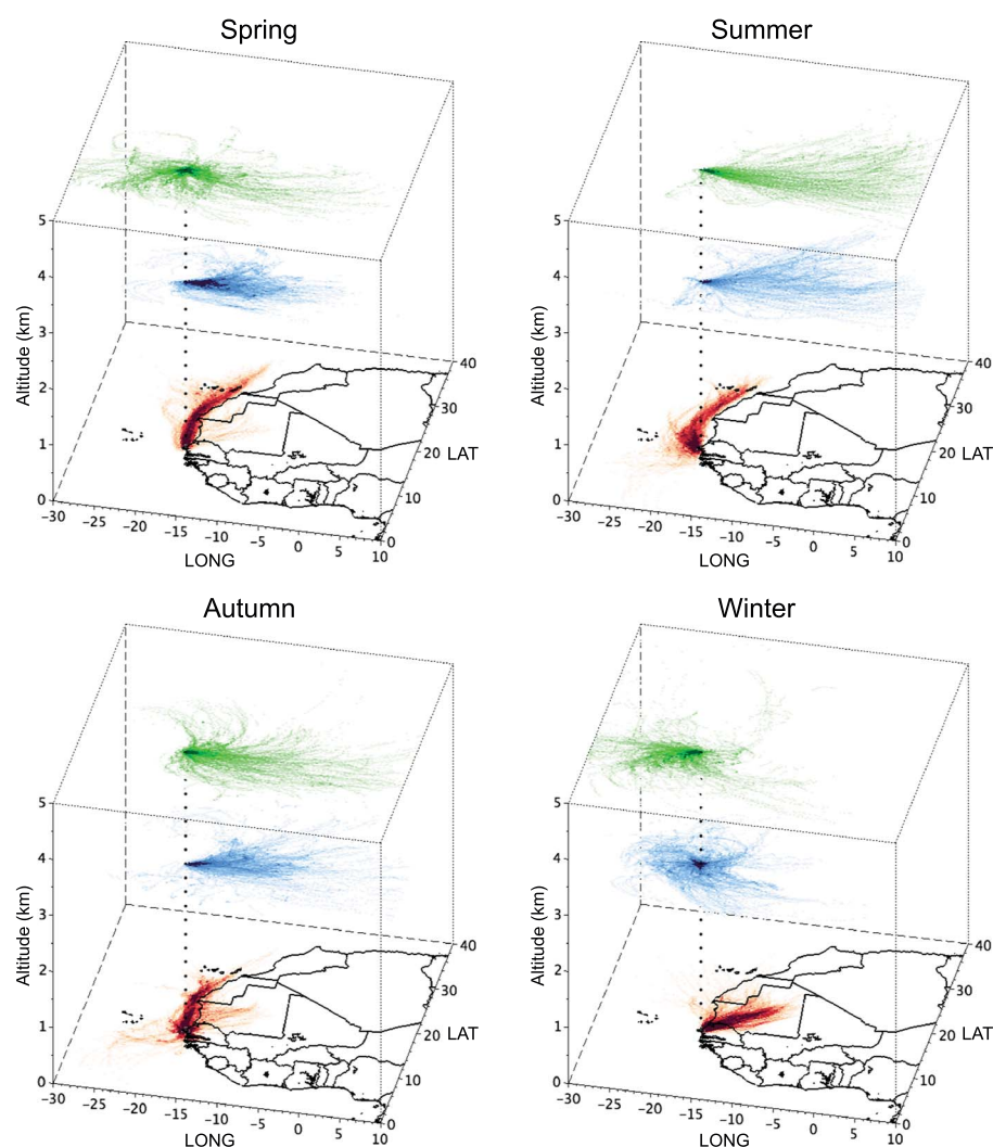
Figure 1. Seasonally averaged back trajectories processed over 72 h and finishing at Mbour at ground level (red), 3000 m (blue), and 5000 m (green) for 2006. The color intensity is proportional to the number of back trajectories contained by pixel. The black dotted line follows the vertical of the observation site.
