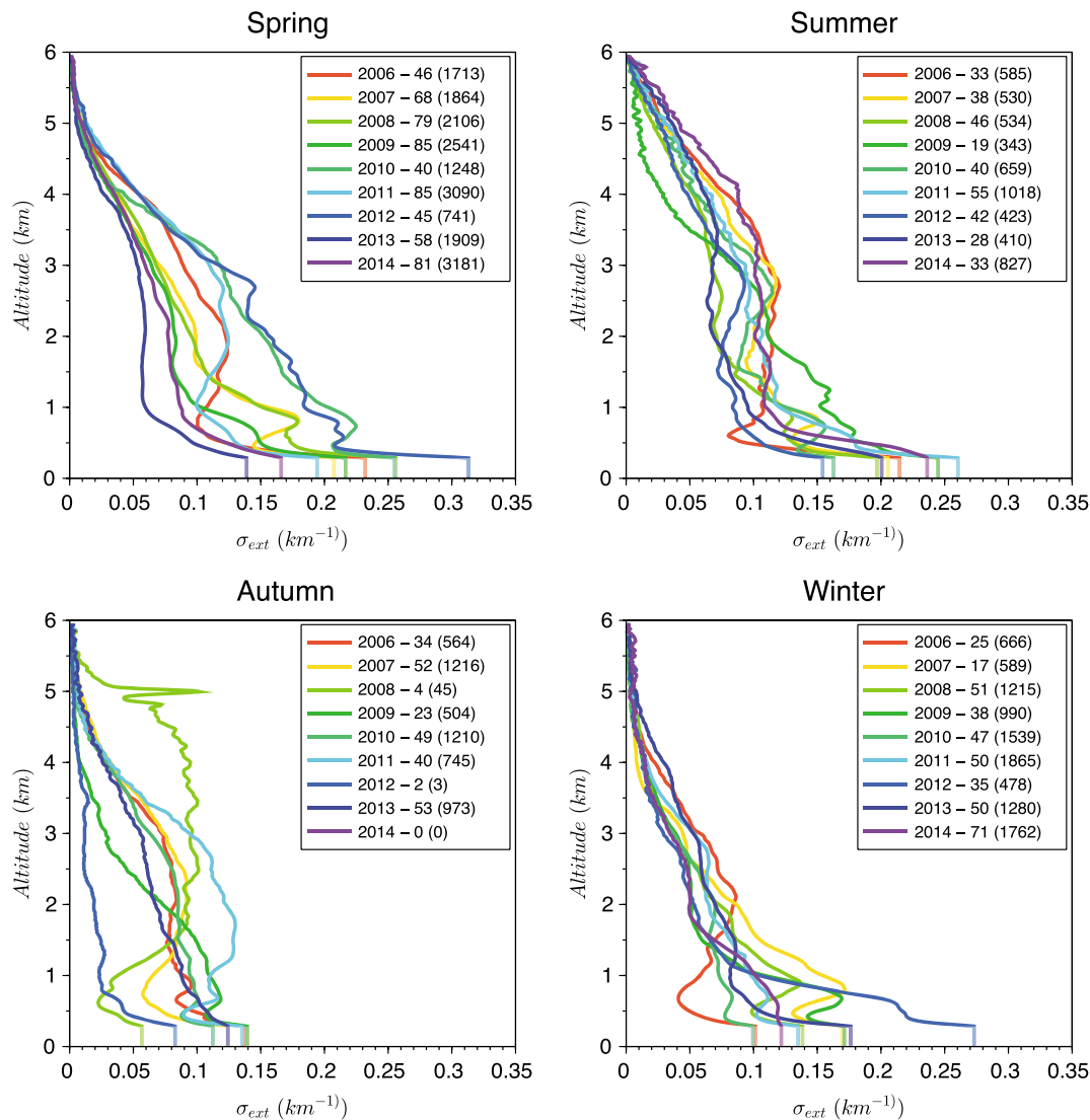
Figure 7. Seasonally averaged extinction profiles for different years. Beside each year, the numbers of different days available and, in parentheses, the total number of inversions for this period.
