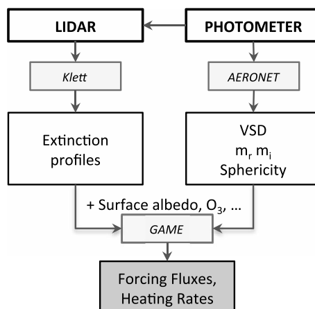
Figure 8. Aerosol radiative effect calculation logistics.
