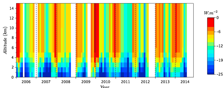
Figure 9. Monthly averages vertical profiles of direct aerosol net radiative effect between 2006 and 2014.
