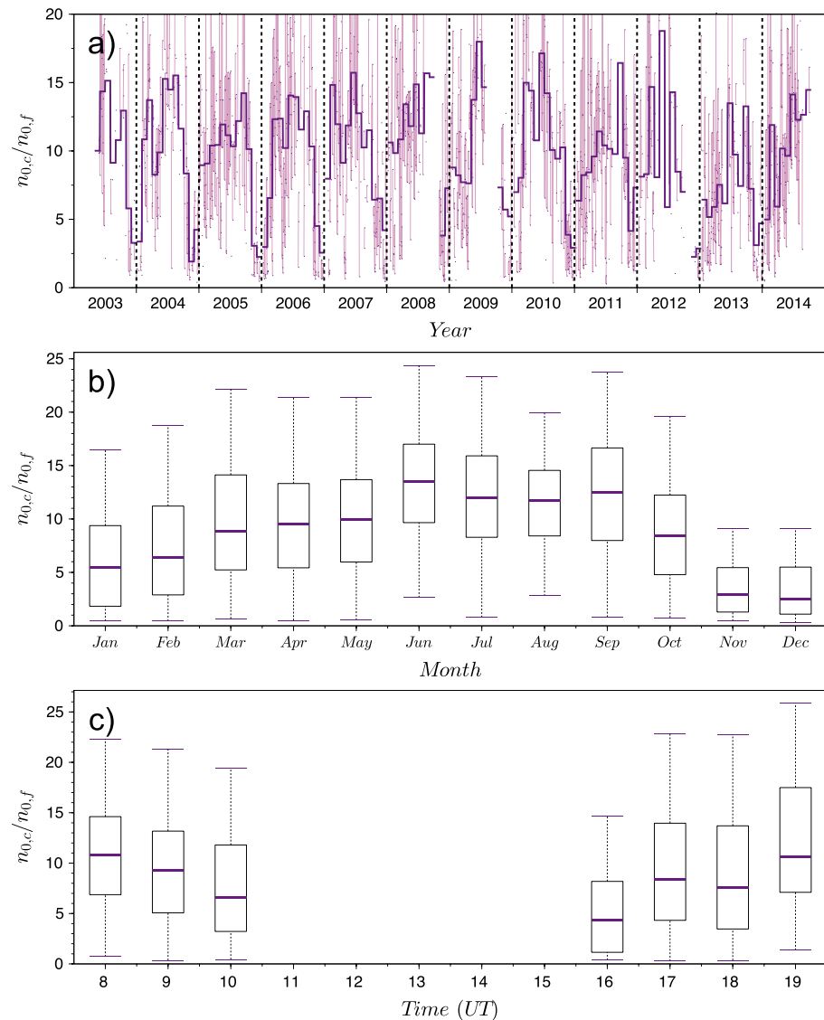
Figure 4. Same as Figure 2 but for the ratio of coarse and fine modes amplitude.
