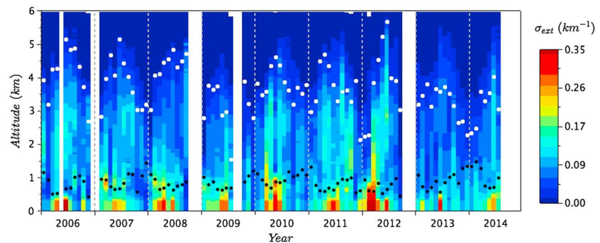
Figure 6. Time series of monthly averaged extinction profiles. The white and black dots refer, respectively, to the heights of the planetary boundary layer and the top layer.
