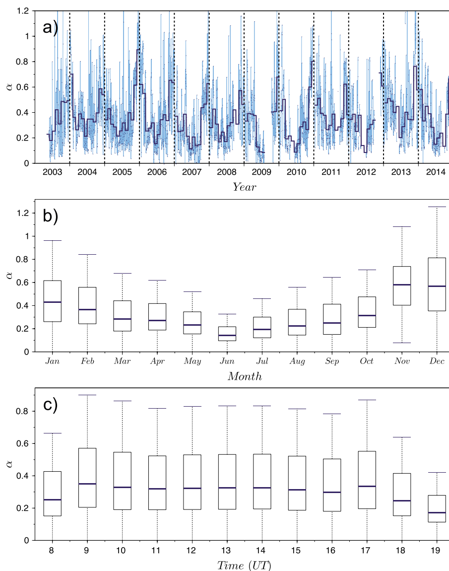
Figure 3. Same as Figure 2 but for Angstrom exponent.
