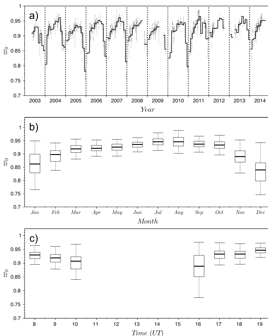
Figure 5. Same as Figure 2 but for the single-scattering albedo \omega_0 .
