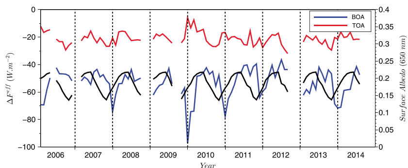
Figure 10. Solar clear-sky radiative effect efficiency at the top (in red) and the bottom (in blue) of the atmosphere. The black solid line is the surface albedo at 650 nm.
