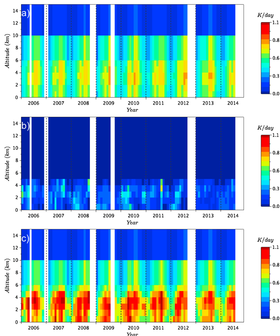
Figure 11. Solar clear-sky heating rates profiles (monthly averages) from 2006 to 2014 for the different atmospheric contributions: (a) gases, (b) aerosols, and (c) total.
