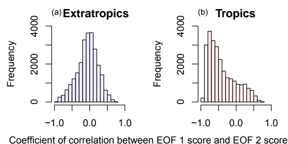
Figure 17. Histograms of the coefficient of correlation between EOF 1 and EOF 2 scores. Out of 79 192 total inferred pixels, 49 902 pixels are selected by the condition \text{SD}(\text{EOF 1 Score}) < 0.02 , \text{SD}(\text{EOF 2 Score}) < 0.02 . The results in Figs. 12–14 are based on the data within the center six bins in these histograms.
