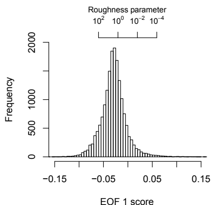
Figure 12. The distribution of EOF 1 scores obtained from cold ice clouds over extratropical oceans during September 2005. The median of the EOF 1 score is -0.0293 , corresponding to a roughness parameter of 2.82. Consistent with previous studies, roughened particles better simulate the measured polarized reflectivity.
