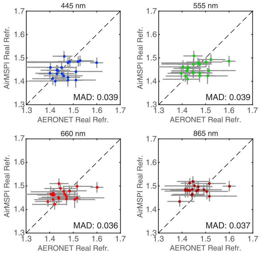
Figure 6. Same as Figure 5 but for the real part of the aerosol refractive index.
