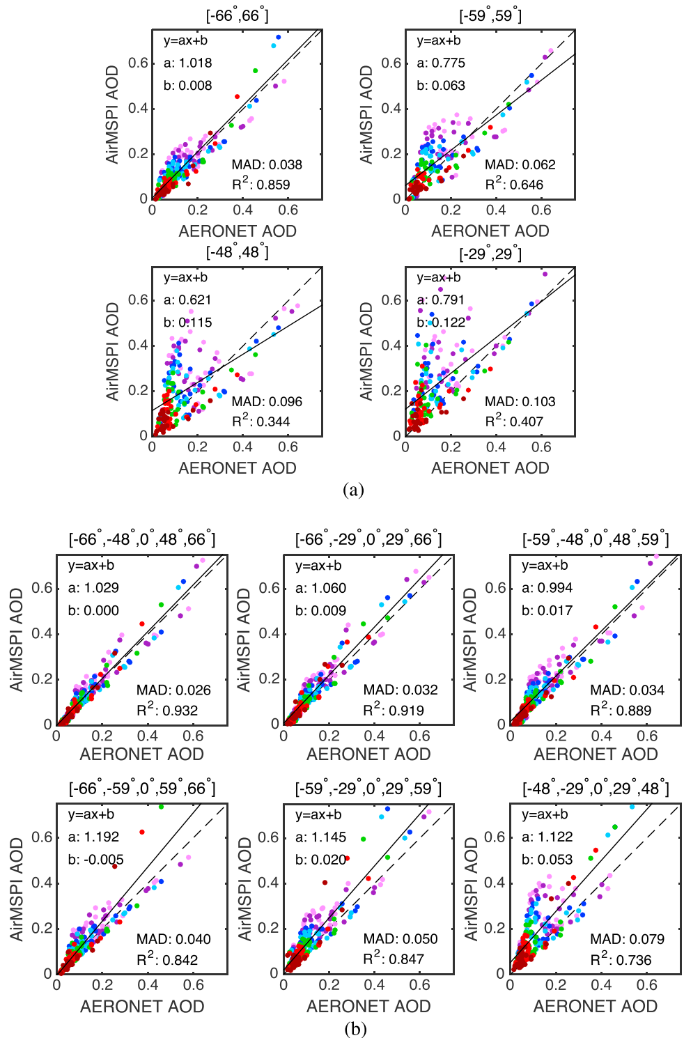
Figure 9. Regression of AirMSPI retrieved AOD against AERONET measured values using different combinations of (a) two-viewing angle and (b) five-viewing angle retrievals. The results for seven AirMSPI spectral bands are plotted in different colors: pink (355 nm), purple (380 nm), dark blue (445 nm), light blue (470 nm), green (555 nm), red (660 nm), and brown (865 nm). As indicated in the subtitle, the results from two-angle combinations ( -66^\circ, +66^\circ ), ( -59^\circ, +59^\circ ), ( -48^\circ, +48^\circ ), and ( -30^\circ, +30^\circ ) are plotted in Figure 9a (top left), Figure 9a (top right), Figure 9a (bottom left), and Figure 9a (bottom right), respectively. The results from five-angle combinations ( 0^\circ, \pm 48^\circ, \pm 66^\circ ), ( 0^\circ, \pm 29^\circ, \pm 66^\circ ), ( 0^\circ, \pm 48^\circ, \pm 59^\circ ), ( 0^\circ, \pm 59^\circ, \pm 66^\circ ), ( 0^\circ, \pm 29^\circ, \pm 59^\circ ), and ( 0^\circ, \pm 29^\circ, \pm 48^\circ ) are plotted in Figure 9b (top left), Figure 9b (top middle), Figure 9b (top right), Figure 9b (bottom left), Figure 9b (bottom middle), and Figure 9b (bottom right), respectively.
