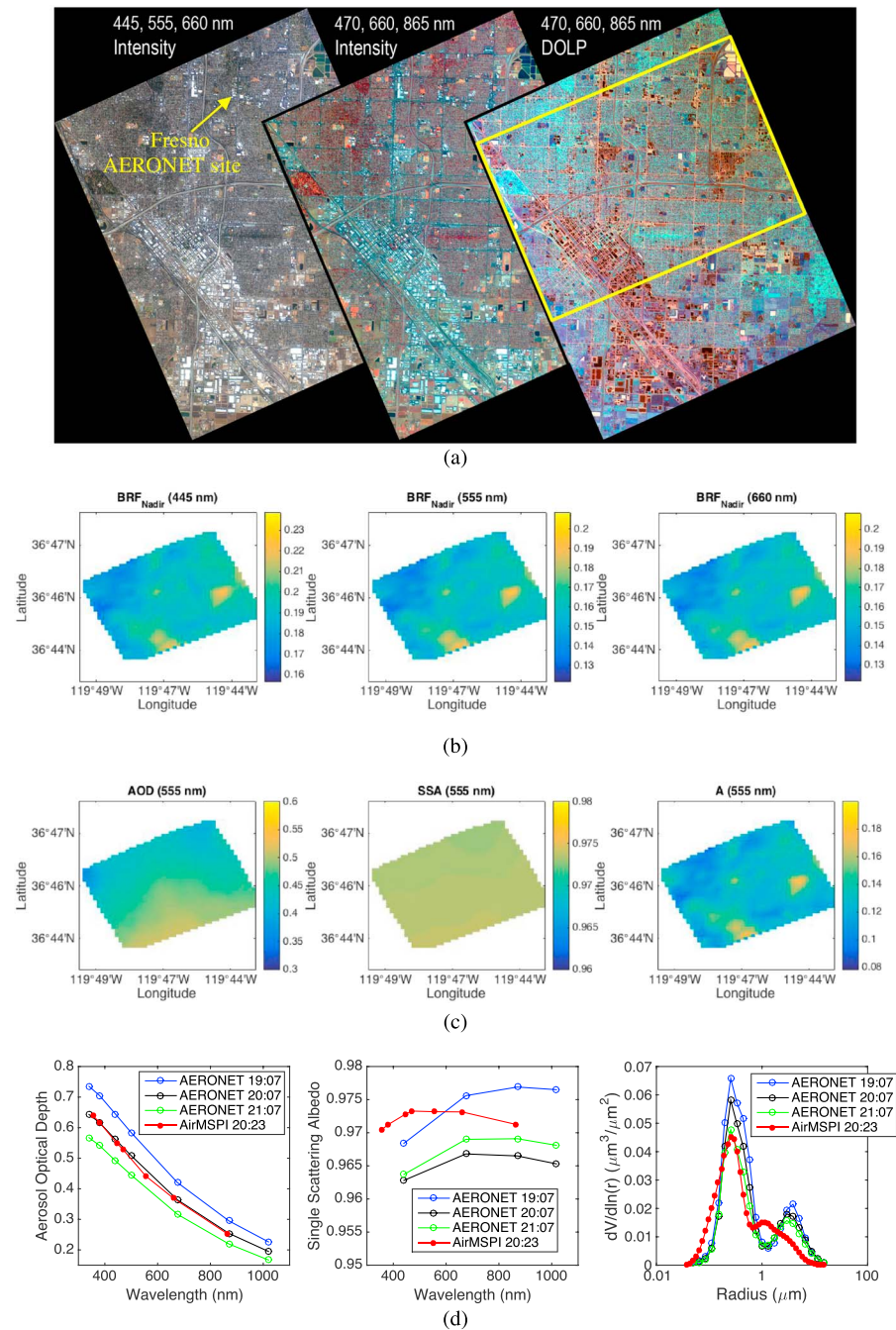
Figure 3. (a) High-resolution (10 m) AirMSPI nadir imagery of Fresno, CA, acquired on 6 January 2012 [Diner et al., 2013]. The left and middle images are radiance data using different spectral band combinations. The location of the Fresno AERONET site is marked in the left image. The right image displays DOLP in the three polarimetric bands, and the yellow box indicates the area viewed at all nine AirMSPI view angles and where data are collected for retrieval. (b) Lower resolution imagery (~0.5 km) of the retrieval area after pixel aggregation. The left, middle, and right panels give the images of bidirectional reflectance factor (BRF) at blue (445 nm), green (555 nm), and red (660 nm) bands, respectively. BRF is defined as \pi I_{\text{meas}} d^2 / \mu_0 E_0 , where I_{\text{meas}} is the measured radiance, d is the Earth-Sun distance, \mu_0 is the cosine of solar zenith angle, and E_0 is the exo-atmospheric solar irradiance. (c) Retrieved AOD, SSA, and surface albedo (A) maps at 555 nm in the left, middle, and right panels, respectively, with patch resolution 0.5 km. (d) AirMSPI retrieved AOD, SSA, and volume-weighted aerosol size distribution at the patch closest to the Fresno AERONET site, compared to the AERONET-derived values.
