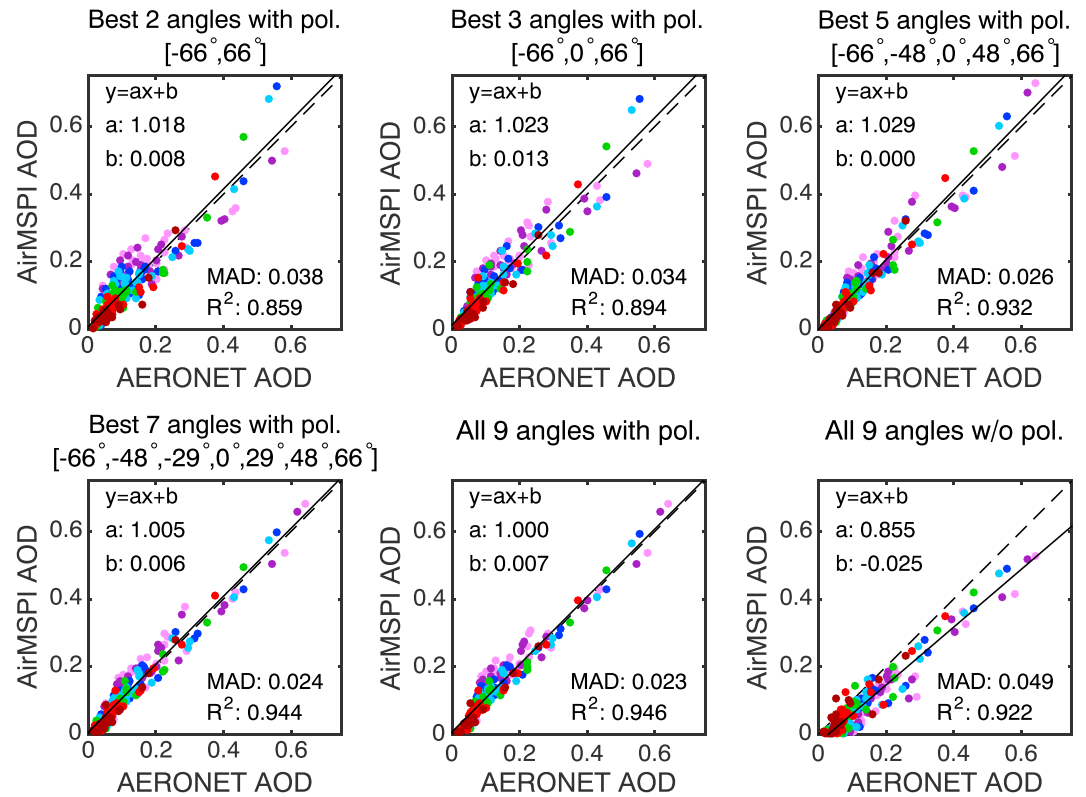
Figure 10. Regression of AirMSPI retrieved AOD against AERONET measured values using different numbers of view angles. For a given number of viewing angles, only the results from the best angular set indicated in a panel title are demonstrated. As described in Figure 9, different colors are assigned to the results for seven AirMSPI spectral bands. The retrievals use observations from (top left) two angles, (top middle) three angles, (top right) five angles, (bottom left) seven angles, and (bottom middle) nine angles, with polarization data at 470, 660, and 865 nm included in the retrievals. The nine-angle-based retrieval without polarization (indicated as “w/o pol.” in the title) is shown in Figure 10 (bottom right).
