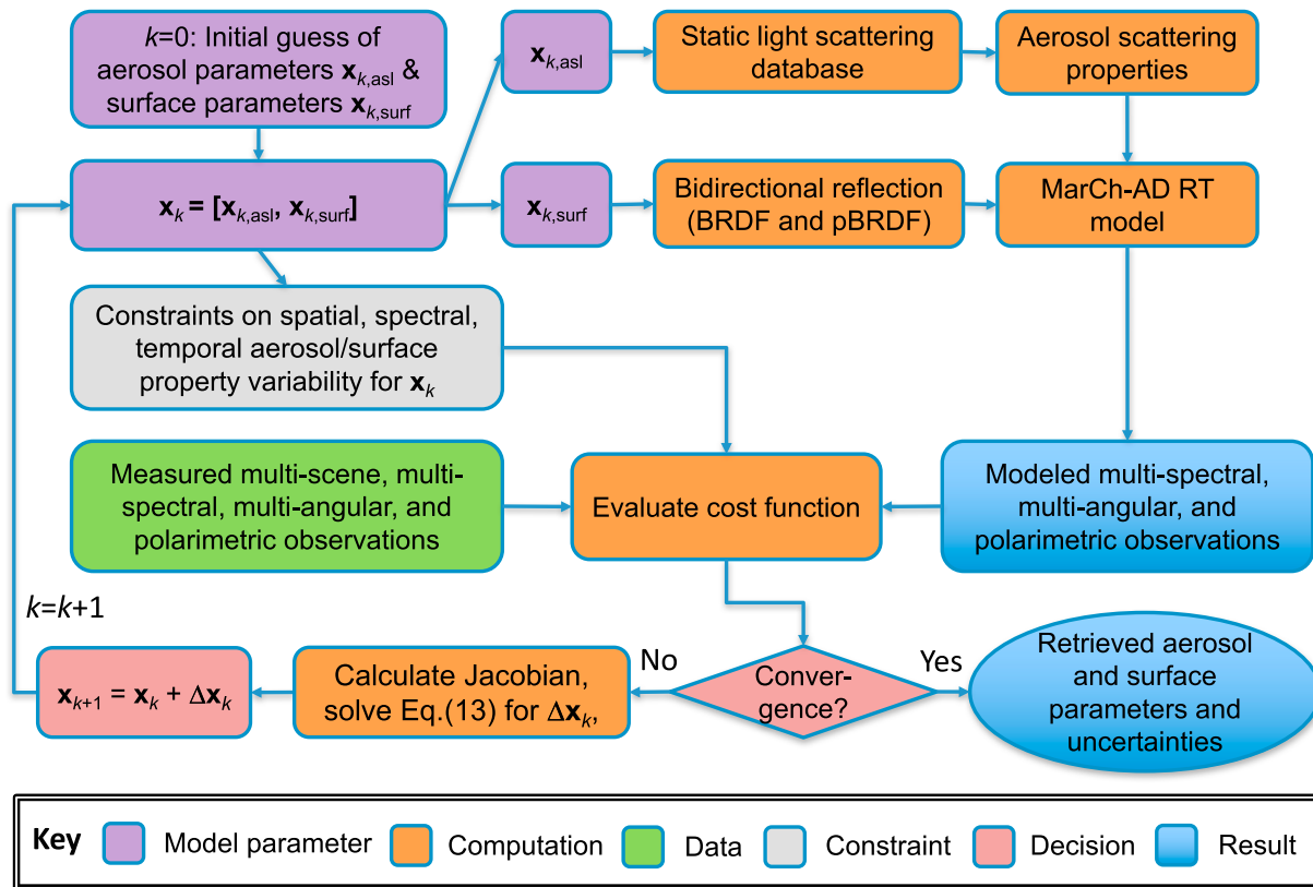
Figure 1. Algorithm flowchart for coupled retrieval of aerosol land surface reflection properties.
