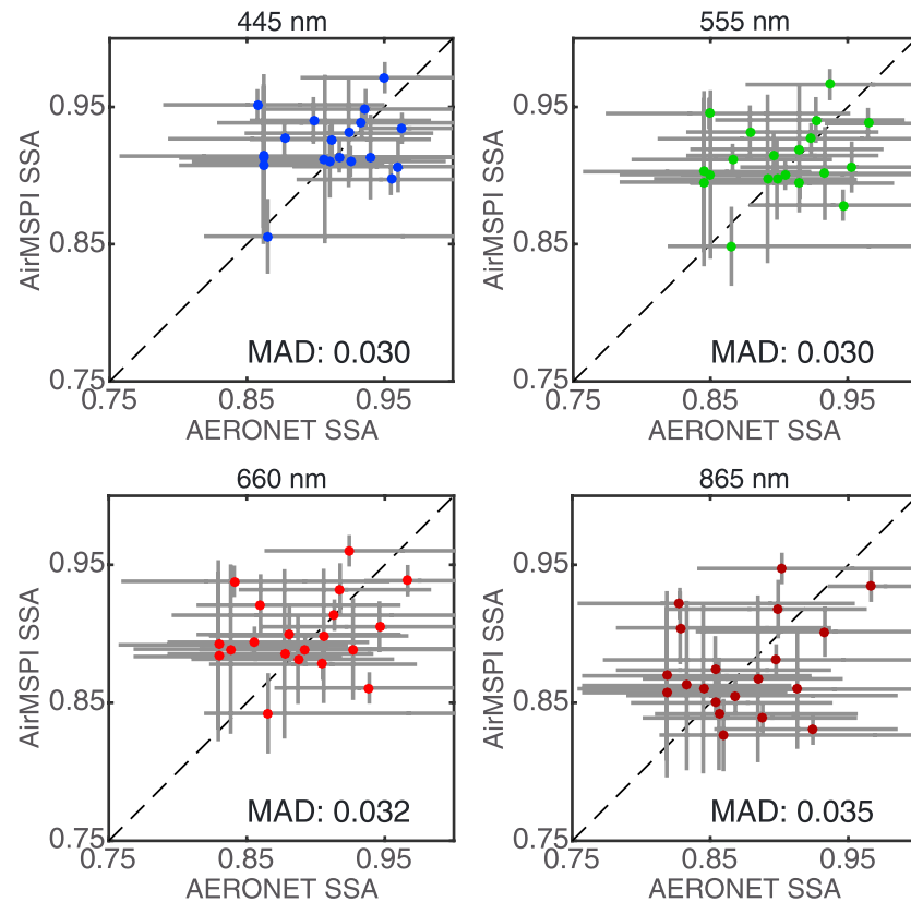
Figure 5. Regression of AirMSPI retrieved single-scattering albedo (SSA) against AERONET reference data: the SSA for (top left) 445 and (top right) 555 nm, and the SSA for (bottom left) 660 and (bottom right) 865 nm. Linear interpolation is used to obtain AERONET SSA values at the AirMSPI wavelengths. The AERONET retrieval uncertainties are adopted from Dubovik et al. [2000]. The AirMSPI errors are computed from statistics obtained over the whole image plus the errors evaluated using the method in section 4.2.
