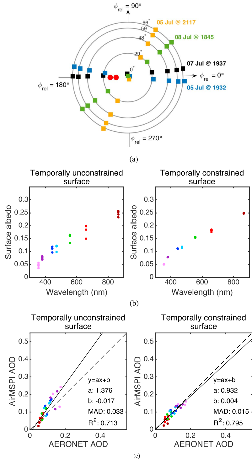
Figure 12. (a) Sun and viewing geometries of four AirMSPI visits over the Bakersfield AERONET site during 5–8 July 2016. For simplicity, the geometries for one image patch are illustrated here. The red dots indicate the solar zenith angle, \theta_0 , which had values of 13.9°, 14.0°, 21.0°, and 20.9°. The viewing geometries corresponding to the relative azimuthal angles \phi_{rel} = \phi_v - \phi_0 for the four overpasses of about 5°, 170°, 60°, and 40° are marked in black, blue, dark yellow, and green, respectively. (b) Retrieved surface albedo of the single patch from the four overpasses (left) without and (right) with imposition of temporal smoothness constraints on variations of surface reflection. Colors are the same as those specified in Figure 9. Nine-angle polarimetric observations of the pixels revisited during all four overpasses are used for retrieval. (c) Comparison of retrieved AOD from the four overpasses (left) without and (right) with temporal smoothness constraints on variations of surface reflection.
