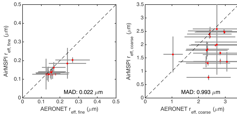
Figure 8. Same as Figure 5 but for the effective radii of fine and coarse mode aerosols.
