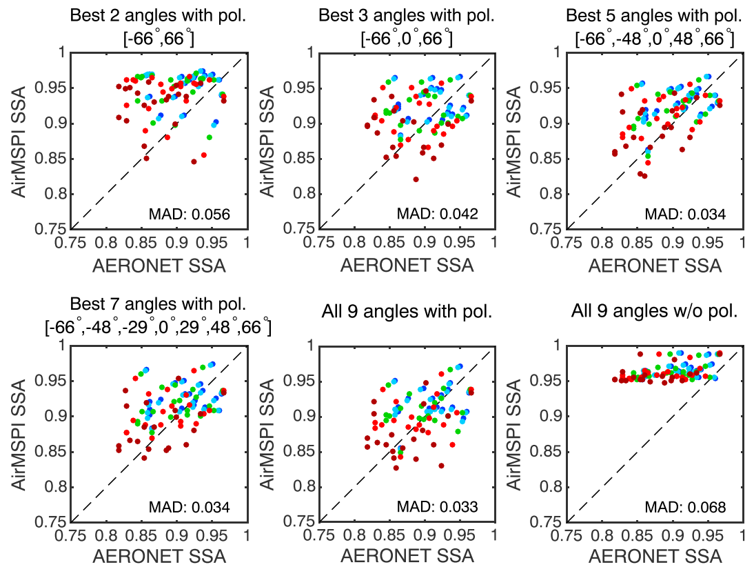
Figure 11. Regression of AirMSPI retrieved SSA against AERONET values using different number of viewing angles. Colors are the same as those in Figure 9, and retrieval conditions are the same as those in Figure 10. In the title of Figure 11 (bottom right), “w/o pol.” means “without polarization.”
