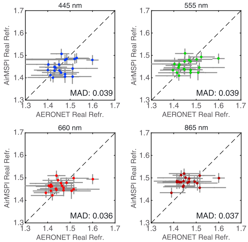
Figure 6. Same as Figure 5 but for the real part of the aerosol refractive index.
