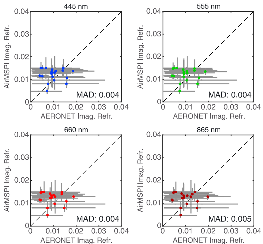
Figure 7. Same as Figure 5 but for the imaginary part of aerosol refractive index.
