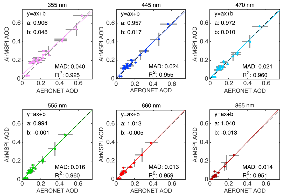
Figure 4. Regression of AirMSPI retrieved aerosol optical depth (AOD) against AERONET measured values: (top row) 355, 445, and 470 nm; (bottom row) 555, 660, and 865 nm. Linear interpolation is used to obtain AERONET AOD values at the AirMSPI wavelengths. The AERONET uncertainties are from the \pm 1 h window around the time of AirMSPI overflight plus measurement uncertainties (0.01), while the AirMSPI uncertainties are the root-mean-square of the pixel-resolved errors over the whole image. Linear regression analysis yields values of slope “a,” intercept “b,” coefficient of determination “R 2 ,” and mean absolute difference (MAD) as indicated in all panels.
