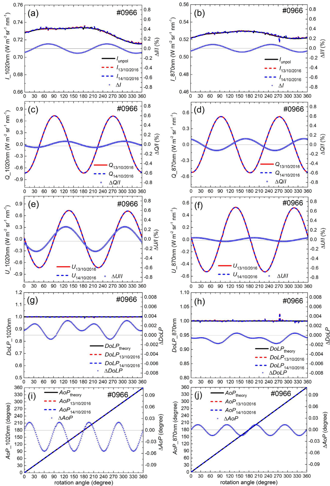
Fig. 5. Comparisons of I (a,b), Q (c,d), U (e,f), DoLP (g,h) and AoP (i,j) for the CE318-DP #0966 calculated with the coefficients measured on 13 and 14 October 2016.
