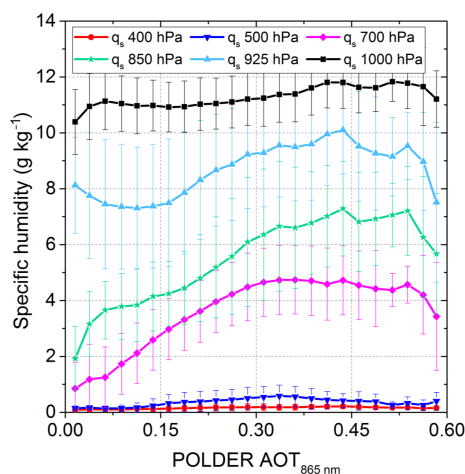
Figure 7. Mean specific humidity as a function of POLDER \text{AOT}_{865\text{ nm}} retrieved at different pressure levels, within the selected region over June–August 2008. The vertical bars represent the standard deviation for the specific humidity.
