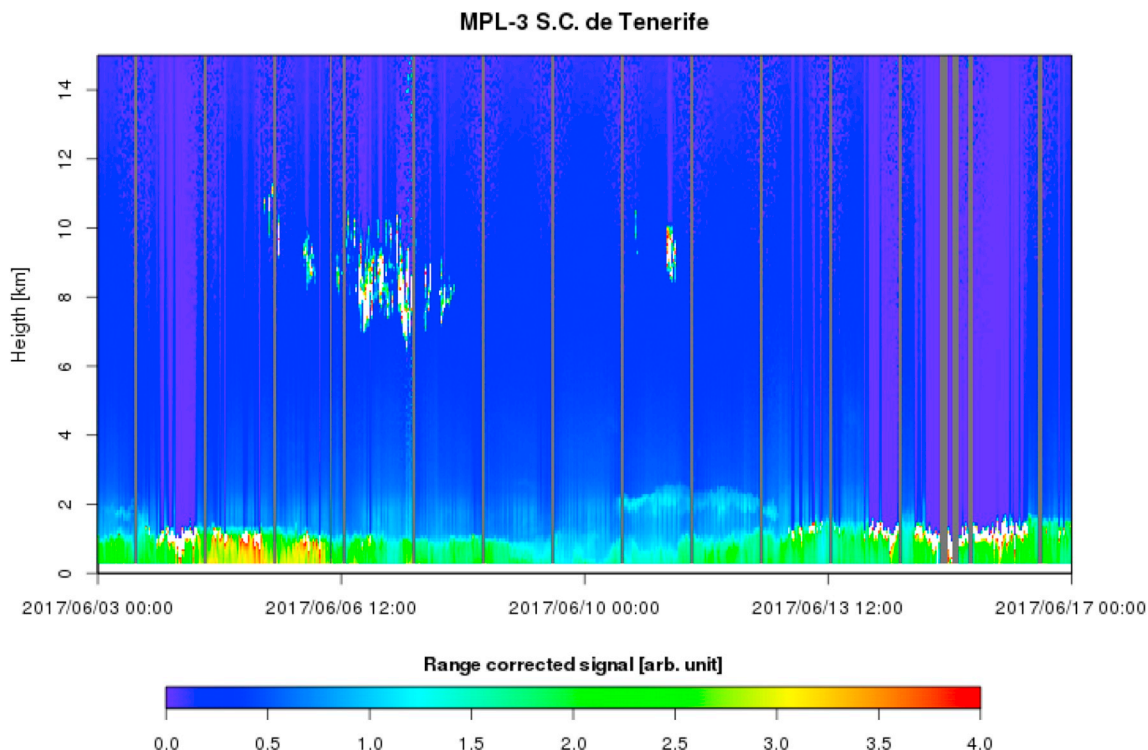
Fig. 2. Micro-Pulse Lidar (MPL-3) range corrected signals at 523 nm obtained at Santa Cruz de Tenerife station (60 m a.s.l.). Grey vertical lines represent the absence of measurements due to rain or direct solar incidence in the detector at noon.
