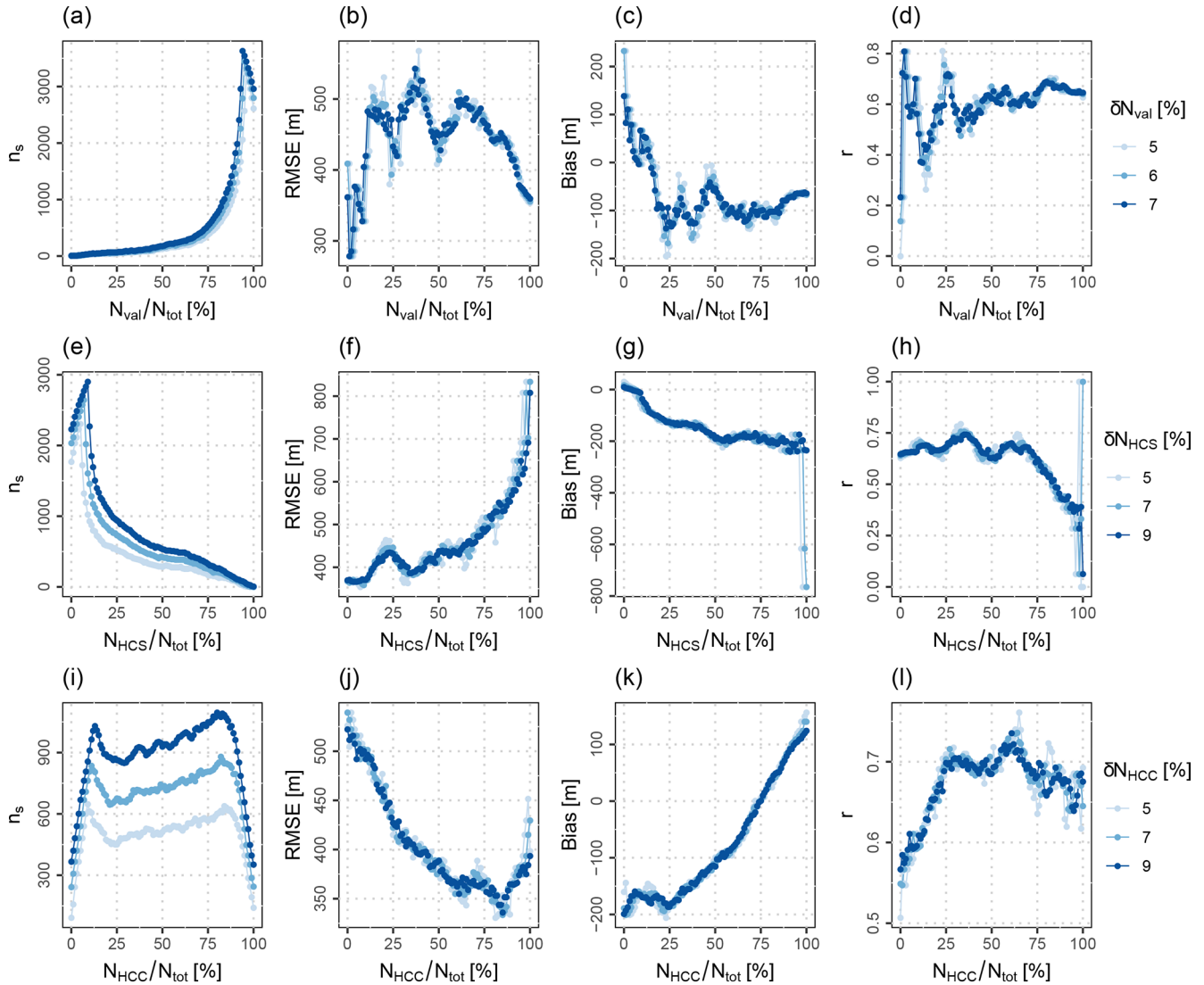
Figure 8. From left to right: number of samples n_s , RMSE, bias and correlation coefficient r for the comparison of MISBase and ceilometer retrievals as a function of the number of valid z retrievals N_{\text{val}} (panels a–d), the number of retrievals marked as high confidence surface N_{\text{HCS}} (panels e–h) and the number of retrievals marked as high confidence cloud N_{\text{HCC}} (panels i–l). Each data point is calculated for a subsample which includes only N_{\text{val}} \pm \delta N_{\text{val}} , N_{\text{HCS}} \pm \delta N_{\text{HCS}} and N_{\text{HCC}} \pm \delta N_{\text{HCC}} , respectively. The various widths of the considered N_{\text{val}} and N_{\text{HCC}} windows are indicated by the blue shading. All values are normalized by the total number of pixels within the MISBase cell N_{\text{tot}} . Data are for the year 2008 with R_c = 10 km, P = 15 and N = 10 .
