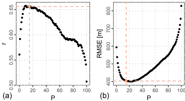
Figure 6. Evaluation of the percentile P which is applied to retrieve z_{\text{base}} from the distribution of z for the year 2008, with N = 10 and R_c = 10\text{ km} . (a) The linear correlation coefficient r between z_{\text{base}} and \hat{z}_{\text{base}} . (b) The RMSE between z_{\text{base}} and \hat{z}_{\text{base}} . The chosen value for P is highlighted in orange.
