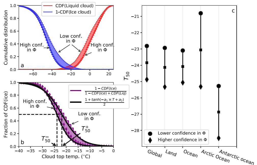
Figure 2. (a) Cumulative distribution function (CDF) of liquid cloud top temperatures (CDF(liquid)) in red and 1-CDF(ice) in blue for two degrees of confidence in the phase index ( \Phi ). (b) Fraction of CDF(ice) defined as \frac{1 - CDF(ice)}{1 - CDF(ice) + CDF(liq)} considering two levels of confidence in \Phi (purple) and the hyperbolic tangential fit retrieved from the fraction of CDF(ice) and T_{50} is retrieved from Equation (2). (c) T_{50} is retrieved considering all the pixels, for different bins of latitude, and surface type. The diamonds consider a higher confidence in the phase retrieval than the dots. The squares show the average between T_{50} retrieved considering the high and low level of confidence in the phase detection for each regime considered.
