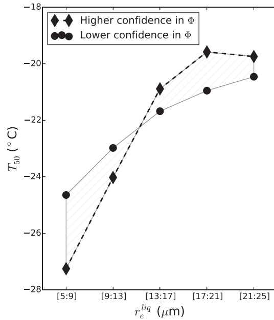
Figure 3. Glaciation temperature T_{50} from Equation (2) for different cloud droplet effective radius bins considering global data. The diamonds on the dashed line consider a higher confidence in the phase retrieval—phase index ( \Phi ) less than 20 for liquid cloud detection and \Phi greater than 180 for ice cloud detection—than the dots on the solid line— \Phi less than 60 for liquid cloud detection and \Phi greater than 140 for ice cloud detection. The results from the dashed lines are supported by fewer data points, but the phase determination is more robust than the results shown by the solid line. The area between the solid and the dashed lines represents an estimate of the uncertainty introduced by the phase decision itself.
