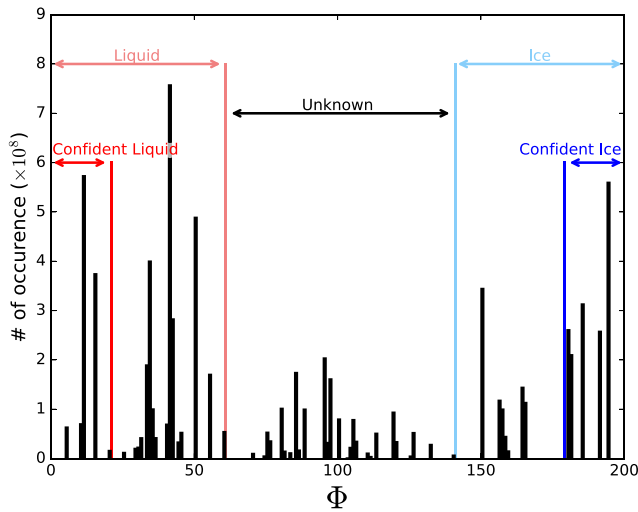
Figure 1. Cloud top phase ( \Phi ) distribution from the algorithm developed by Riedi et al. (2010). The vertical bars for confident liquid, liquid, ice, and confident ice are respectively at \Phi equal to 20, 60, 140, and 180.
