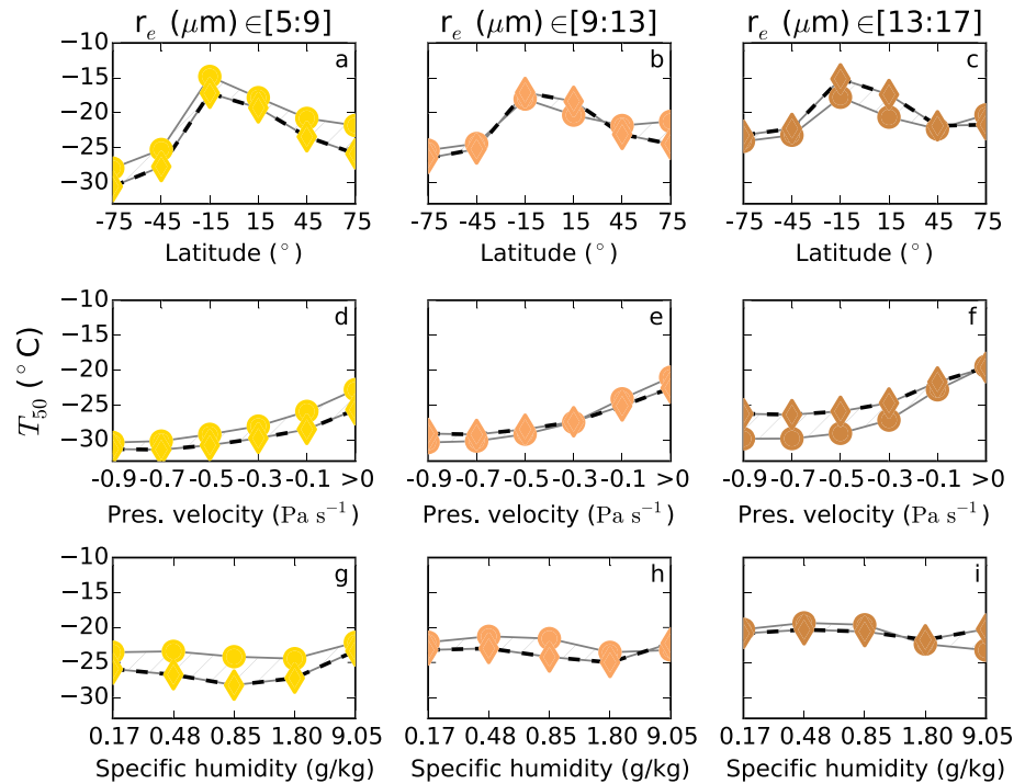
Figure 4. Glaciation temperature T_{50} from Equation (2) for different bins of cloud droplet effective radius, and (a, b, c) latitude, (d, e, f) large-scale pressure velocity, and (g, h, i) specific humidity. Global data are considered for the bins of large-scale pressure velocity and specific humidity. The diamonds on the dashed line consider a higher confidence in the phase retrieval—phase index ( \Phi ) less than 20 for liquid cloud detection and \Phi greater than 180 for ice cloud detection—than the dots on the solid line— \Phi less than 60 for liquid cloud detection and \Phi greater than 140 for ice cloud detection. The hatched area represents the uncertainty.
